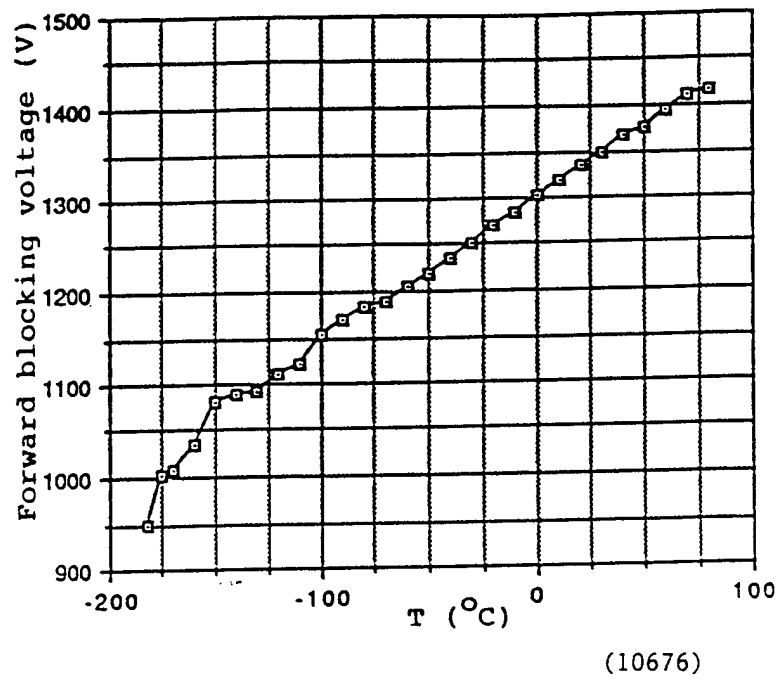
Figure 2. Measured blocking voltage versus temperature.
