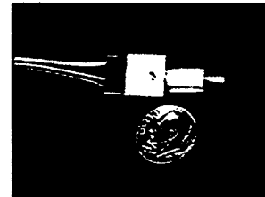
■ ERG's fiber-optic light-emitting diode, pictured above, can measure the vibration of a free-standing structure or of a structure in which it is embedded.
