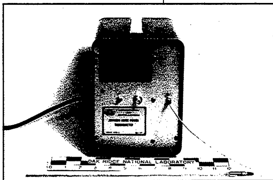
■ Pictured above is an industrial prototype of the JNT. In a demonstration at a fossil-fuel utility plant, this device monitored furnace temperature.
