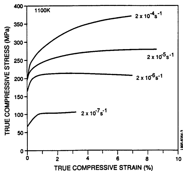
Figure 23. True compressive stress-strain diagrams for the forged Al 66 Ti 25 Mng + 5 vol.% TiB 2 material at various strain rates at (a) 900K, (b) 1000K, and (c) 1100K.
