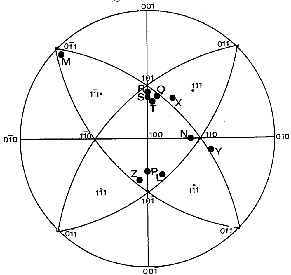
Tensile specimen deformed (1.2% plastic strain) at 923K
