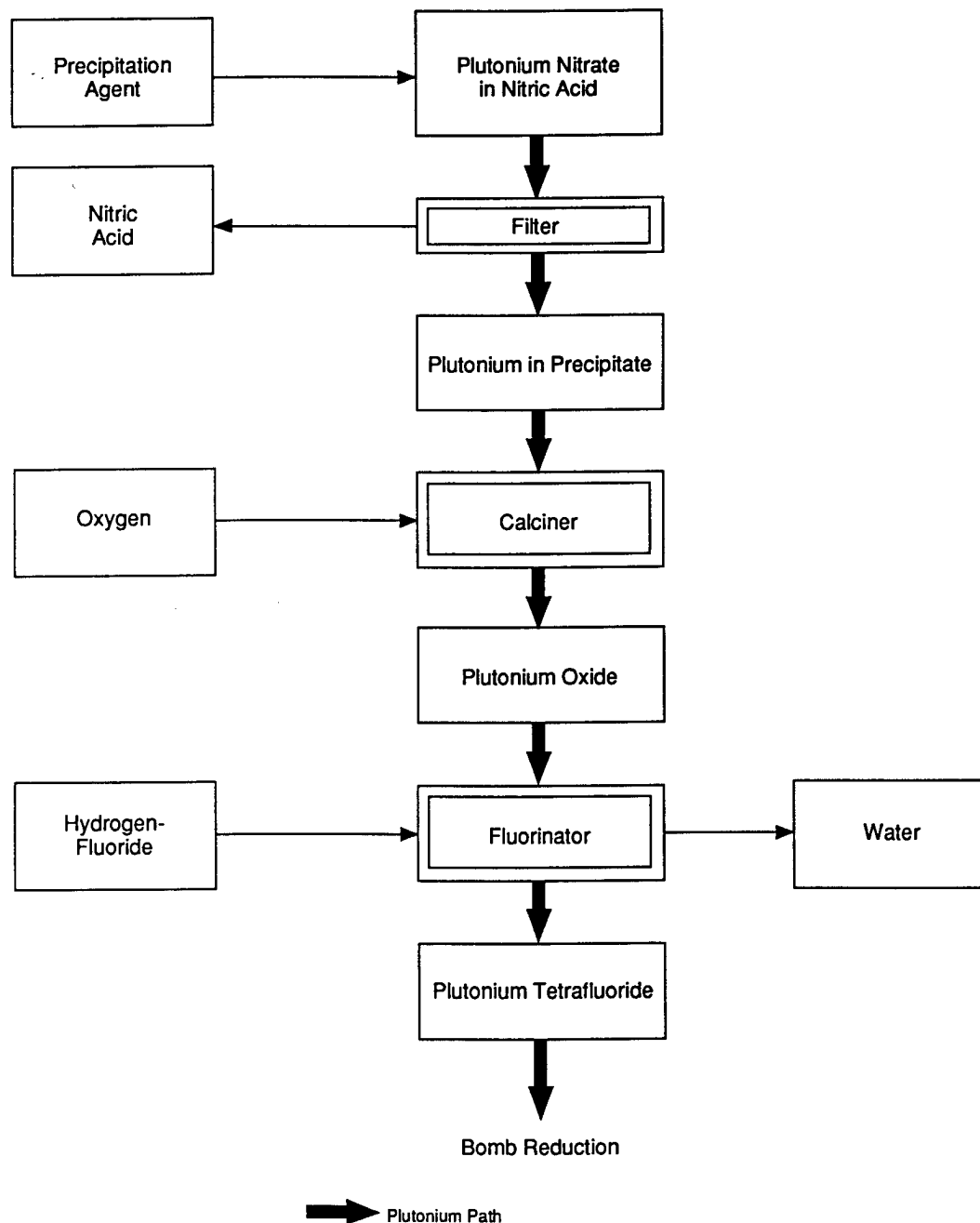
Figure 2.4: Aqueous Processing Final Steps
