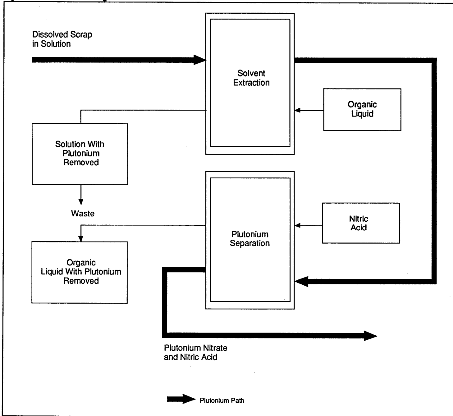
Figure 2.2: Purification Using Solvent Extraction
