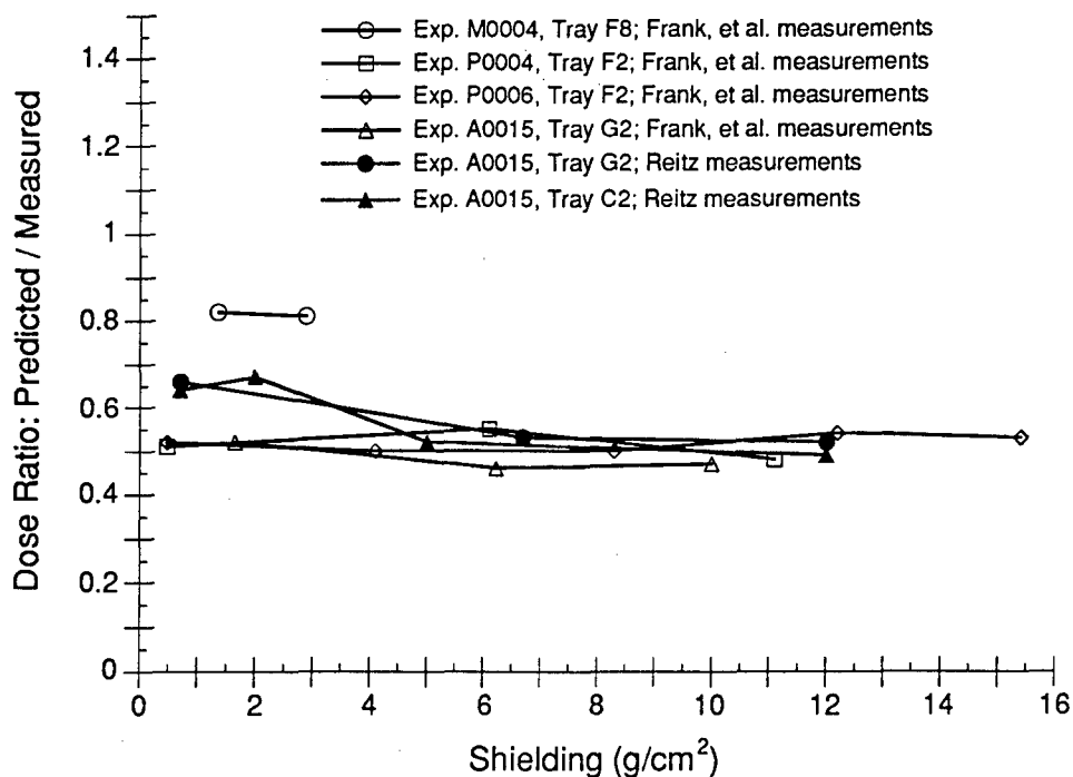
Figure 7. Ratio of predicted-to-measured radiation dose (in tissue) due to trapped proton environment based on LDEF data from thermoluminescent dosimeters.
