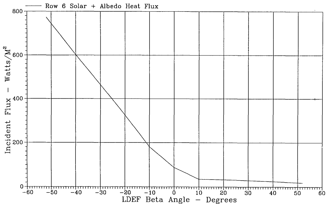
Figure 12. Row 6 orbital average heat flux vs LDEF beta angle.
