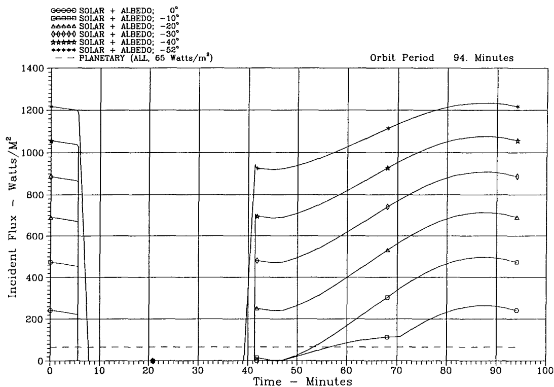
Figure 10. Row 6 orbital heat flux for negative beta angles.
