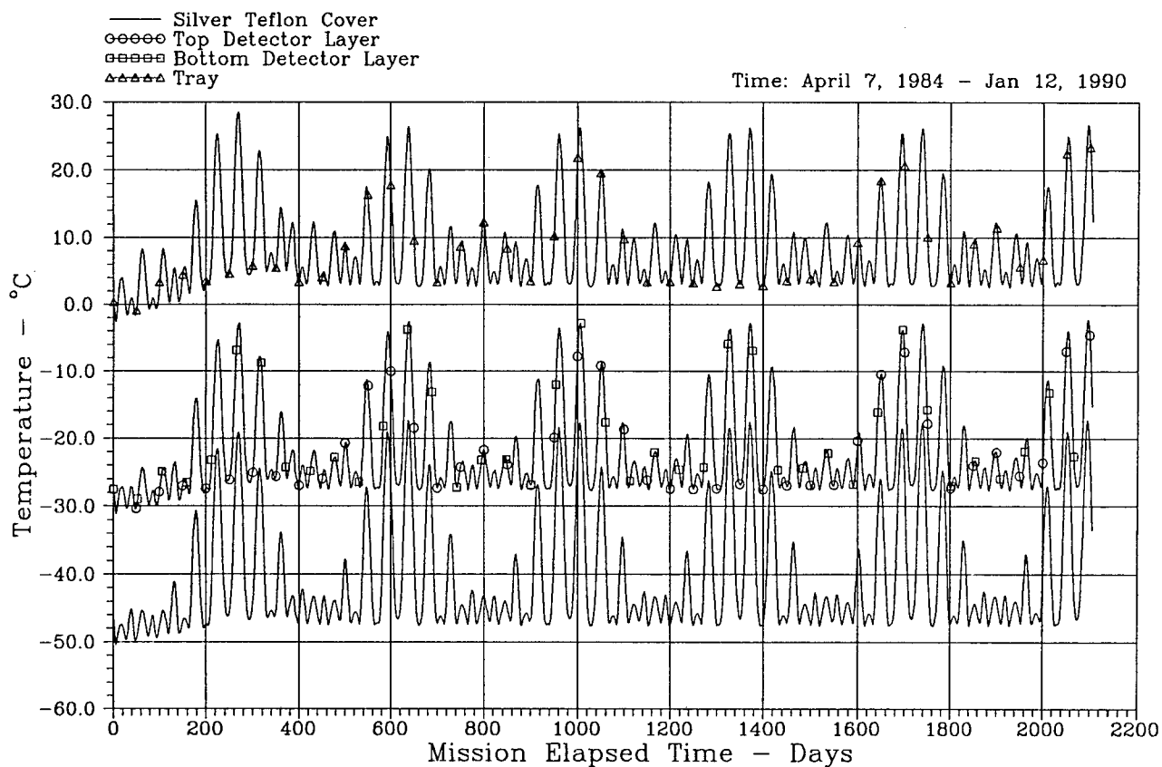
Figure 20. A0178-C6 Mission temperature history.
