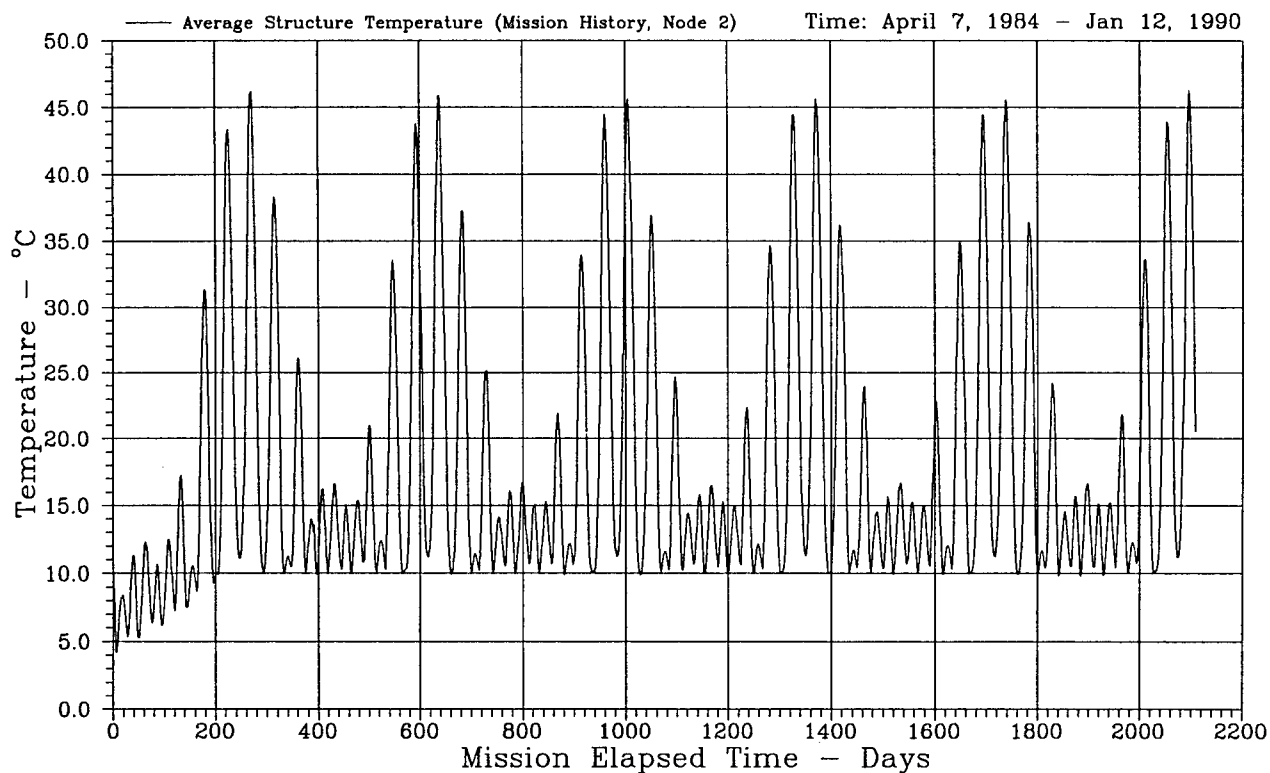
Figure 16. Mission average structure boundary temperature.
