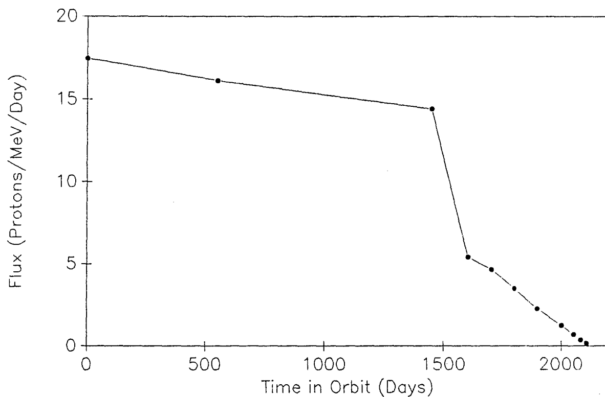
Figure 7. Proton Flux at 50 MeV as a Function of Time in Orbit
