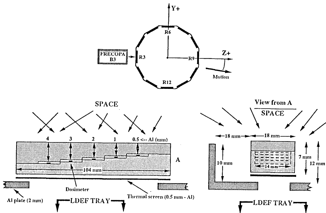
Figure 1 : FRECOPA location on board LDEF and dosimeter assembly
