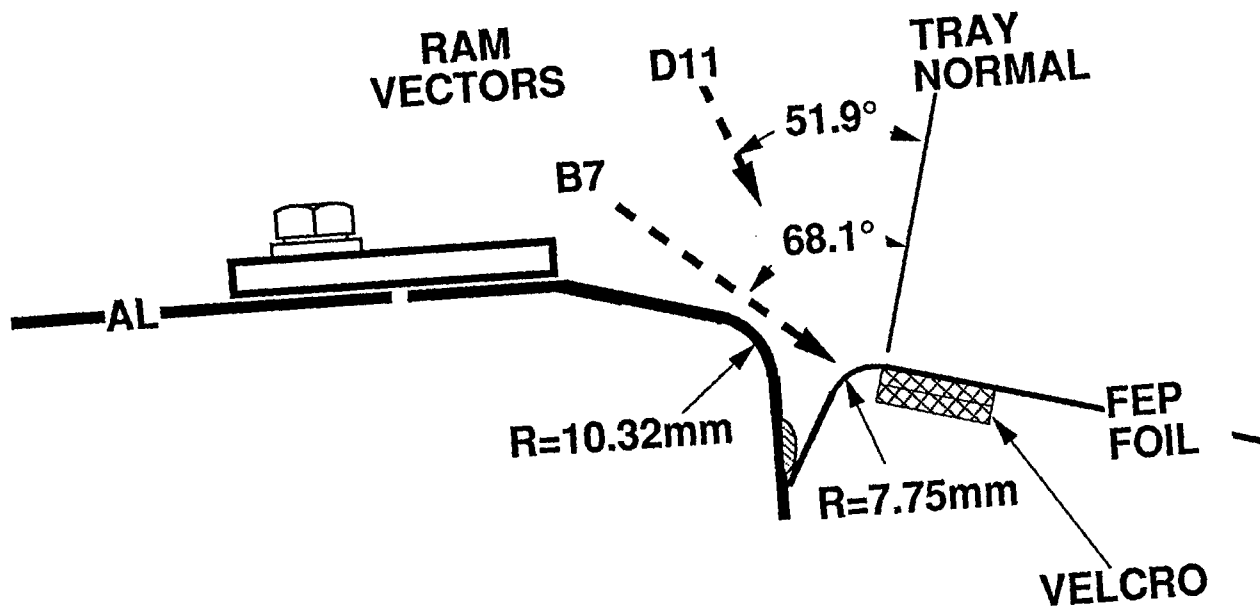
Figure 9. Shape of the edge attachment holding the thermal control blanket, Experiment Trays B7 and D11.
