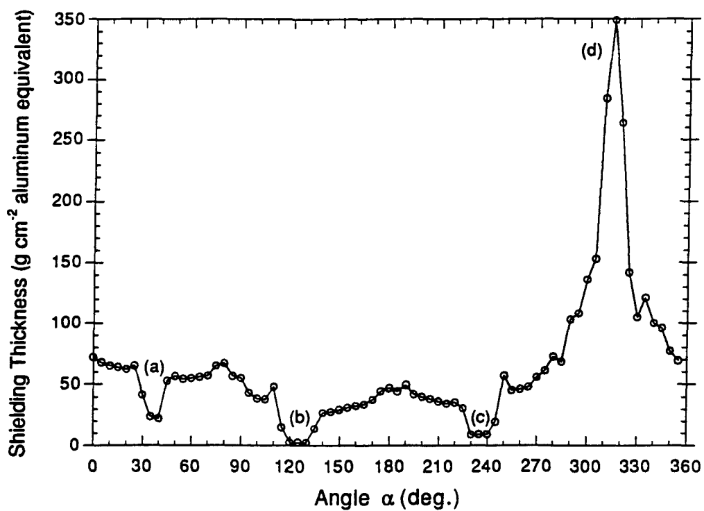
Figure 5. Shielding distribution in horizontal plane for a point on the surface of the detector module of Exp. P0006.
