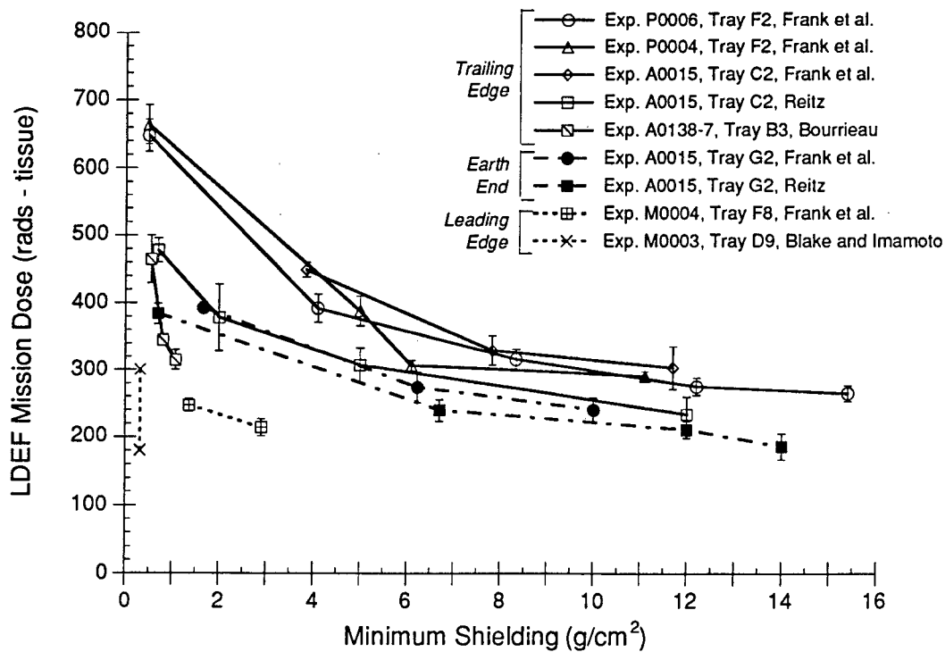
Figure 3. Summary of ionizing radiation dose measurements made on LDEF by thermoluminescent dosimeters (TLDs) at shielding depths where the dose is dominated by trapped protons.
