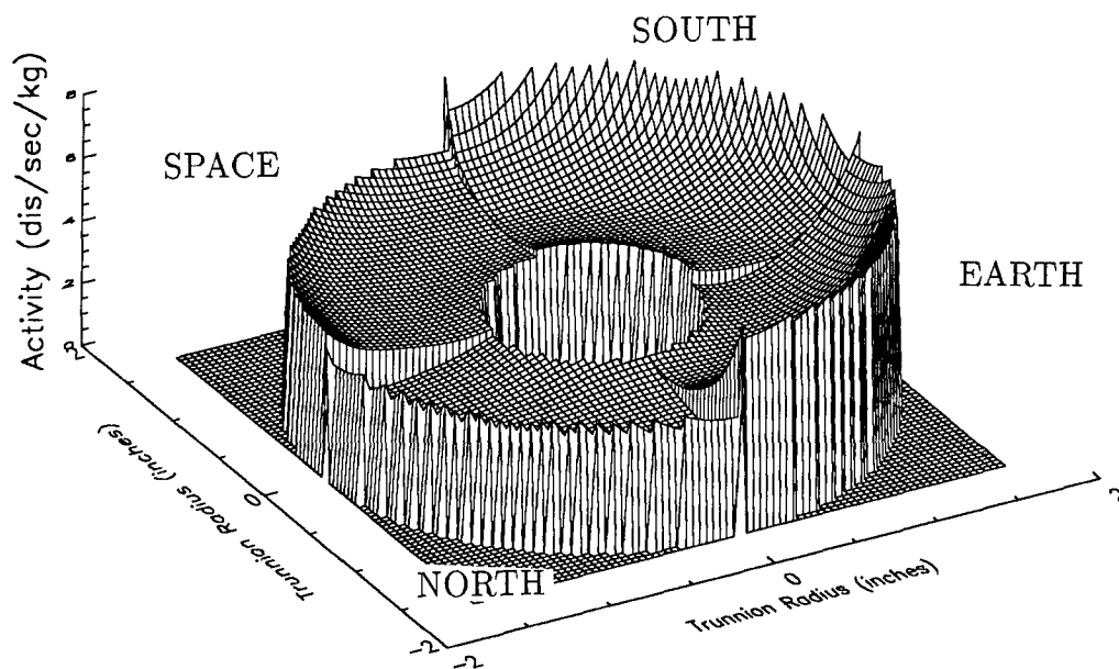
Figure 3. 54 Mn activity as a function of radius and direction for thin steel layers taken from the West (LH) trunnion. Top figure shows the activity profiles in the Earth, Space, North and South directions. Continuous curves represent a spline fit to the data. The spline fits were then used to create the bottom figure, which is an approximate two-dimensional representation of the activity throughout the cylindrical section. For clarity, no smoothing of the directional variation was performed.
