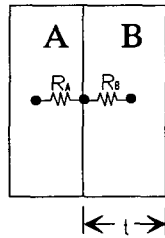
Figure 6. Thermal conduction network for the UHCRE experiment.
