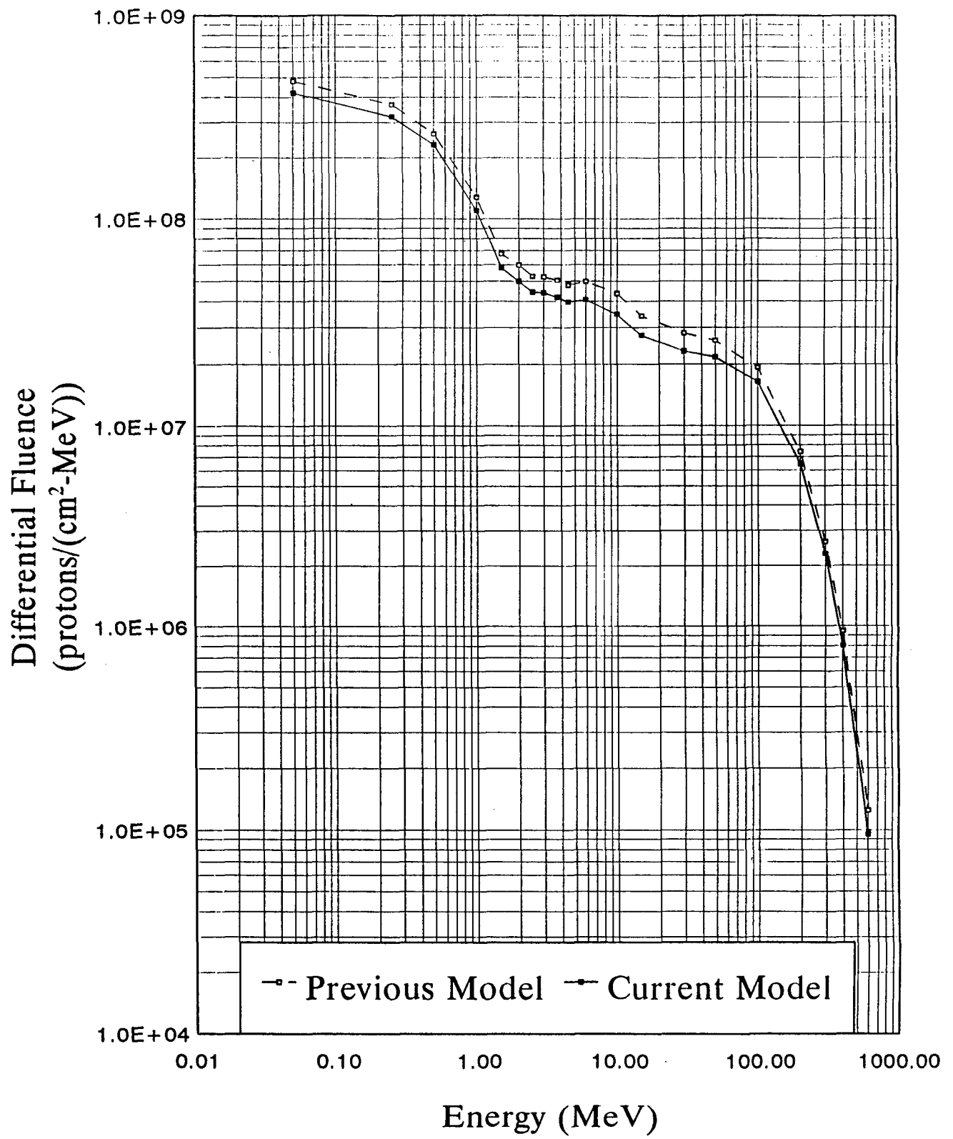
Figure 4. Current model proton mission fluence compared to previous model predictions (ref. 5).
