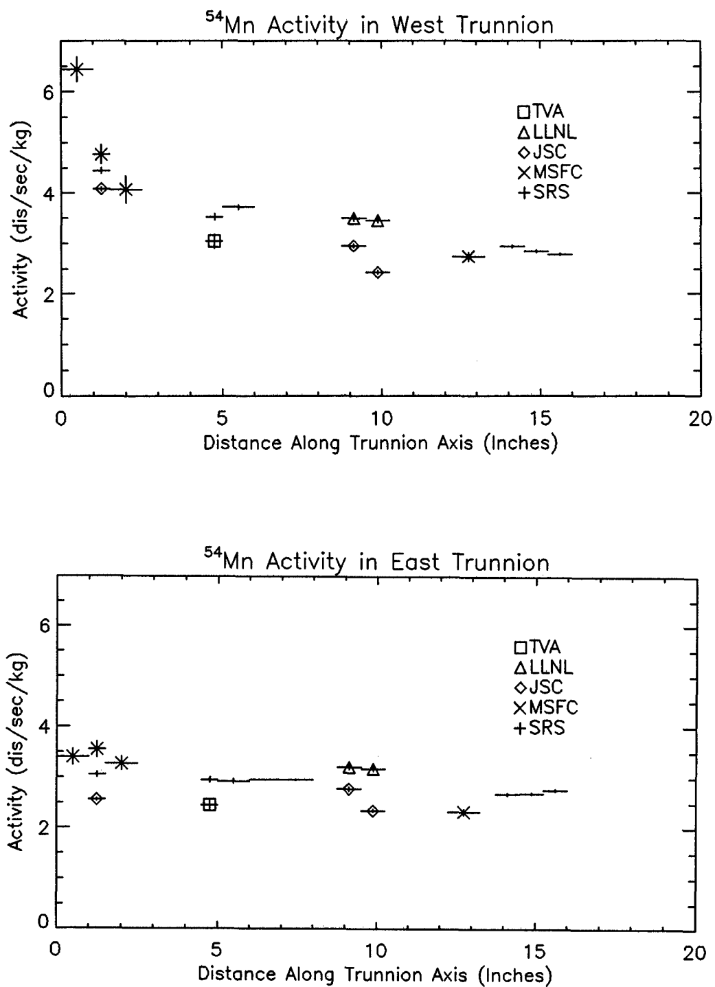
Figure 2. 54 Mn activities in the end frame steel trunnion as a function of distance along the trunnion center line. The origin of the horizontal axis represents the end of the trunnion farthest from the spacecraft.
