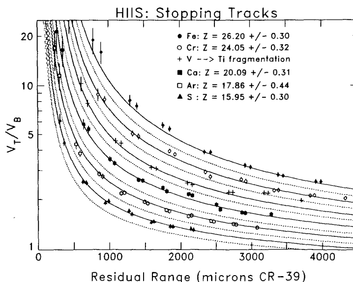
Figure 4: A sample of 6 stopping tracks, each represented with a different symbol. For clarity, only even Z-tracks are shown. The fitted atomic numbers with errors are also shown. Calibration curves, derived from the response function in Fig. 3 are shown for elements 15-26 (solid line: even-Z; dashed line: odd-Z). Note the fragmentation V to Ti.
