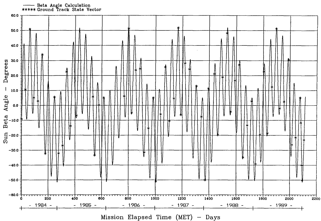
Figure 8. LDEF Beta angle history: April 7, 1984 - January 12, 1990.
