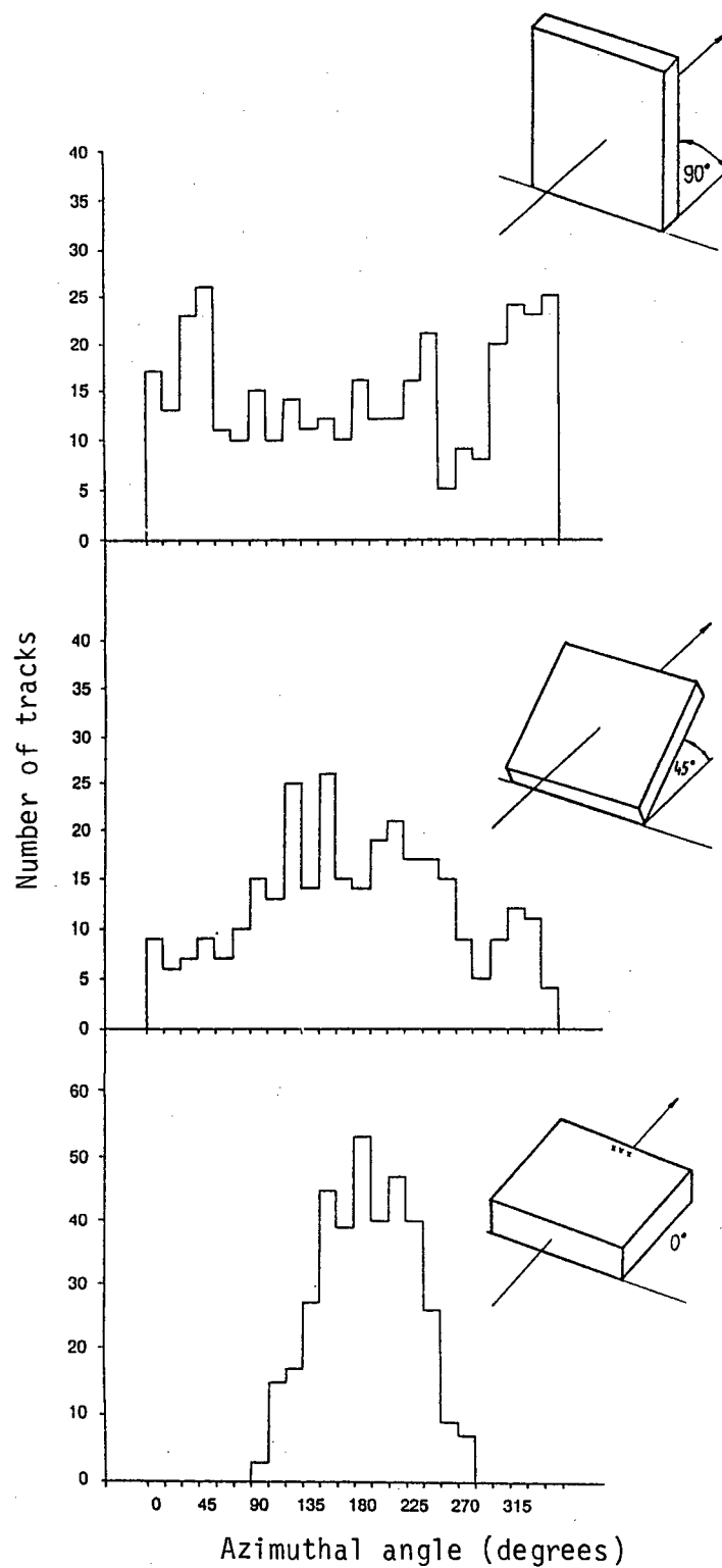
Figure 3: Azimuthal angle distributions of 300 energetic recoils produced by 200 MeV protons incident on CR-39 at various dip angles. Anisotropy of recoils show the directionality of the primary proton beam in the case of 45° and 0° dip angles.
