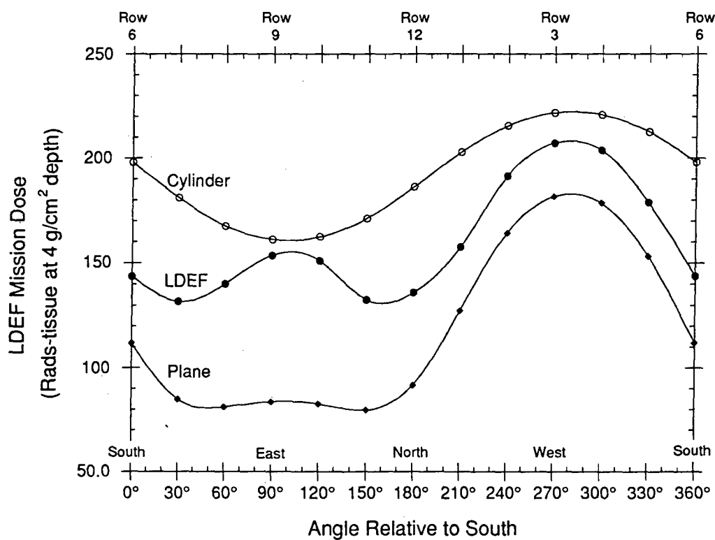
Figure 10. Influence of geomery model on predicted directionality of absorbed dose for LDEF mission due to trapped proton exposure.
