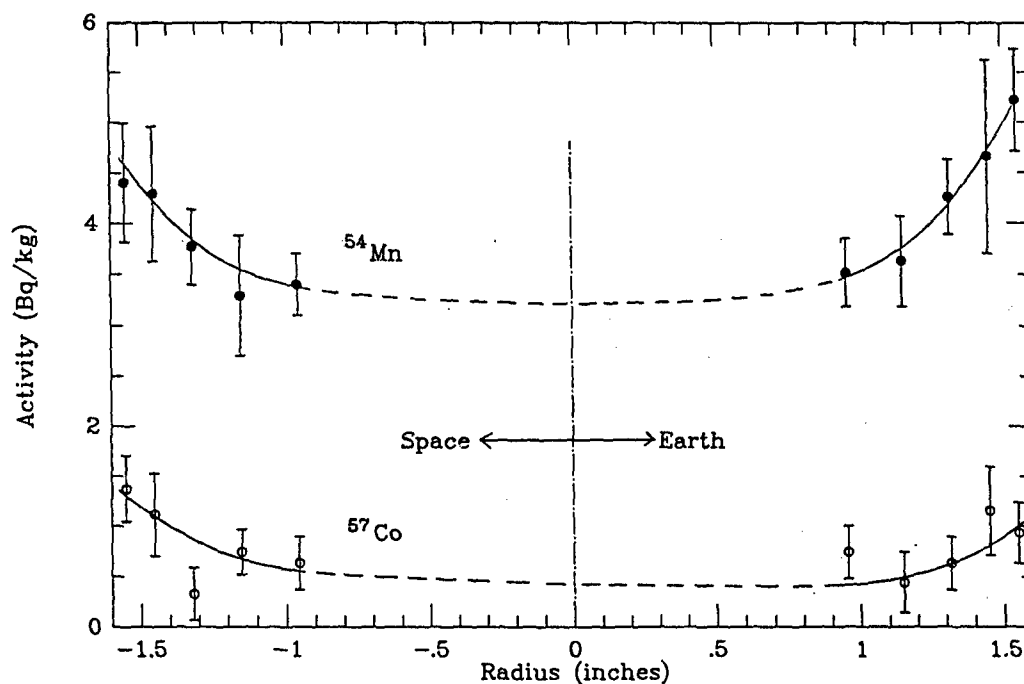
Figure 1. Induced radioactivity in section D of the left hand (west) trunnion. The curves are to guide the eye, especially to the enhanced activity near the surface and the flattening of the profile near the center.
