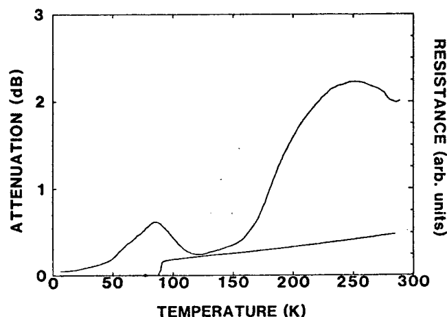
FIG. 1. The attenuation of 15 MHz longitudinal waves in a single-phased sample of \text{YBa}_2\text{Cu}_3\text{O}_7 in the temperature range from 7 to 289 K. The lower curve represents values for resistance measurements.
