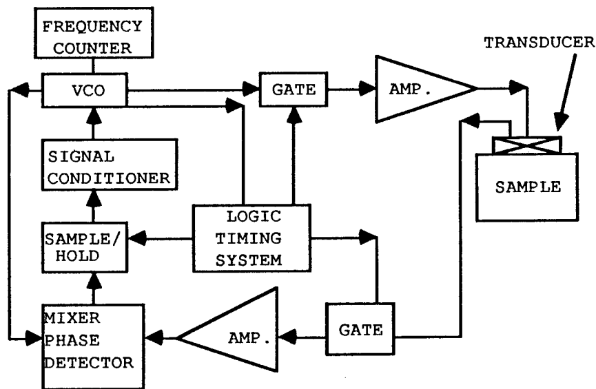
Fig. 1. Block diagram of the pulsed phase locked loop ultrasonic interferometer.
