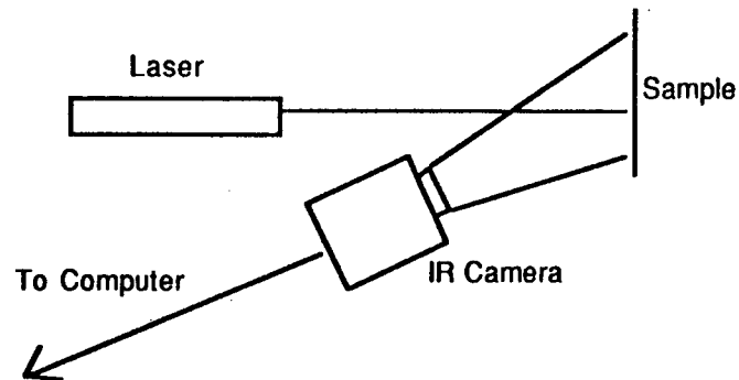
Figure 1: Experimental Schematic for In-Plane Measurements
