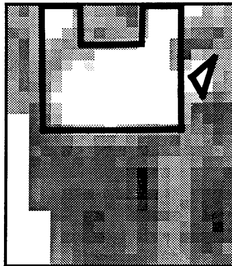
Figure 8. a) The C-scan image of the rough interface sample using a standard pulse echo system. b) The C-scan image of the rough interface sample using a phase insensitive array system.
