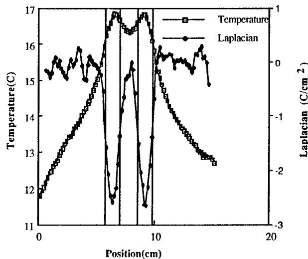
Figure 3. Profiles of Temperature and its Laplacian Across the Center of the Delaminations with Lines Drawn to Show Edges of Delaminations.
