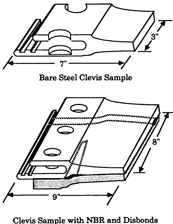
Figure 5. The two clevis samples used in this study. The first sample is a bare steel sample three inches across and seven inches long. The second sample is eight inches across and nine inches long, with NBR insulation bonded to it. Two disbonds were fabricated into this sample, indicated by dashed lines: a one-inch wide disbond running the length of the specimen and a wedge-shaped disbond running across the specimen and varying from two inches at the edge to approximately one-quarter inch at the center of the sample.
