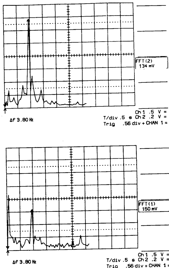
Figure 6. Frequency spectrum of vibration of a cantilever beam obtained with optical phase locked loop. Upper curve is the signal from the strain gauge and lower curve is the signal from the optical fiber.
