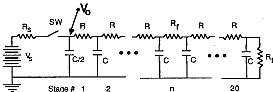
Fig. 2. Electrical circuit analogy to a one-dimensional heat propagation situation using a source connected by conductive transfer.
