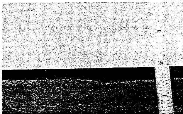
Figure 2. A photograph showing the cross-section of the inhibitor-liner-fuel system used in the SRM. The rough liner-to-fuel interface is visible.
