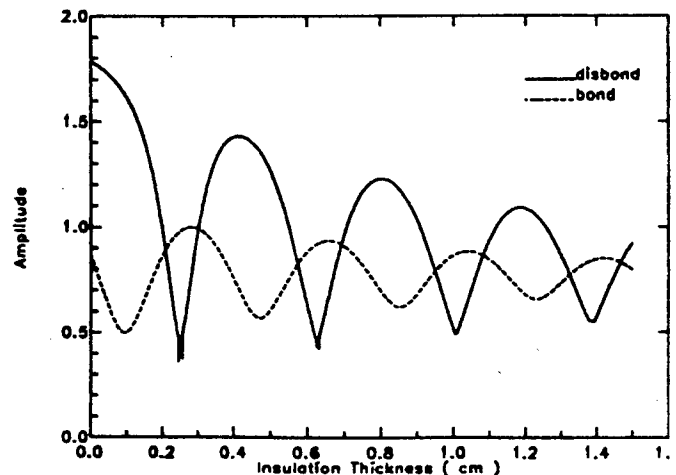
Figure 2. Calculated contrast levels at the first steel resonance of layered SRM system with varying thicknesses of insulation comparing a normal bonded sample with 0.127 m of steel, insulation, 0.0025 m of liner and 0.1016 m of inert fuel vs. a disbond condition between the liner and fuel.
