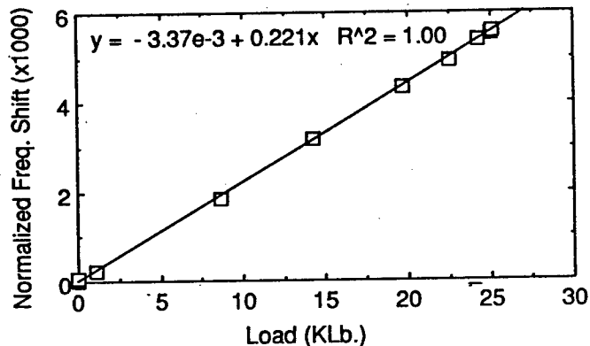
Figure 3 Bolt ultrasonic calibration (shuttle wheel).
