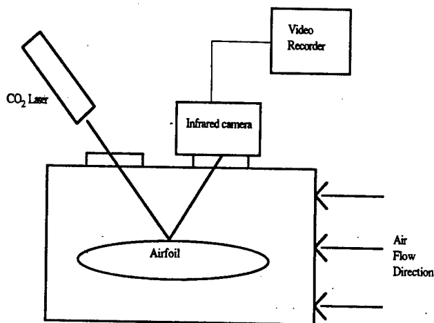
Fig. 1: Experimental Configuration
