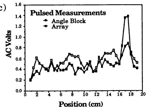
Figure 8. Results obtained from the disbond sample. (a) A sketch of the sample from above, showing the positions of the disbonds as shaded regions. (b) Results of measurements in continuous wave transmit mode. (c) Results obtained using tone burst transmit mode.
