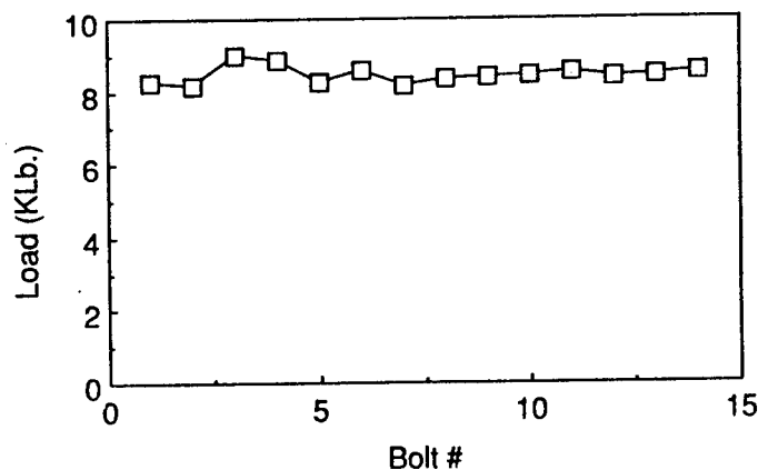
Figure 9 Magnetic Suspension Tunnel fan blade bolt loads.
