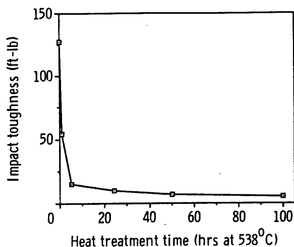
Fig. 1. Impact toughness vs. heat treatment time for CVN samples from slabs heat treated 0, 1, 5, 24, 50 and 100 hours, respectively, at 538 degrees C and broken at -1 degree C.
