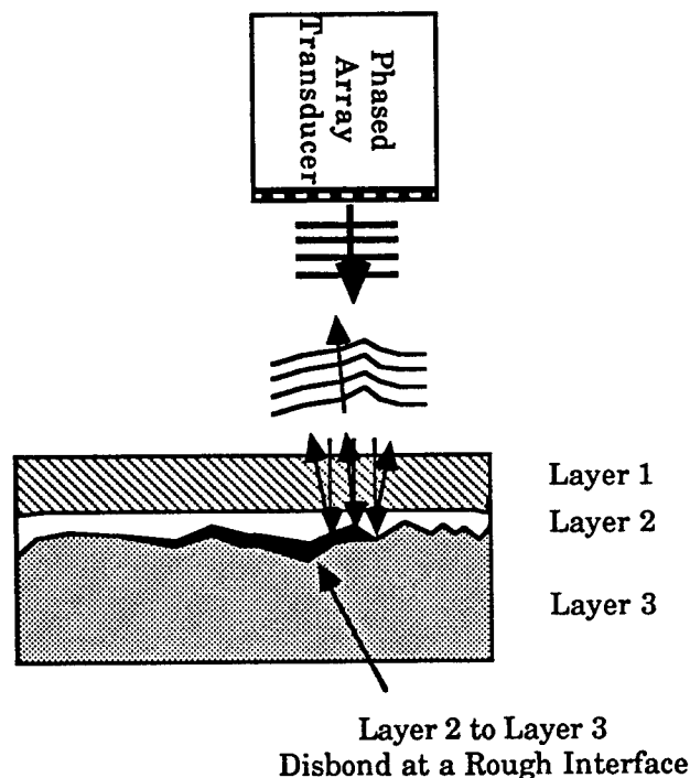
Figure 3. The concept of a phase insensitive array for detecting disbands at a rough interface.
