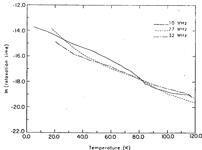
FIG. 2. Temperature-dependent relaxation time of \text{YBa}_2\text{Cu}_3\text{O}_7 .
