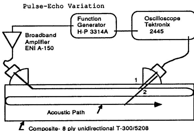
Fig.3 Equipment Arrangement for Pulse-Echo Velocity Measurements
