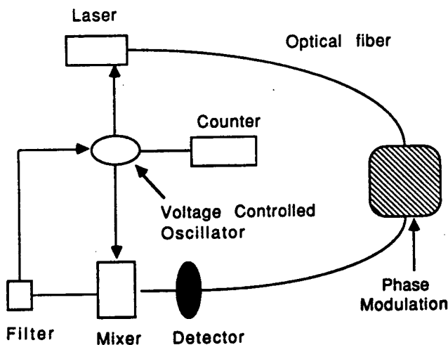
Figure 5. Schematic diagram of optical phase locked loop.
