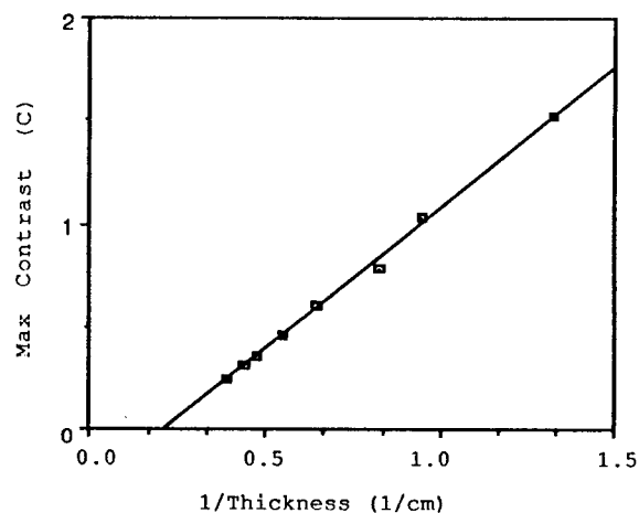
Figure 9. Maximum Contrast is Inversely Proportional to Steel Thickness.
