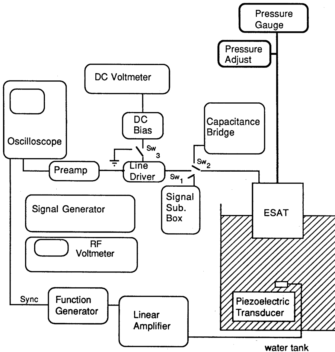
Figure 2. Experimental Setup
