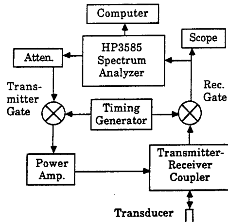
FIGURE 2- Block diagram of the experimental test set-up used to obtain ultrasonic spectral information on the SRM.
