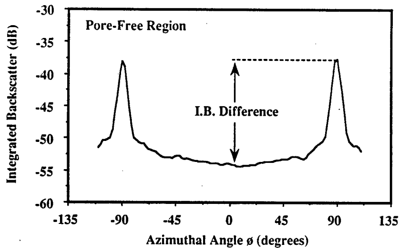
Figure 1: One measure of the anisotropy of polar backscatter is the integrated backscatter difference, defined as the difference in decibels between the maximum and minimum integrated backscatter as a function of azimuthal angle in a pore-free region. Data were obtained from a pore-free region of a uniaxial graphite/epoxy composite.
