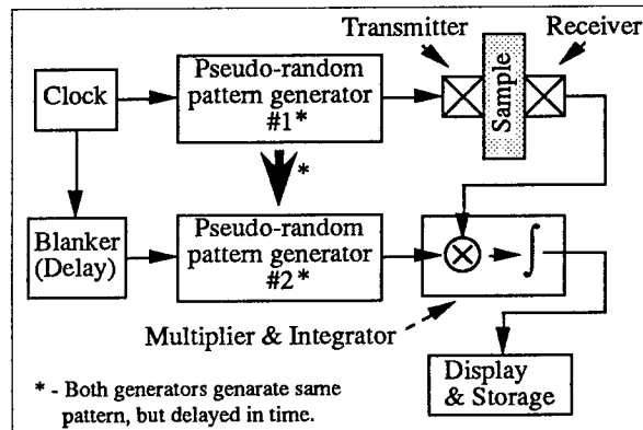
Figure 1. Correlator, schematics.
