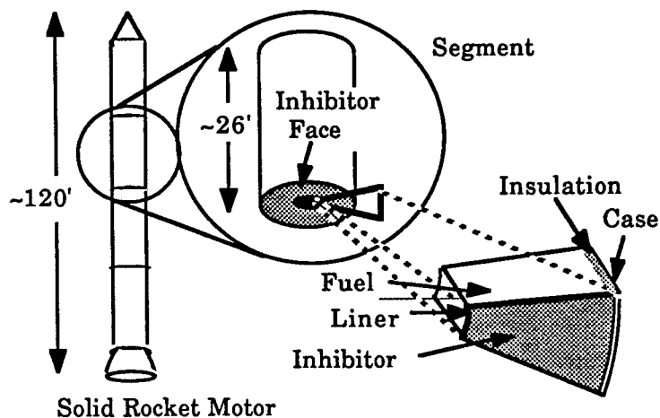
a) b) Figure 1a) A simplified drawing of the location of the inhibitor. 1b) A close up of the inhibitor-liner-fuel bond line roughness.
