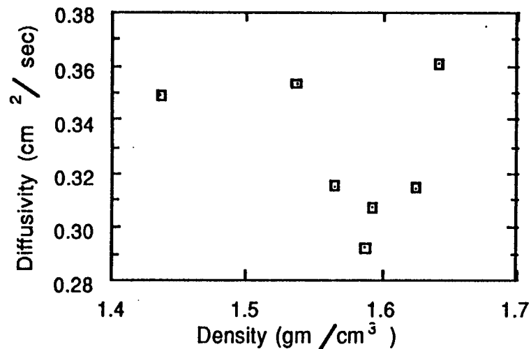
Figure 10: Diffusivity Versus Density Cross-fiber direction
