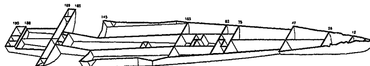
DOUBLE BOTTOM
