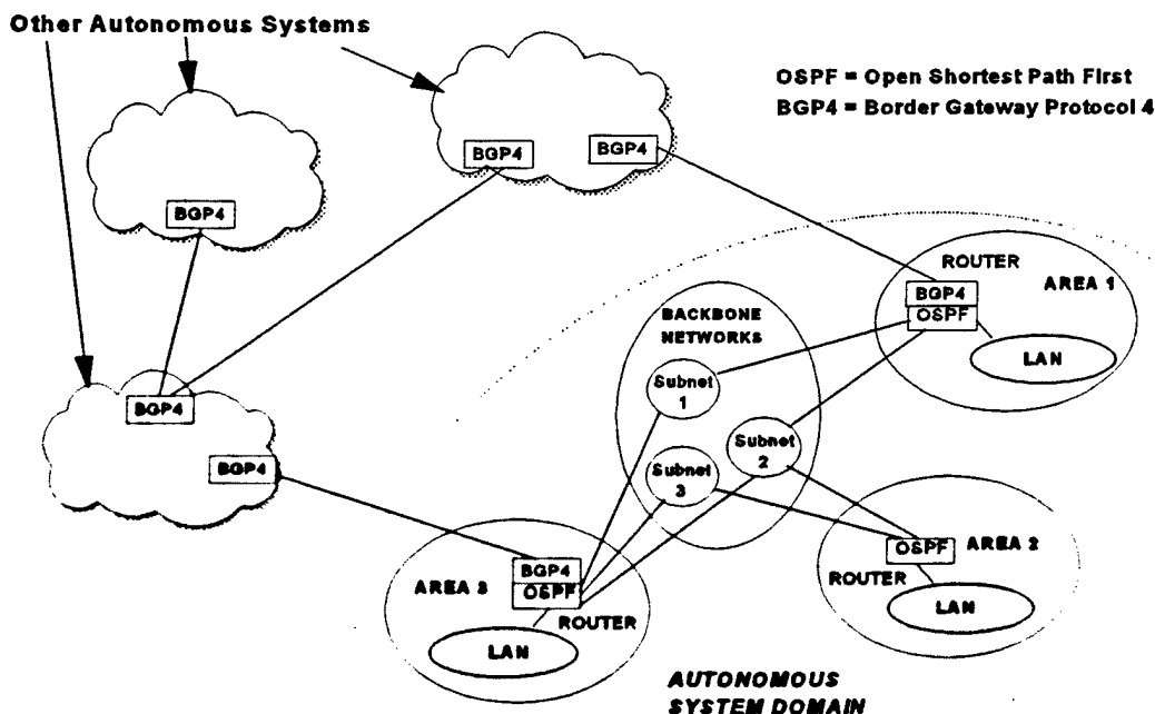
Figure 2.3 Autonomous System Boundaries and Routing Protocols (Casey, 1997)
