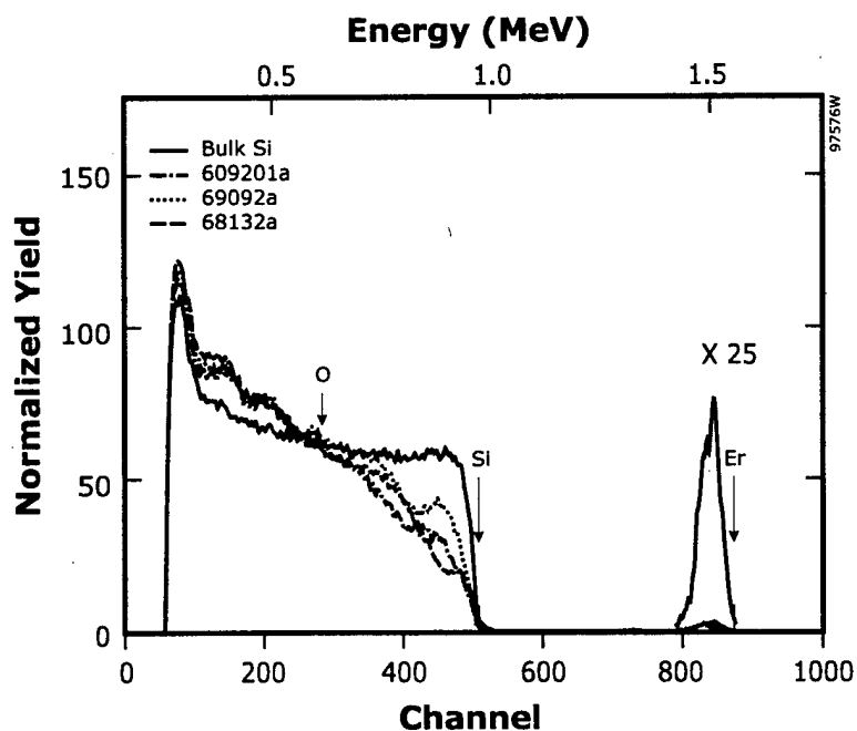
Figure 37 Comparison of RBS spectra of three porous Si wafers etched under identical conditions (100 mA, 60 min) and \text{Er}^{3+}:\text{Si} . All three porous Si samples had Al back contacts during etching.
