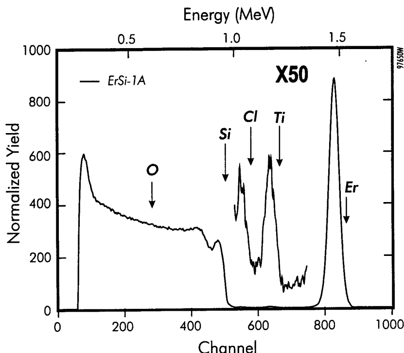
Figure 45 Near normal incidence RBS spectrum of \text{Er}^{3+} :Si sample Er-Si-1A. Erbium was implanted into this sample at 380 keV with a fluence of 4.9 \times 10^{15} \text{ cm}^{-2} .
