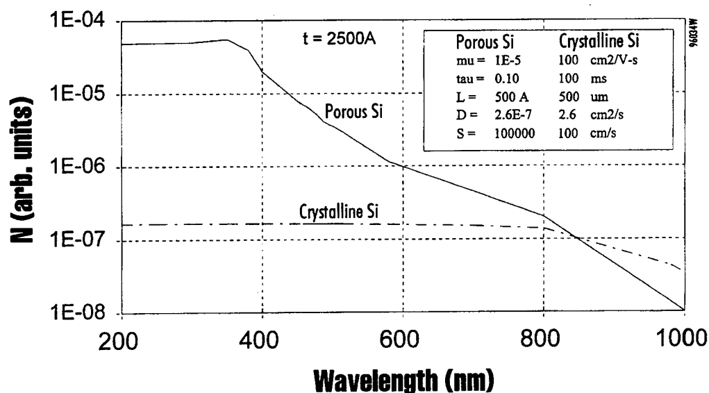
Figure 23 Carriers generated for excitation wavelength from 200 to 1000 nm for bulk Si and porous Si with a thickness of 2500Å. For wavelengths shorter than 400 nm, carriers are influenced by surface recombination.
