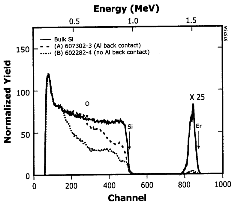
Figure 36 Comparison of RBS spectra of two porous Si wafers, (a) with and (b) without Al back contacts etched under identical conditions (100 mA, 60 min). An RBS spectrum of Si is shown for reference.
