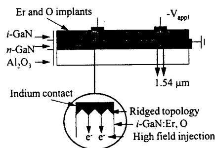
FIG. 1. A side view schematic of a GaN:Er,O implanted m-i-n LED. The substrate is R -plane sapphire, and the i and n -GaN layers were grown by CVD. The i -GaN layer was ion implanted with 10^{15} \text{ Er}^{2+}/\text{cm}^2 at 350 keV, and coimplanted with 10^{16} \text{ O}^+/\text{cm}^2 at 80 keV. A postimplant anneal in a MOCVD quartz reactor at 800^\circ\text{C} for 45 min in flowing \text{NH}_3 was performed. The metal contacts are indium.
