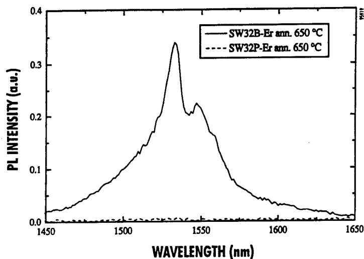
Figure 28 Room-temperature IR PL spectra of Er implanted at 190 keV with a dose of 10^{15} \text{Er}^+/\text{cm}^2 into red-emitting porous Si which peaked at 750 nm. Strong IR emission was observed for the porous Si after annealing at 650 C. In contrast, no IR emission was observed from Er implanted under similar conditions into porous Si which peaked at 650 nm.
