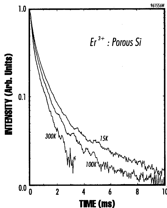
Figure 24 1.54\text{ }\mu\text{m} PL decay curves of Er:porous Si measured at 15, 100 and 300K.
