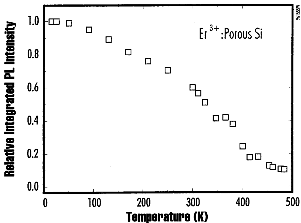
Figure 14 Normalized 1.54 μm integrated PL intensity of Er 3+ :porous Si measured from 15K to 475K.
