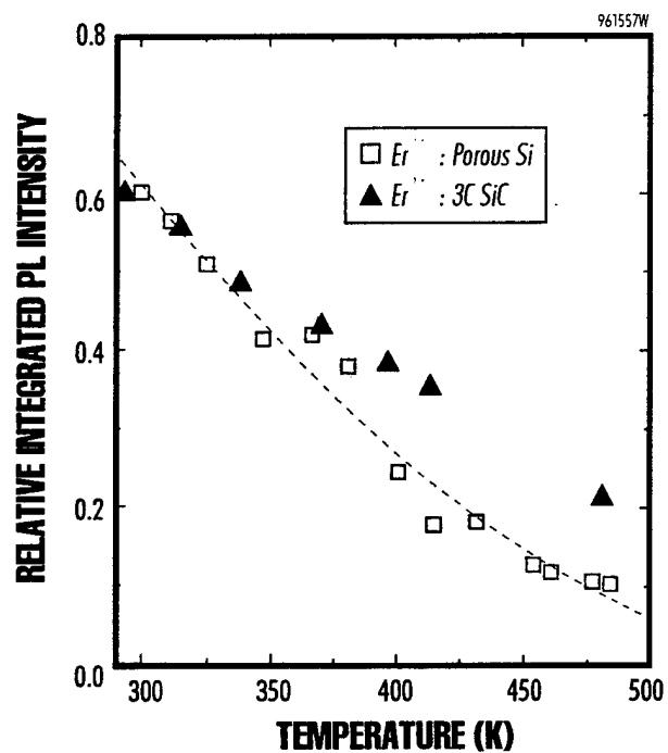
Figure 15 Comparison of temperature dependence of 1.54 μm PL emission in Er:porous Si and Er:3C-SiC. 28
