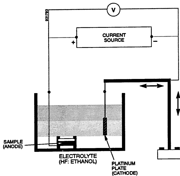
Figure 5 Schematic diagram of the anodic etching apparatus used at Spire for fabricating porous silicon wafers.
