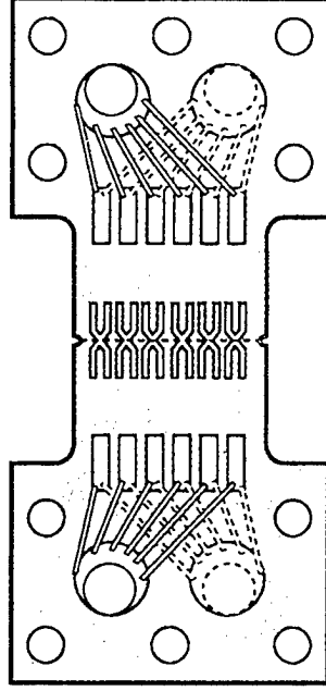
STACKED PLATELET THROUGH VIEW
