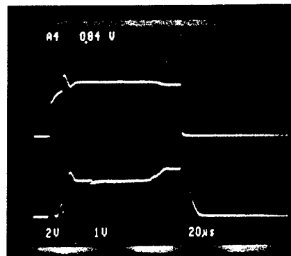
Figure 5.19a. Detected forward and reflected rf waveforms, under closed-loop control with beam.
