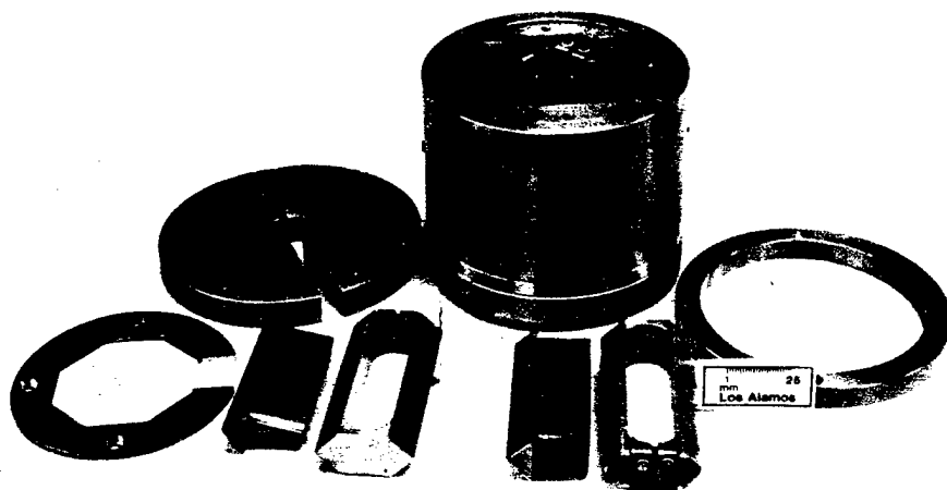
Figure 3.5. Photograph of the iron-core superconducting quadrupole.
