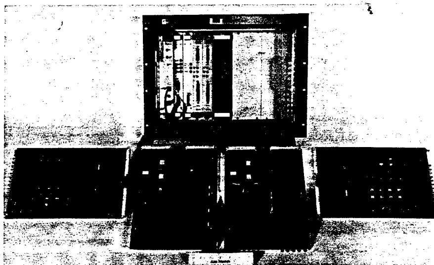
Figure 5.17. AT-5 custom-designed VXI modules for GTA LLRF system.
