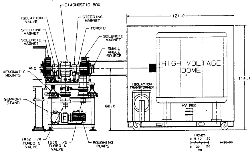
Figure 10.3. Schematic of the GTA injector.
