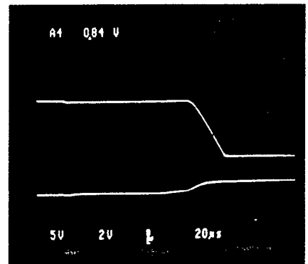
Figure 5.20b. I&Q integral error signals.
