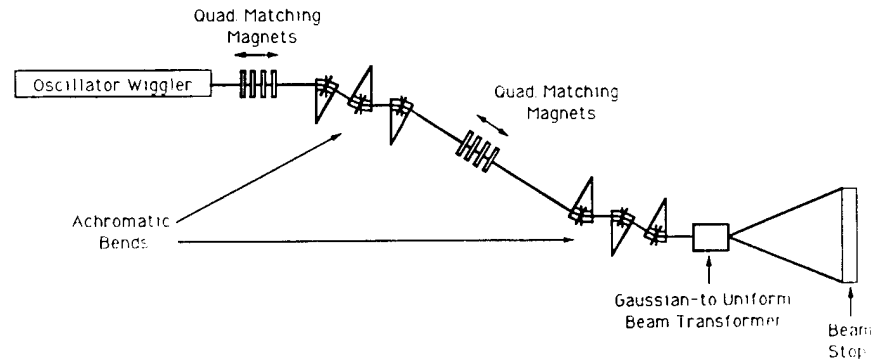
Figure 3.4. Conceptual layout of the GBFEL post-wiggler electron-beam transport system.
