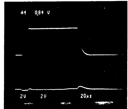
Figure 5.19b. Detected in-phase (I) and quadrature-phase (Q) components of cavity field.
