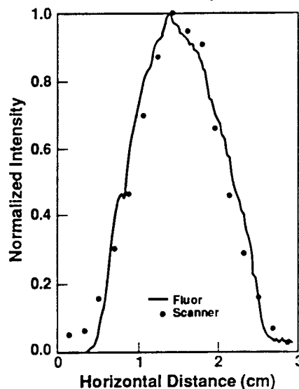
Figure 10.6. Horizontal profile of Figure 10.5 data.
