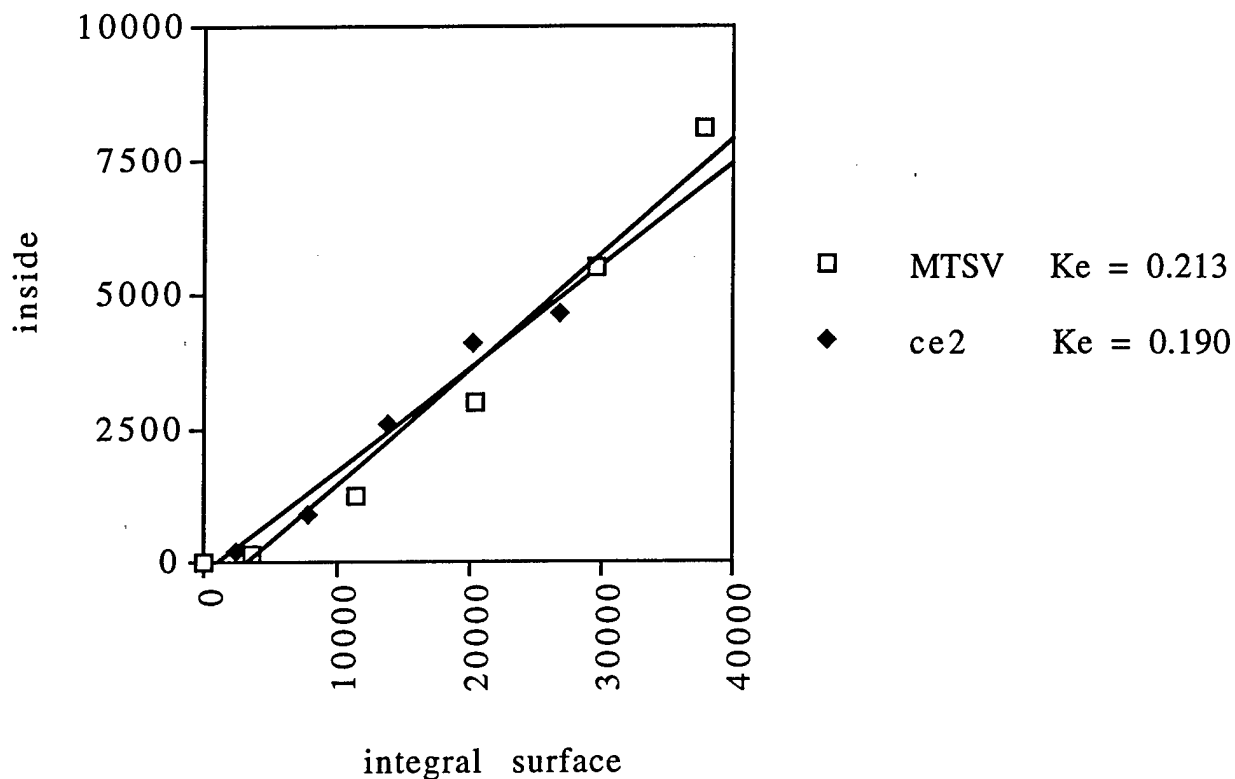
Figure 4. Internalization of the EGF-R is not affected by HER2 overexpression. Cells are incubated with 10ng/ml radiolabeled EGF for a 5 minute time course. Every minute cell surface and internalized counts are measured. The slope of the line yields the internalization rate constant ( K_e ).
