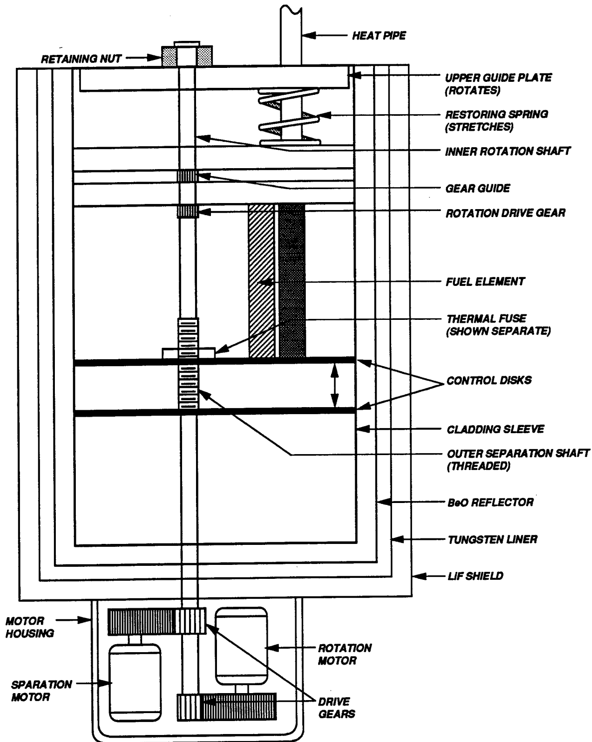
Figure 2.18 \text{Am}_2\text{O}_3 Fueled Reactor Core with No Energy Storage (Concept C)
