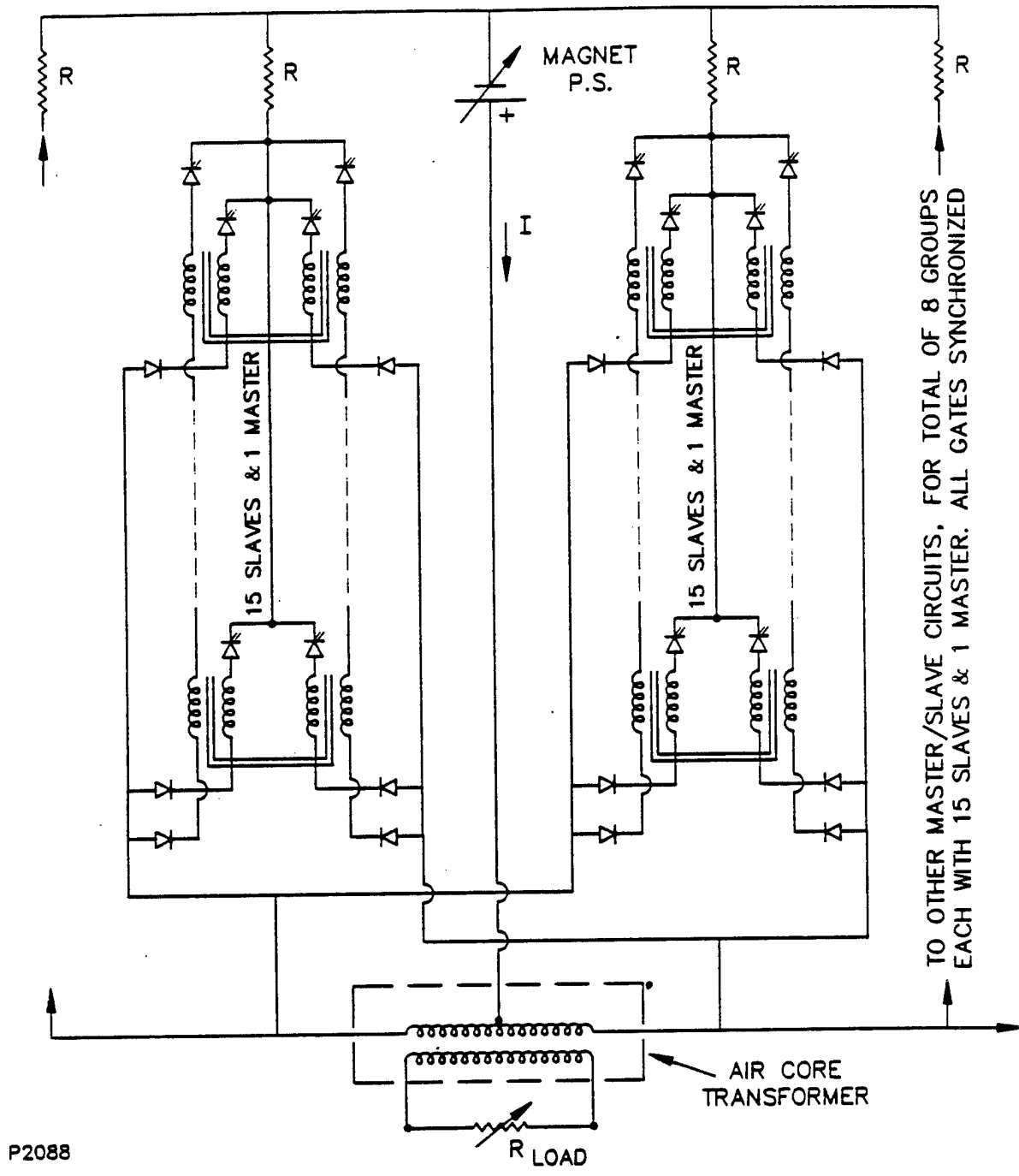
Figure 28 Schematic of the Initial Test Circuit
