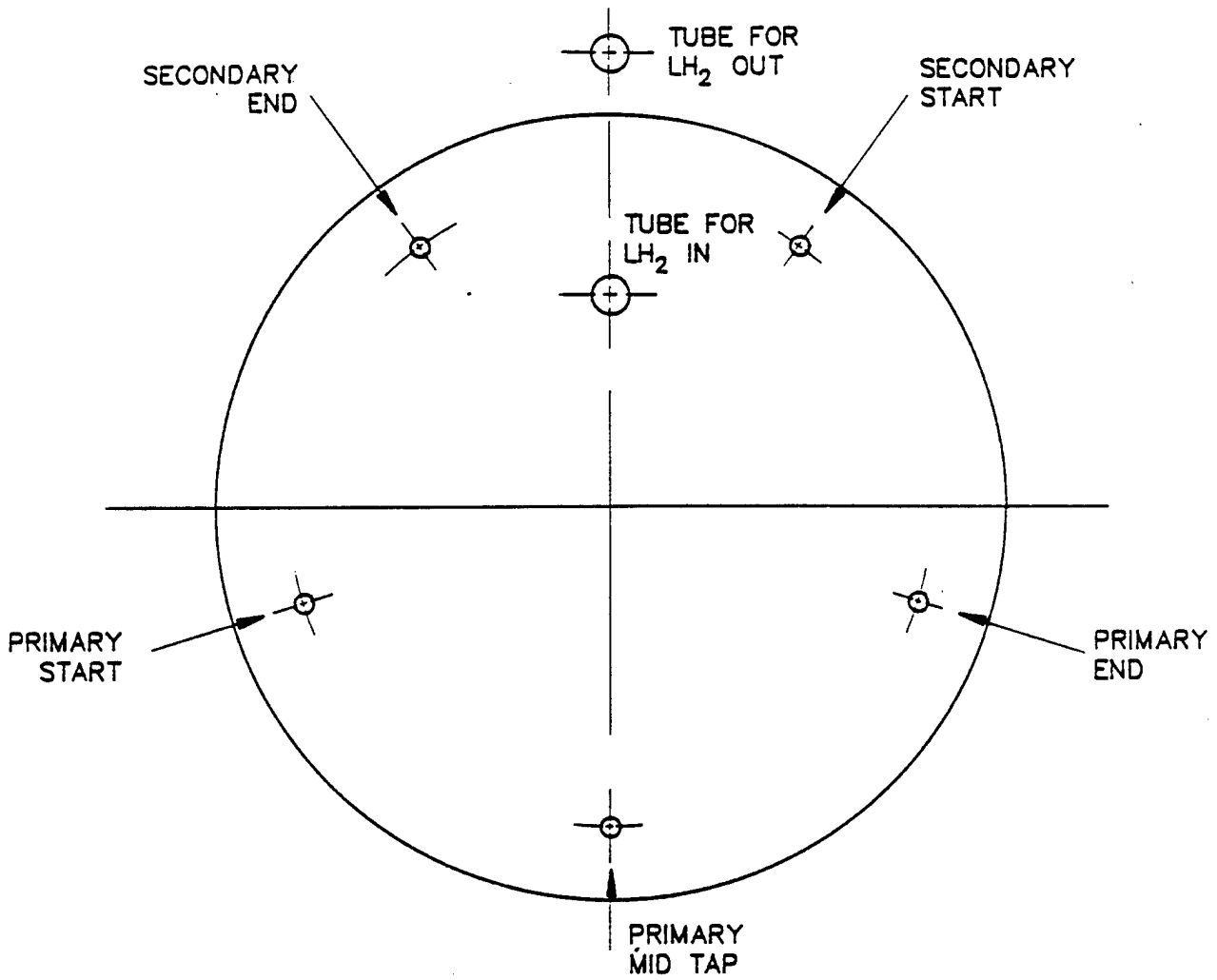
Figure 13 Schematic of the Start/Termination of the Primary and Secondary Conductors as Viewed from the Top of the Transformer
