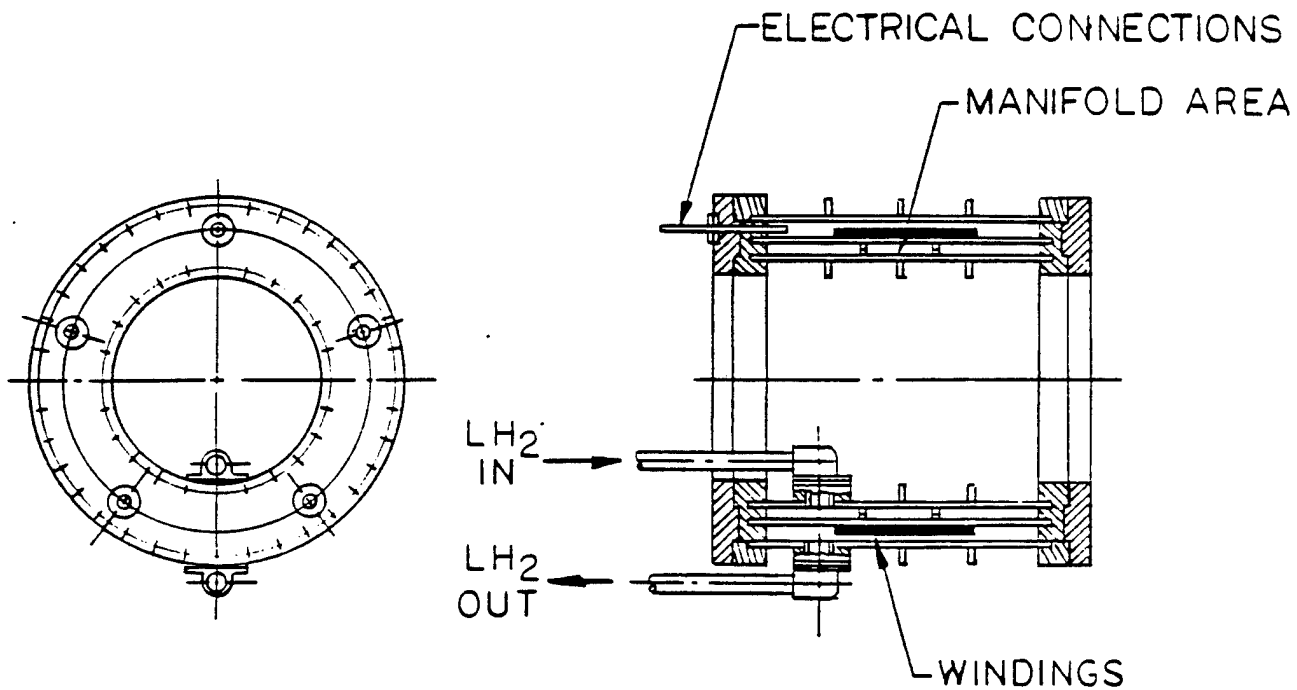
Figure 2b Overall Assembly of High Risk Design No. 10
