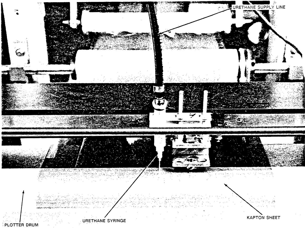
Figure 8 Close-Up of the Urethane/Syringe Drawing Urethane Lines on the Insulator Sheet (KAPTON)
