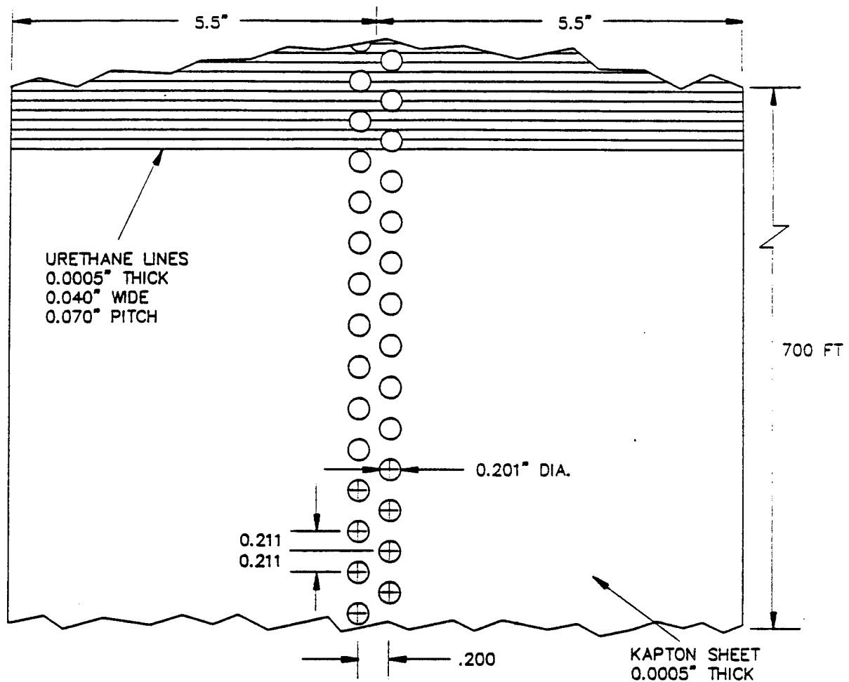
Figure 9 Schematic of the Perforations in the KAPTON Insulating Sheet
