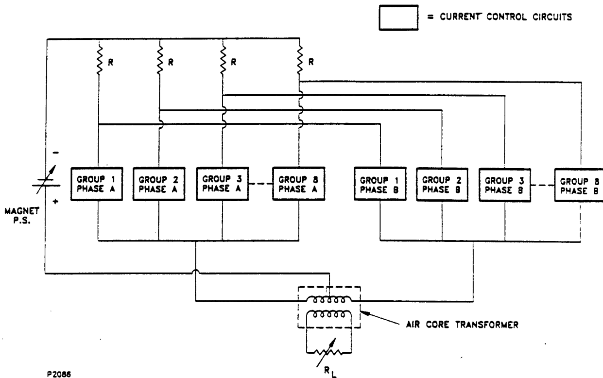
Figure 29 Block Diagram of the Transformer Test Circuit. Up to 4000 A Primary Current Switched By Current Control Circuits (128 GTO's in Parallel for Each Phase).
