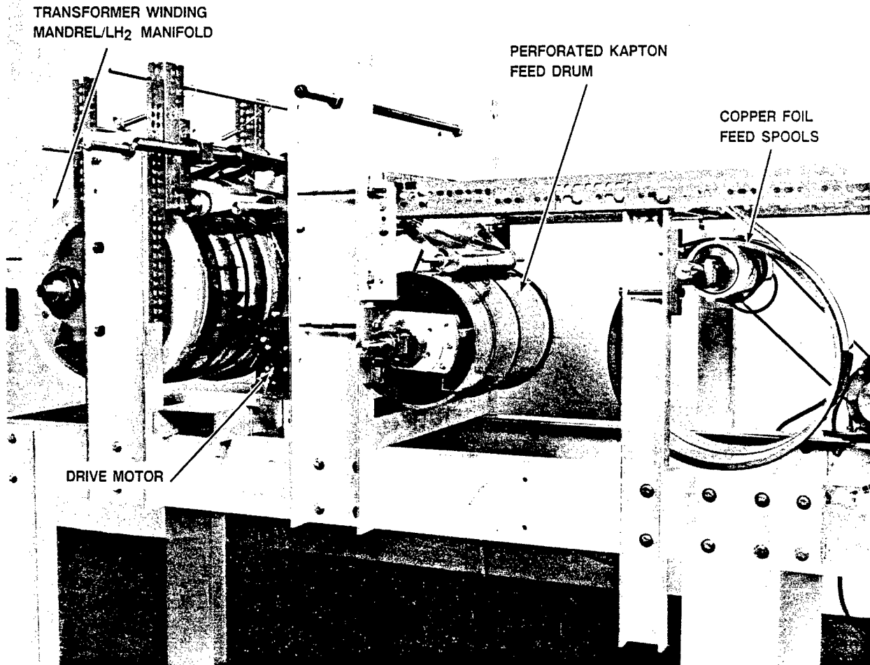
Figure 11 Photo of Winding in Progress
