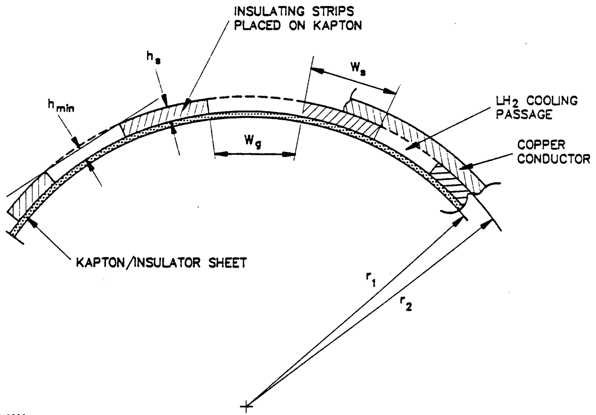
Figure 5 Geometry and Dimensions of the LH 2 Cooling Passages
