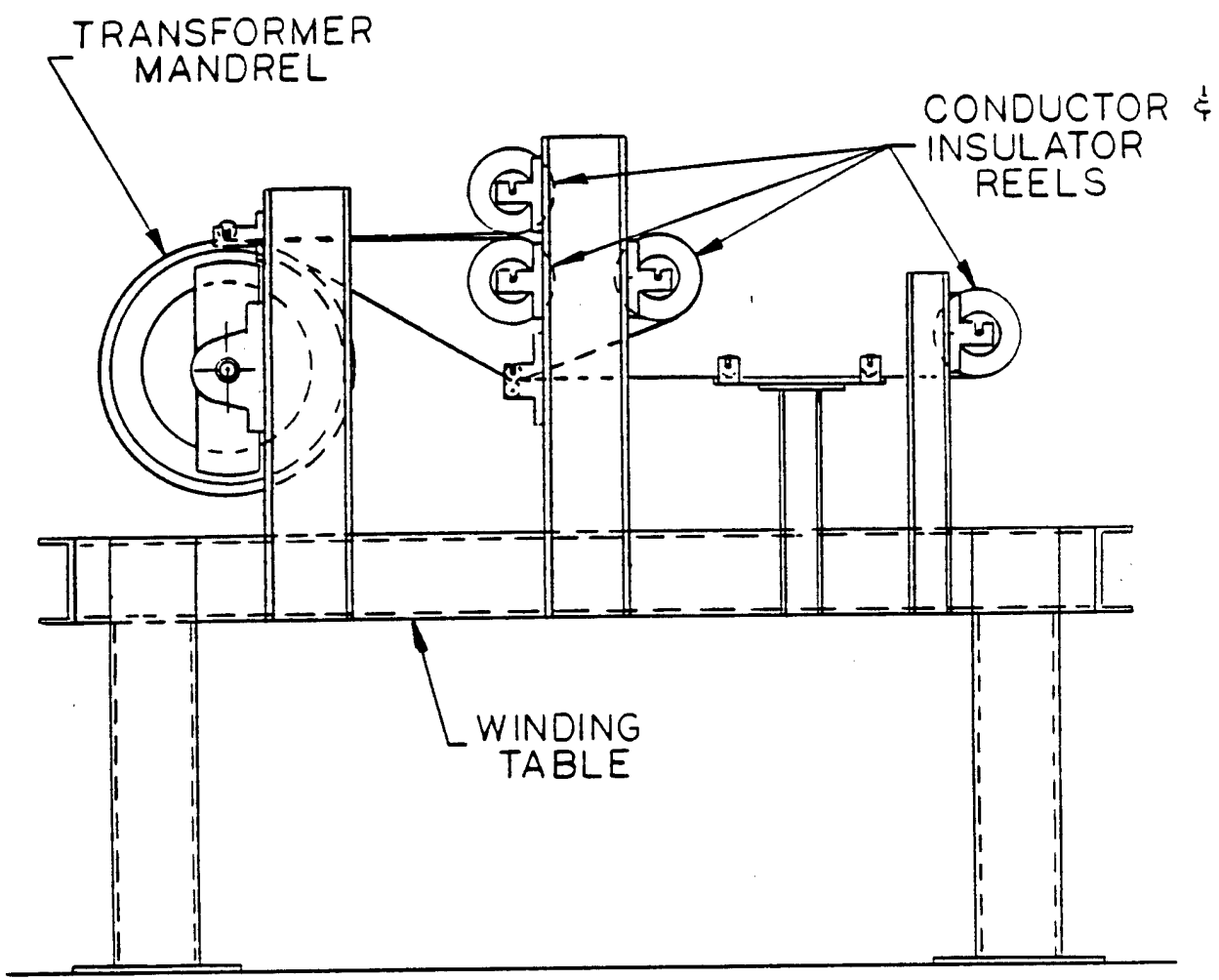
Figure 6 Schematic of the Winding Machine
