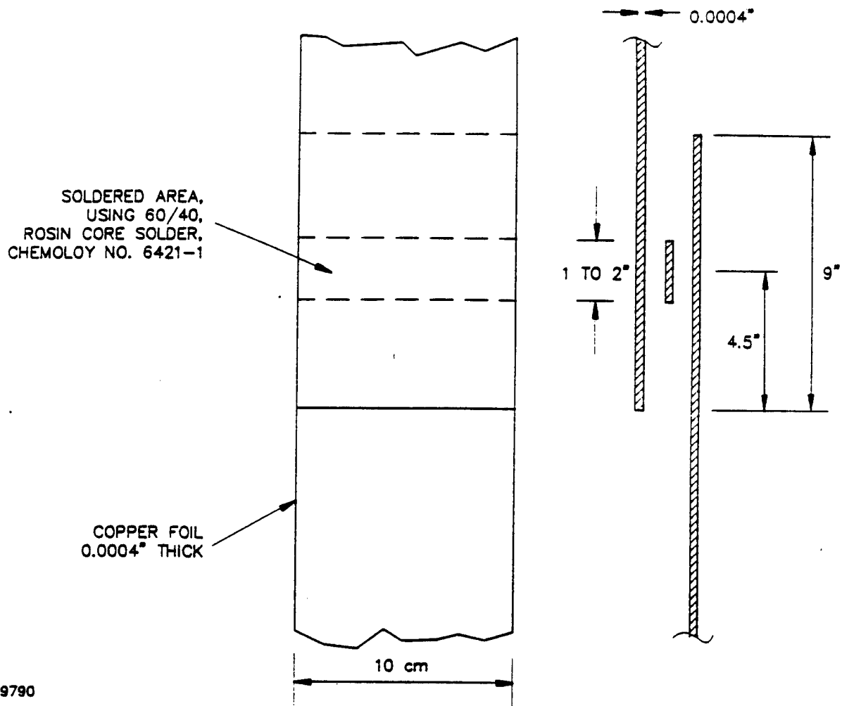
Figure 12 Schematic of the Secondary Coil Splices
