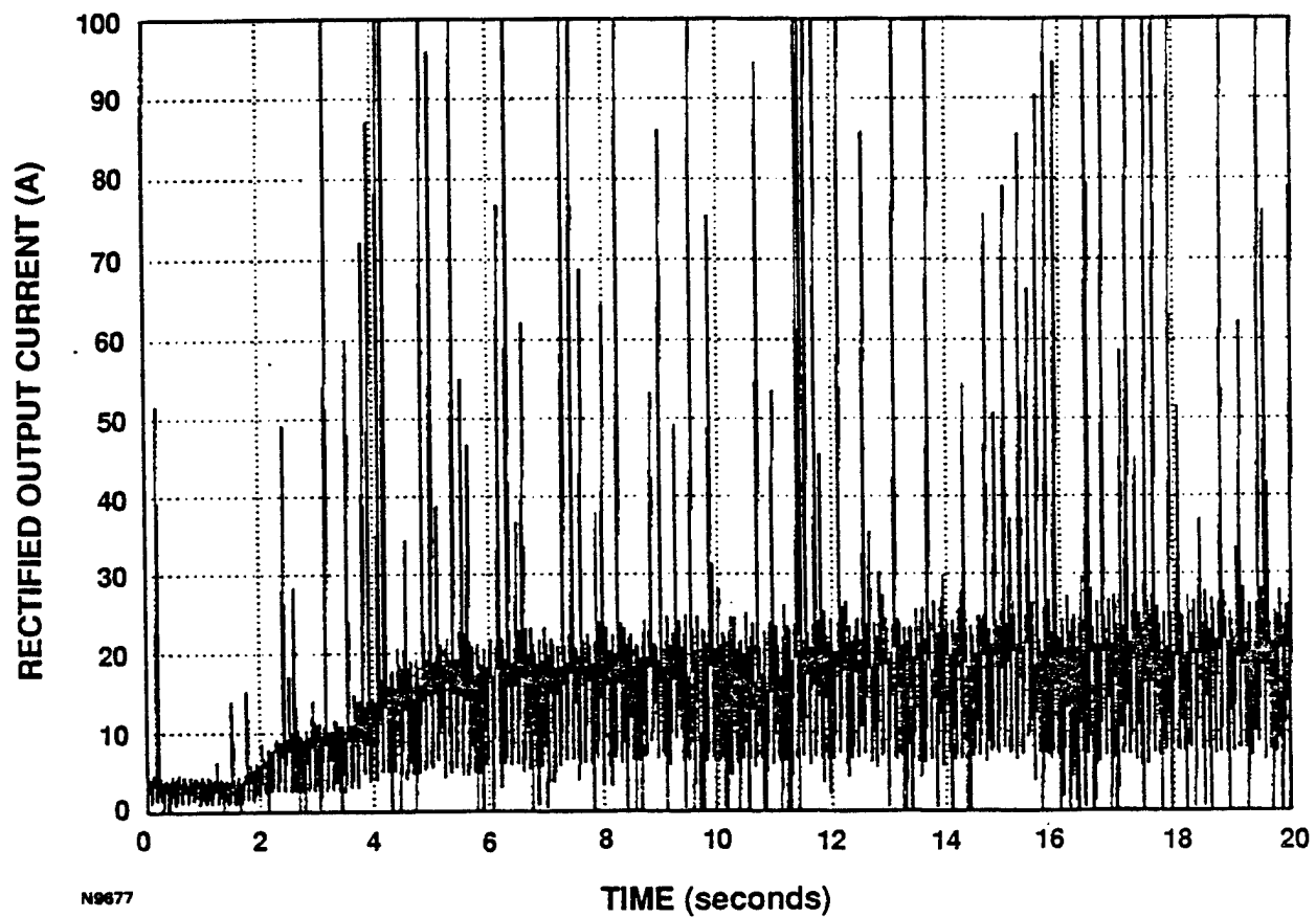
Figure 34 Rectified Output (Secondary) Current Over a 20 sec Period After the Test Start
