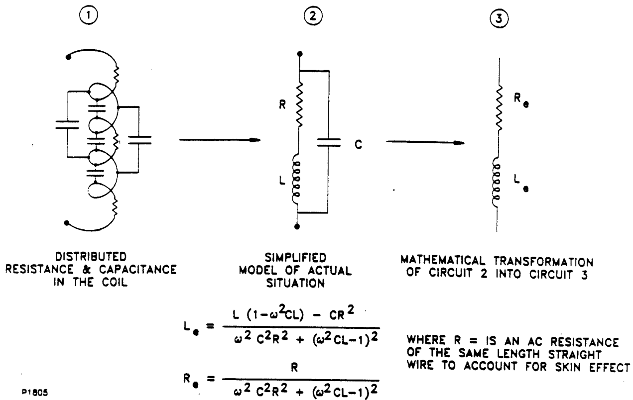
Figure 21 Schematic of Modeling of the Actual Coil
