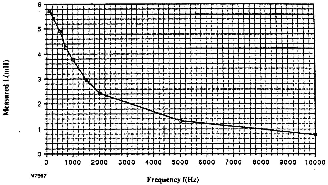
Figure 19 Self Inductance of the Secondary Coil As a Function of the Excitation Frequency
