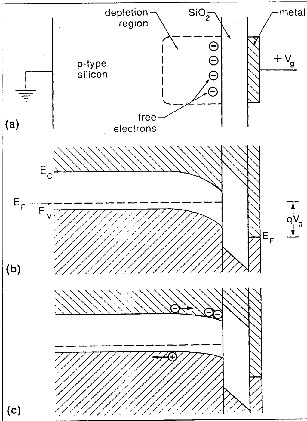
Figure 18: Charge collection at a single pixel of a CCD: (a) illustrates the collection of free charge carriers at the SiO 2 interface, (b) shows formation of a potential well after a voltage is applied, (c) shows collection of charge carriers in the potential well. From Reike (1994).
