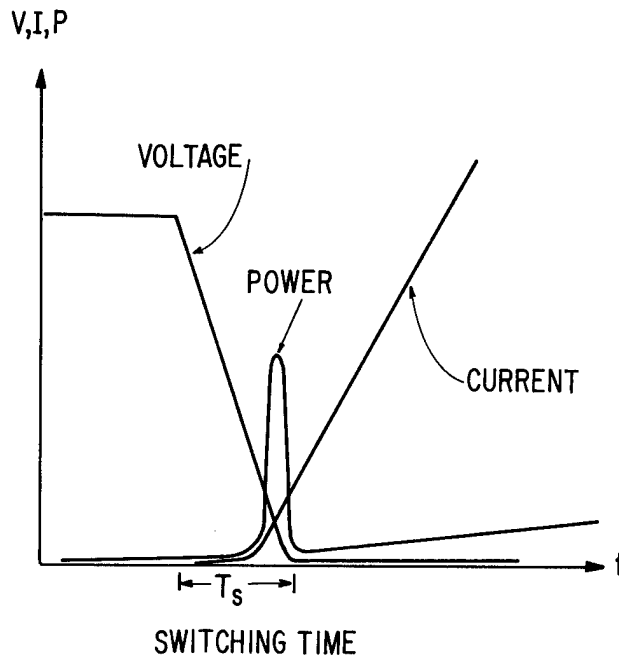
Fig. 10. Magnetic switch waveforms.
