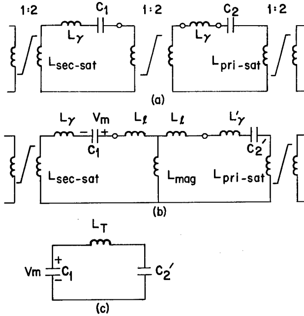
Fig. 13. Transformer resonant energy transfer schematic.
