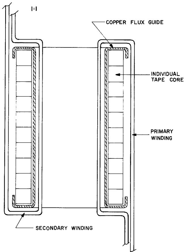
Fig. 17. Skin-effect flux-guide illustration.
