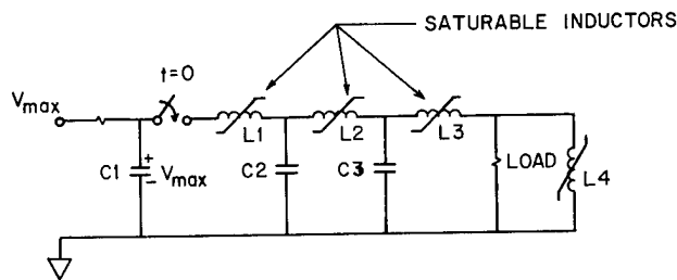
Fig. 3. Basic 3-stage series magnetic pulse compressor.
