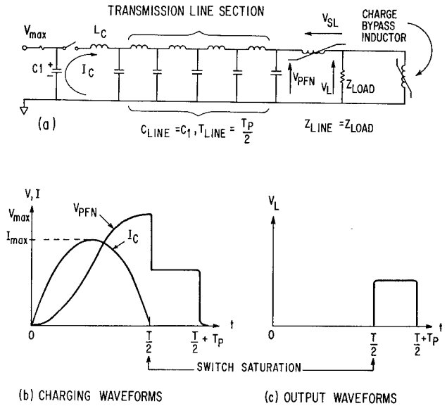
Fig. 8. Transmission line magnetic pulse compressor.
