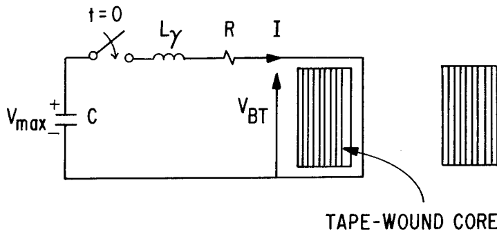
Fig. 18. Saturable inductor simulation circuit.
