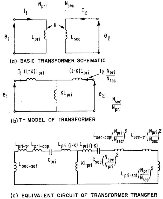
Fig. 14. Transformer equivalent circuits.
