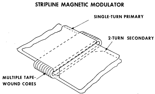
(a) BASIC 1:2 SATURABLE STRIPLINE TRANSFORMER
