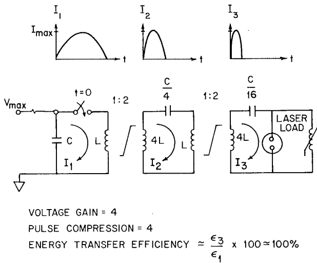
Fig. 7. Parallel magnetic compressor with voltage gain.
