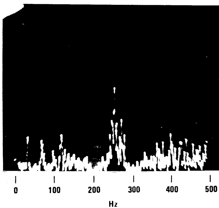
Figure 62. Phase Lock Tests Spectrum of E-0 Signal
