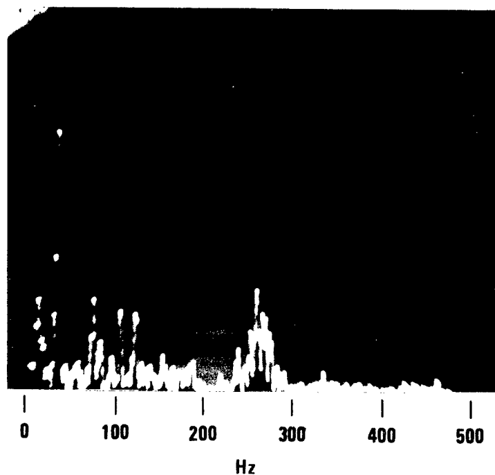
Figure 61. Phase Lock Tests Spectrum of HEL Mirror Signals
