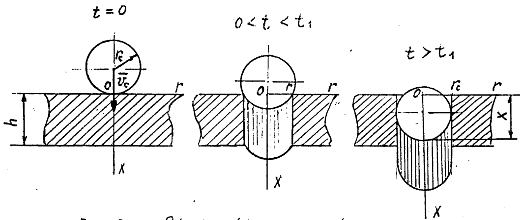
Fig. 3.1. Striker/barrier interaction
