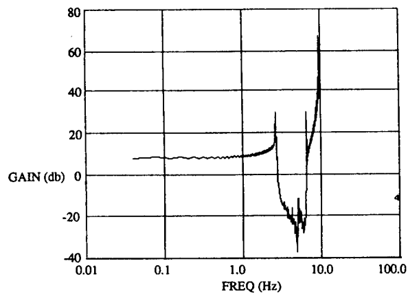
Fig. 3.3-10 Bode Plot of the Transfer Function Spectral Estimate h = P_{uy}/P_{uu} of the 3-6 Hz Narrowband Excitation Experiment.
