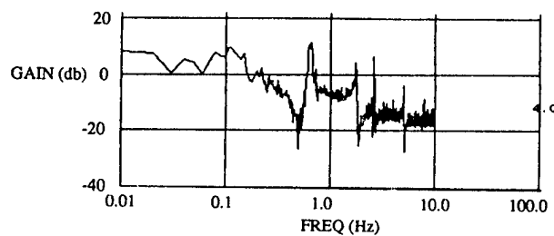
Fig. 3.2-37 Additive Uncertainty \Delta = P_{ee}/P_{uu} of the Identified Parametric Model for the 4-10 Axis Hub Actuator/Hub Sensor Wideband Excitation Case.
