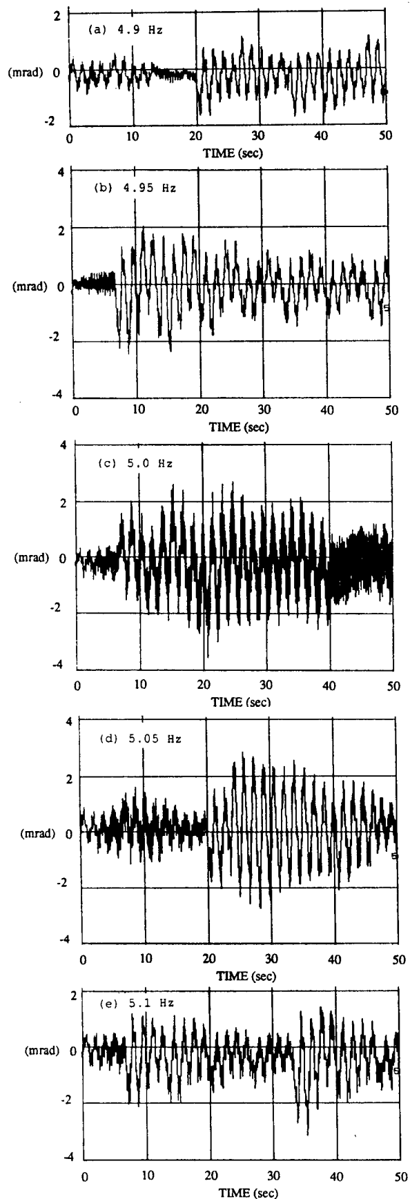
Fig. 3.3-24 Comparison of Output Responses at Sensor HS10 Subjected to Sinedwell Excitations of Frequencies (a) 4.9 Hz, (b) 4.95 Hz, (c) 5.0 Hz, (d) 5.05 Hz, and (e) 5.1 Hz at Actuator HA1.
