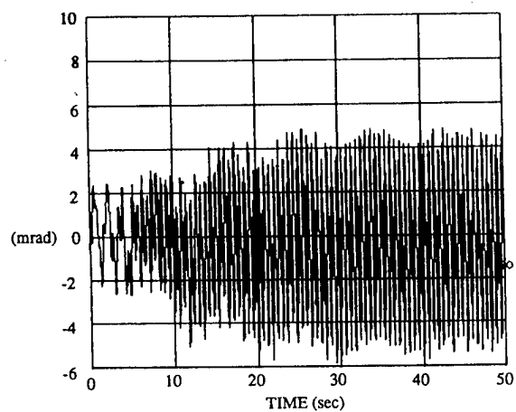
Fig. 3.3-17 Expanded View of Output Response at Sensor HS10 Subjected to 1.7 Hz Sinedwell Input Excitation at Actuator HA1.
