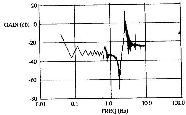
Fig. 3.3-9 Power Spectral Density P_{yy} of the 3-6 Hz Narrowband Excitation Output Response.
