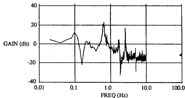
Fig. 3.5-14 Additive Uncertainty of the Identified Parametric Model for the Case of Input Parameters MSE=1024, NSE=8192, LSE=512, and NFFT=1024.
