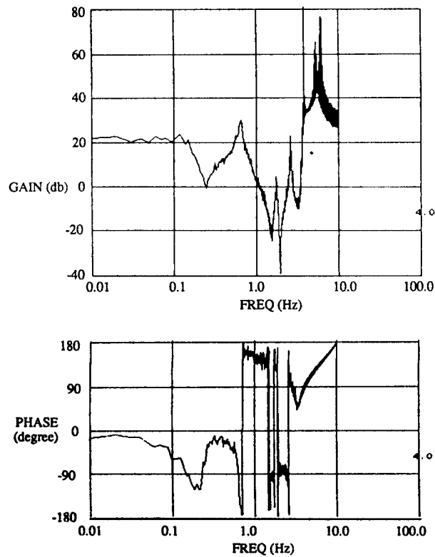
Fig. 3.2-53 Bode Plot of Transfer Function Spectral Estimate h = P_{uy}/P_{uu} for the 4-10 Axis Hub Actuator/Hub Sensor Narrowband (0-3 Hz) Excitation Case.
