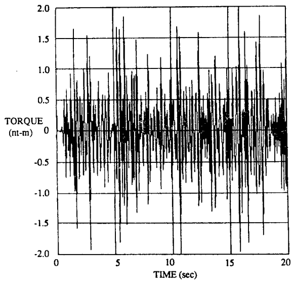
Fig. 3.3-6 Narrowband (3-6 Hz) Excitation Input.
