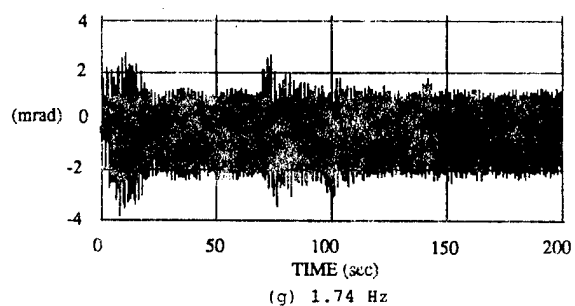
Fig. 3.3-18 Comparison of Output Responses at Sensor HS10 Subjected to Sinedwell Excitations of Frequencies (a) 1.66 Hz, (b) 1.68 Hz, (c) 1.69 Hz, (d) 1.70 Hz, (e) 1.71 Hz, (f) 1.72 Hz, and (g) 1.74 Hz at Actuator HA1.
