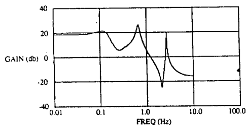
Fig. 3.2-16 Curve Fit Computation Sequence of Assumed Modal Order 3 for the 1-7 Axis Hub Actuator/Hub Sensor Wideband Excitation Case.
