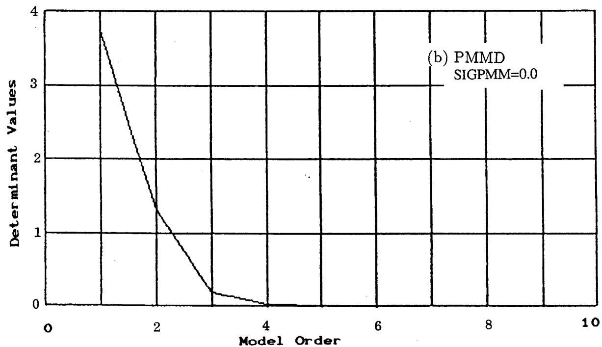
Fig. 2.7-10 The PMM Determinant Tests Using Wide-Band Data (a) PMMDE, (b) PMMD, SIGPMM=0.0.
