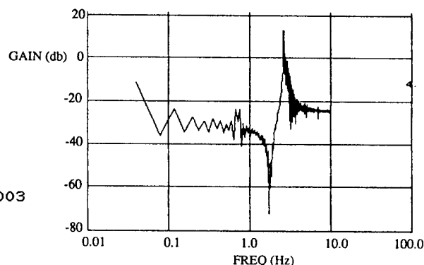
Fig. 3.3-13 Power Spectral Density P_{ee} of the Output Error of the 4.8-5.2 Hz Selected Range Curve Fitted Model.
