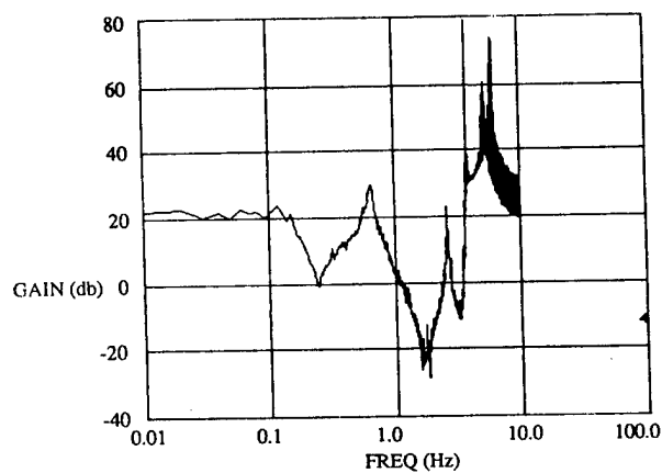
Fig. 3.3-5 Additive Uncertainty P_{ue}/P_{uu} of the 1.65-1.75 Hz Selected Range Curve Fitted Model.
