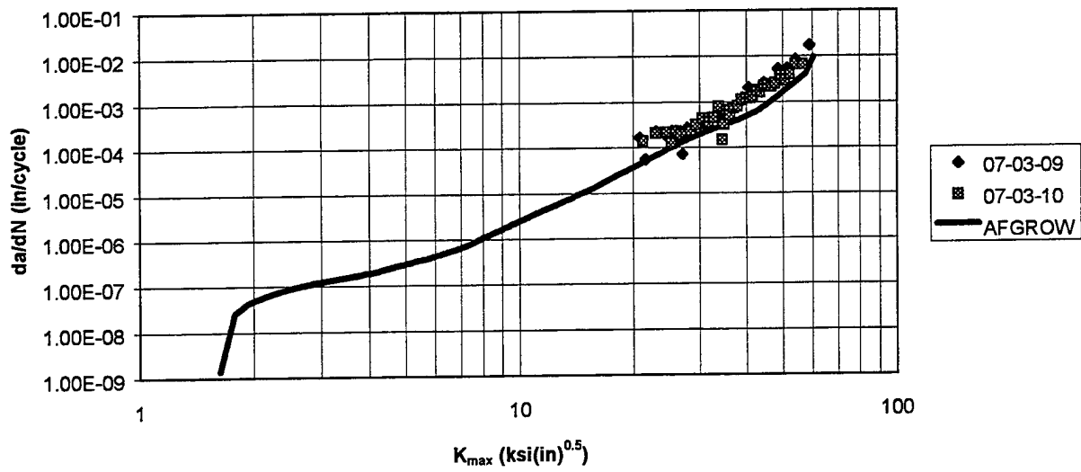
Figure 37: da/dN vs. Kmax data and AFGROW curve for Pmax = 38.6 kips, R=-1.
