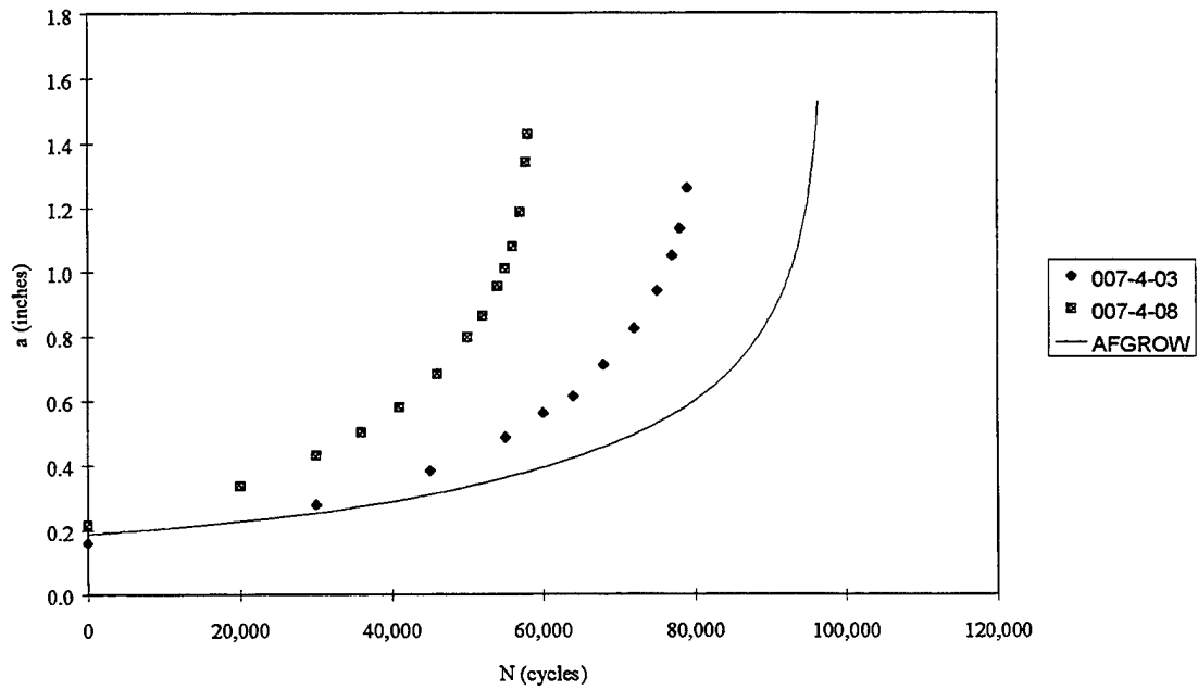
Figure 42: Crack growth plot for 1.5x underload spectrum with AFGROW prediction.
