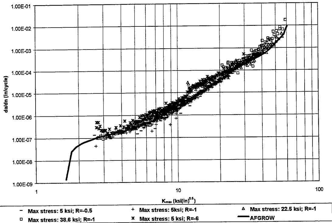
Figure 38: da/dN vs. Kmax data and AFGROW curve for all specimens. (Each data set represents two specimens)
