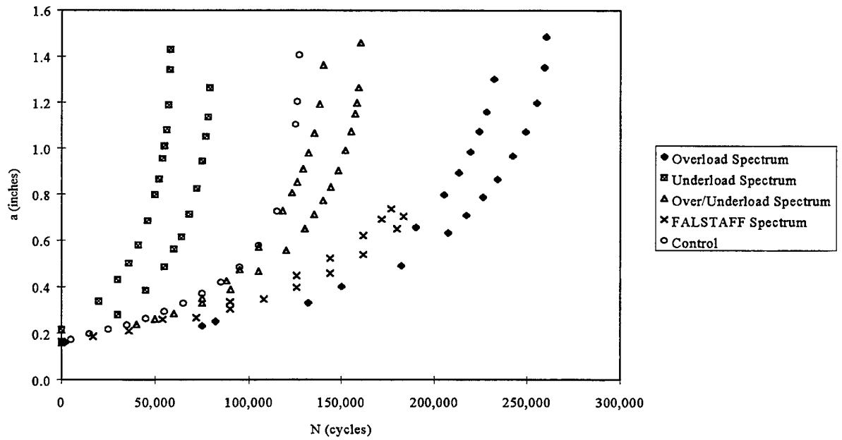
Figure 45: Composite plot of all load sequence specimens. (with the constant amplitude control specimen included)
