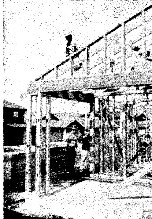
Figure B.22: New construction, central Oahu; fall protection plan; truss installation--walking the top plate
