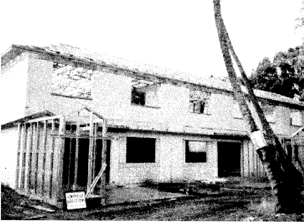
Figure B.9: Renovation project, Hickam Air Force Base; fall protection plan (Note "controlled access zone" sign at left front corner of structure.)
