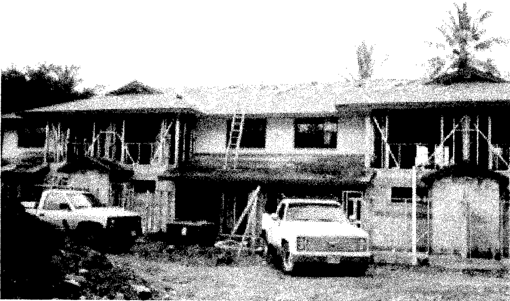
Figure B.10: Renovation project, Hickam Air Force Base; fall protection plan (Note access to roof.)
