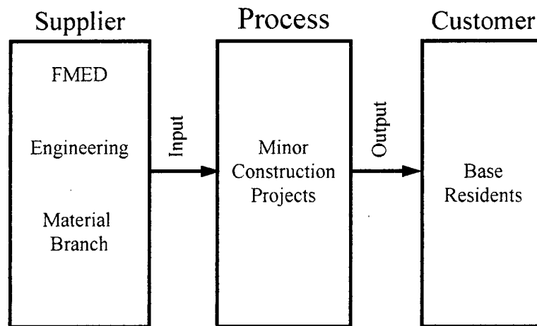
Figure 1 - SIPOC Diagram
