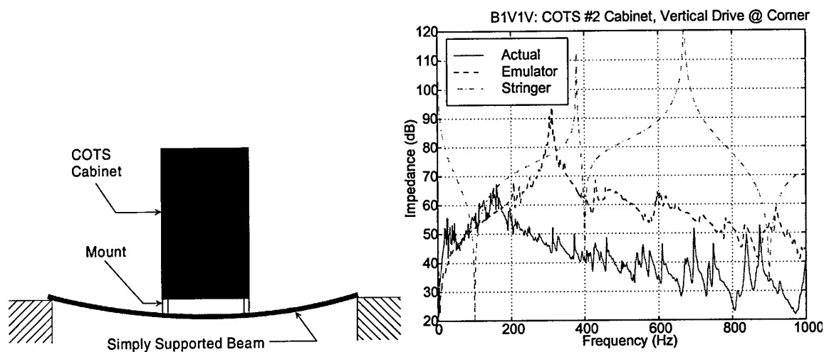
FIGURE 2. Vertical drive point impedance of cabinet, emulator and stringer (beam).
