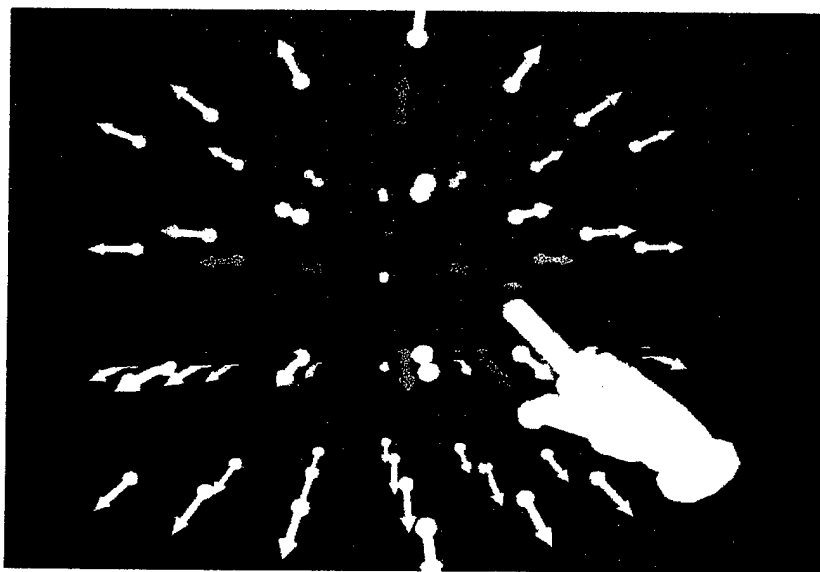
Figure 2. MaxwellWorld
