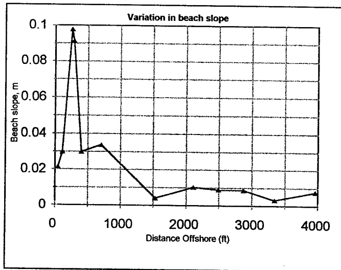
Figure 31. Variation in beach slope with distance offshore
