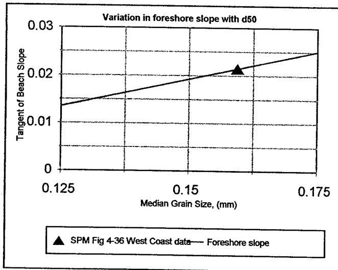
Figure 33. Median grain size versus foreshore slope comparison with SPM data
