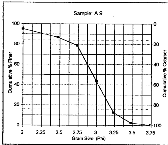
Figure 27. Sediment Distribution: Sample A-9
