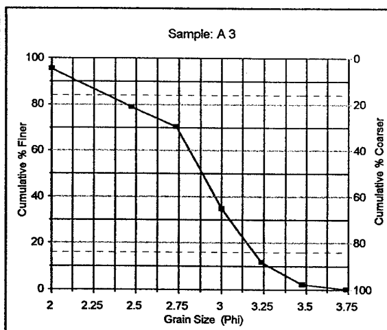
Figure 21. Sediment Distribution: Sample A-3
