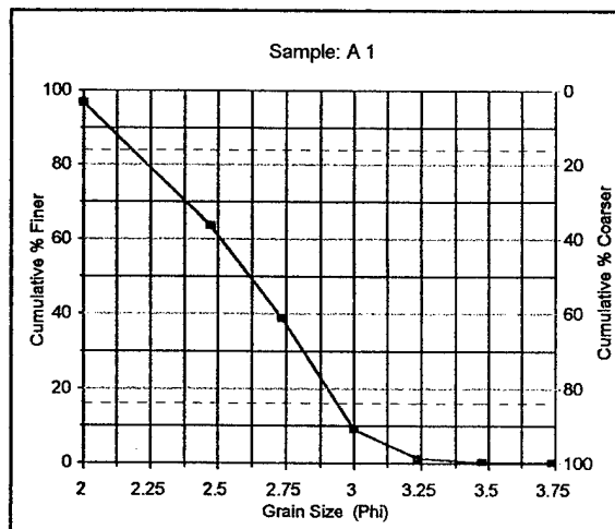
Figure 19. Sediment Distribution: Sample A-1
