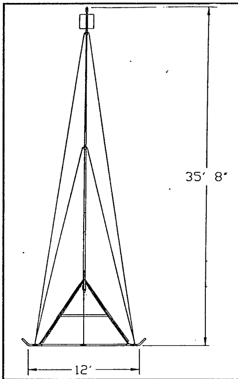
Figure 4. Diagram of basic sled dimensions.
