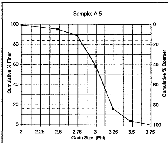
Figure 23. Sediment Distribution: Sample A-5
