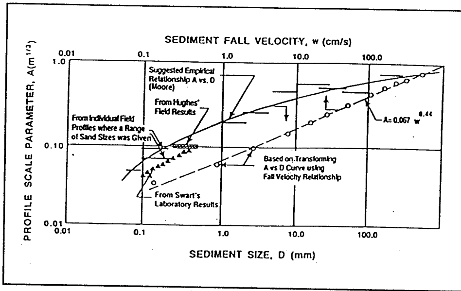
Figure 6. Profile Scale Factor, A versus Sediment Diameter, d , and Fall Velocity, w (Dean, 1987; adapted in part from Moore, 1982)
