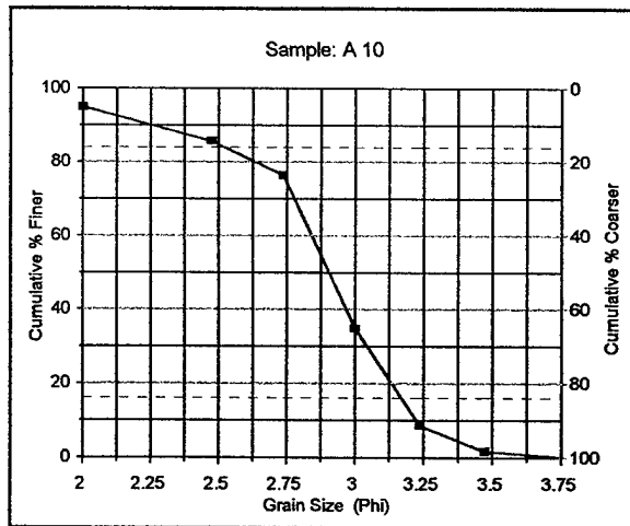
Figure 28. Sediment Distribution: Sample A-10
