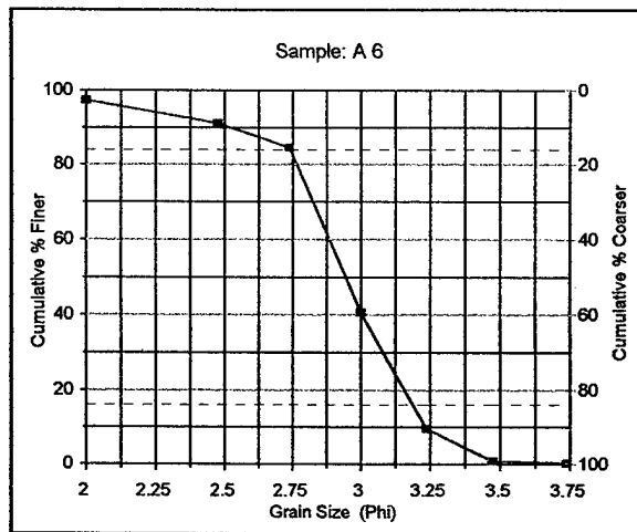
Figure 24. Sediment Distribution: Sample A-6
