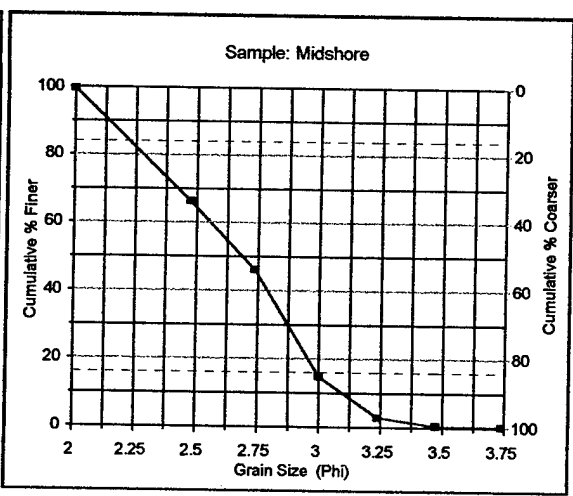
Figure 17. Sediment Distribution: Sample Midshore
