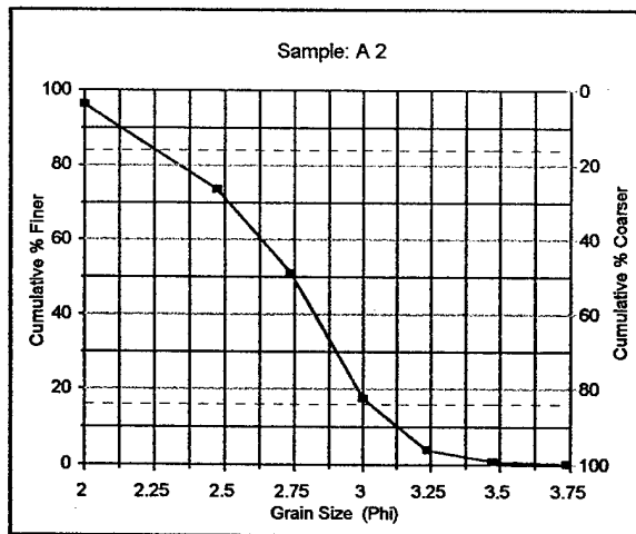
Figure 20. Sediment Distribution: Sample A-2
