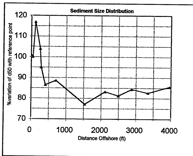
Figure 29. Distance offshore versus percent variation of d_{50} from reference diameter
