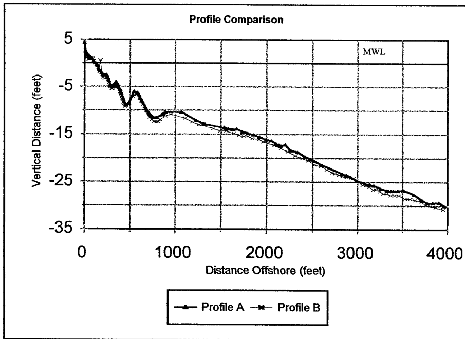
Figure 14. Measured beach profile comparison.
