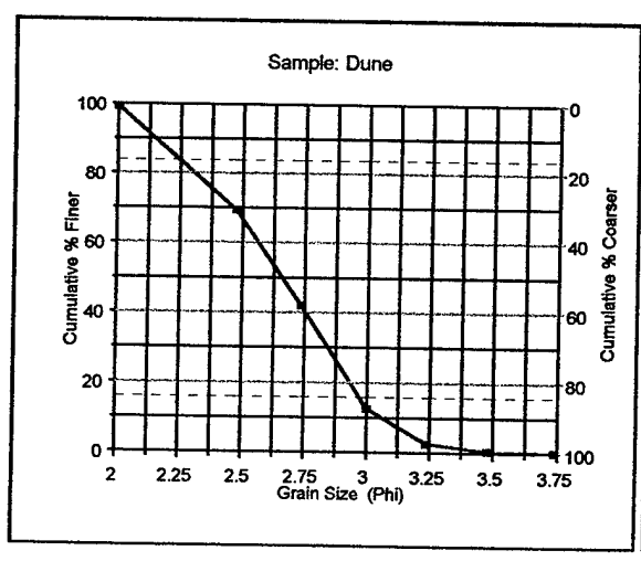
Figure 16. Sediment Distribution: Sample Dune
