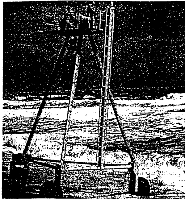
Figure 3. Coastal Research Amphibious Buggy (Birkemeier & Mason, 1984)
