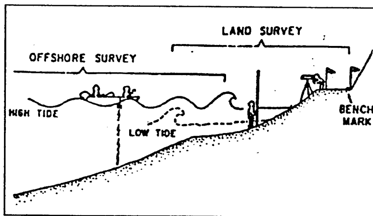
Figure 2. Beach Profile Survey Technique (Dean & Dalrymple, 1996, from Nordstrom and Inman, 1975)
