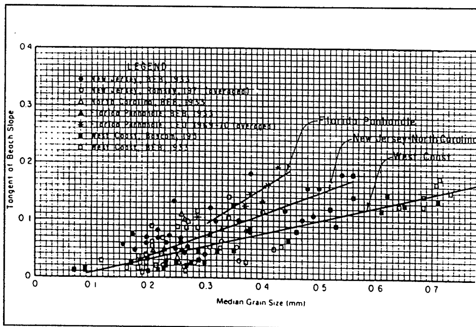
Figure 34. Median Grain size versus foreshore slope (SPM, 1984)
