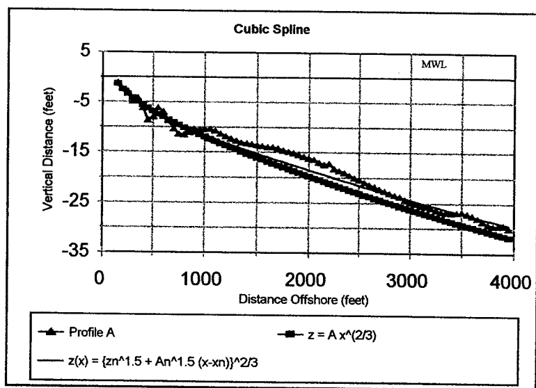
Figure 36. Cubic spline used to calculate percent error of profile predictions
