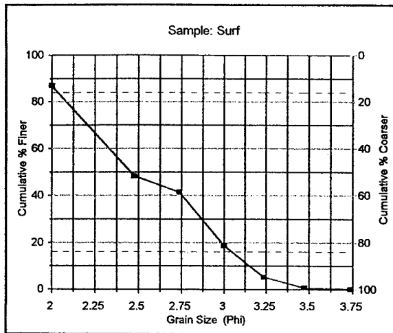
Figure 18. Sediment Distribution: Sample Surf Zone
