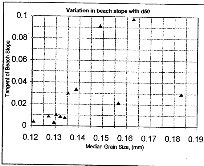
Figure 32. Variation of beach slope with median grain size
