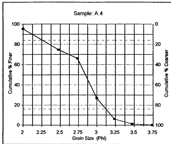
Figure 22. Sediment Distribution: Sample A-4
