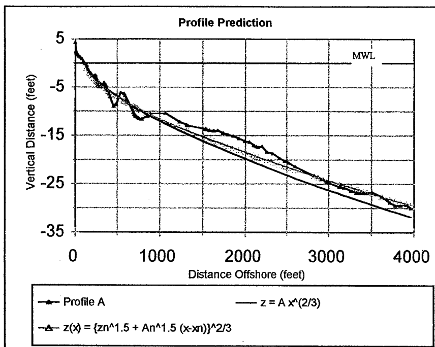
Figure 35. Predicted Profile Comparison
