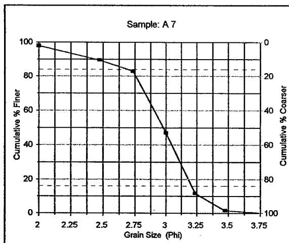
Figure 25. Sediment Distribution: Sample A-7
