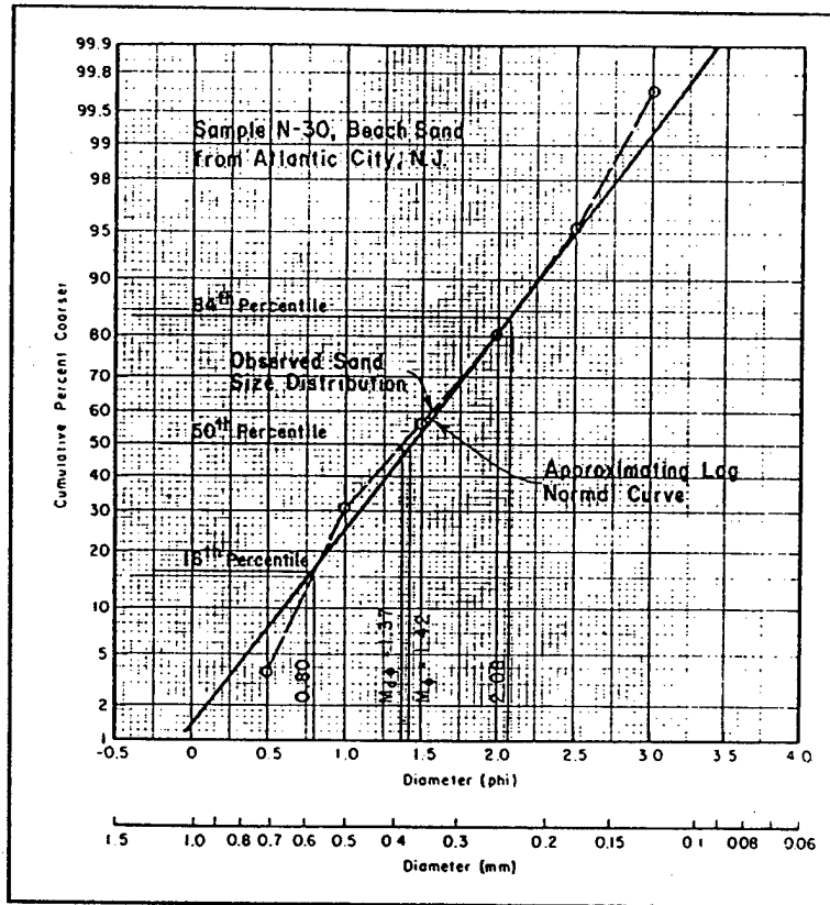
Figure 7. Example size distribution (Shore protection Manual, 1984)
