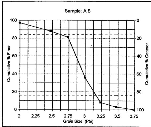
Figure 26. Sediment Distribution: Sample A-8
