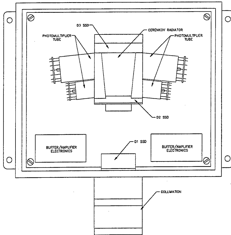
Figure 7 Breadboard Detector Assembly.
