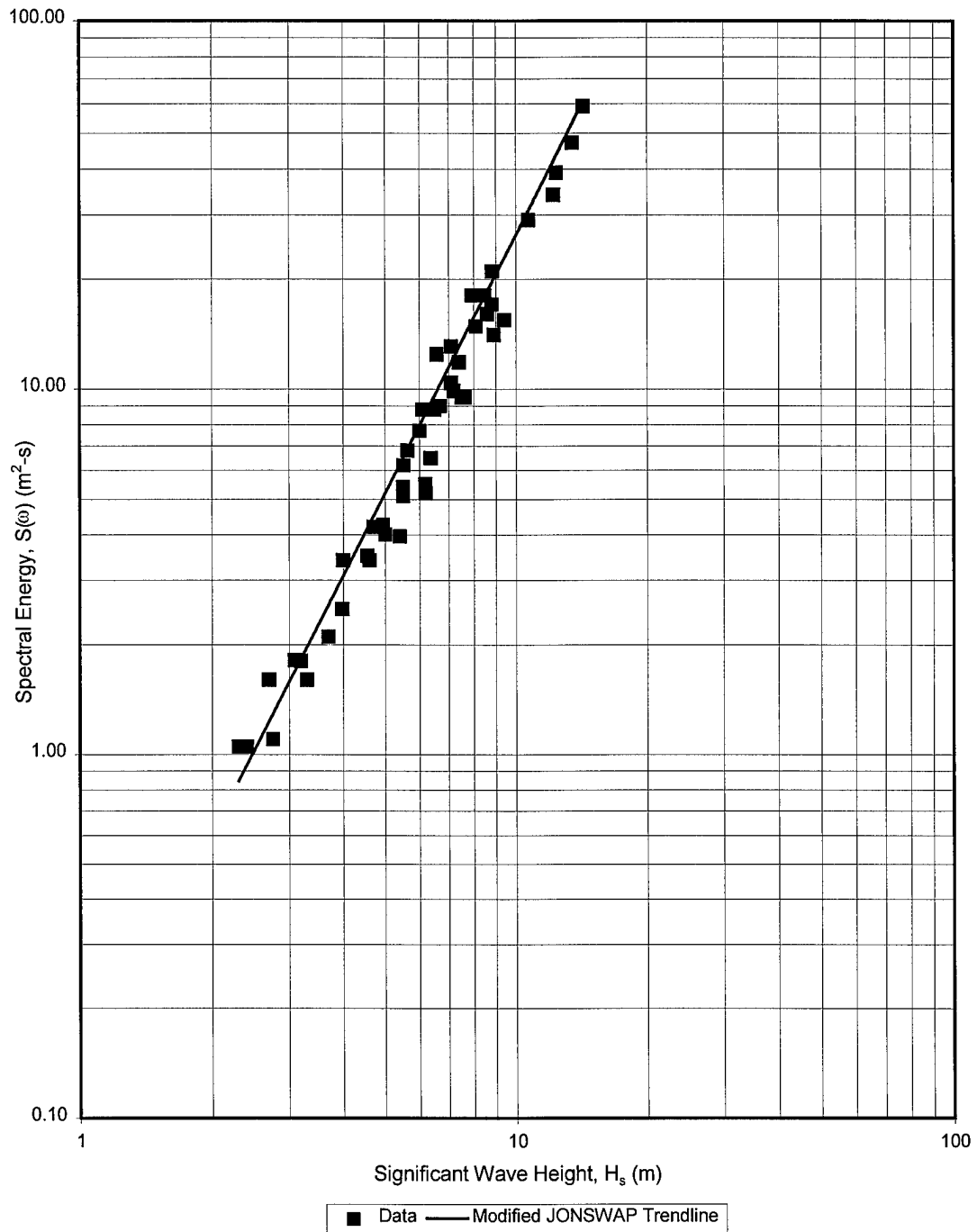
Figure 6 Modified JONSWAP spectrum versus significant wave height for \omega/\omega_m=1.00
