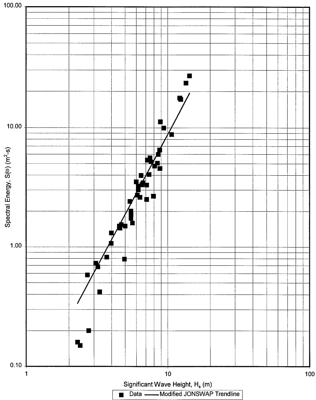
Figure 2 Modified JONSWAP spectrum versus significant wave height for \omega/\omega_m=0.80
