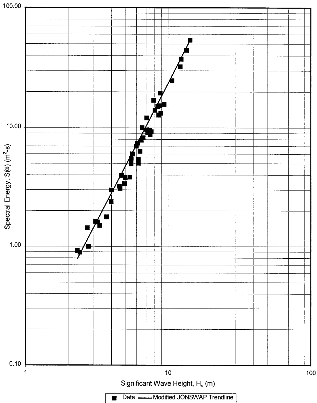
Figure 7 Modified JONSWAP spectrum versus significant wave height for \omega/\omega_m=1.05
