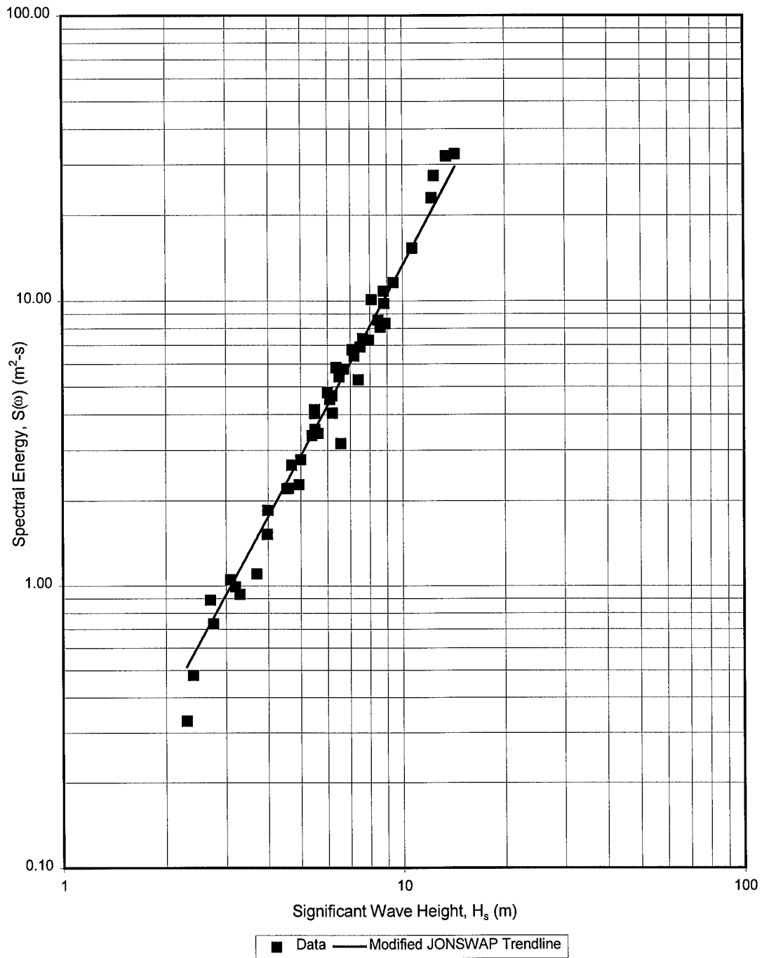
Figure 10 Modified JONSWAP spectrum versus significant wave height for \omega/\omega_m=1.20
