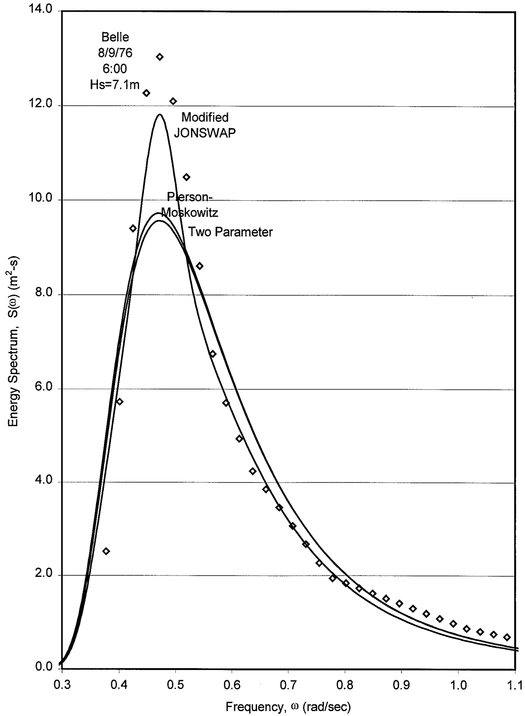
Figure 36 Comparison between Modified JONSWAP and measured spectrum for Hurricane Belle, H_s=7.1 m
