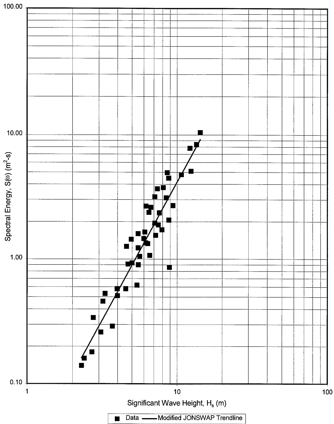
Figure 19 Modified JONSWAP spectrum versus significant wave height for \omega/\omega_m=1.65
