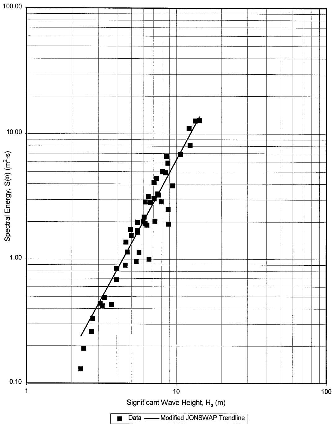
Figure 16 Modified JONSWAP spectrum versus significant wave height for \omega/\omega_m=1.50
