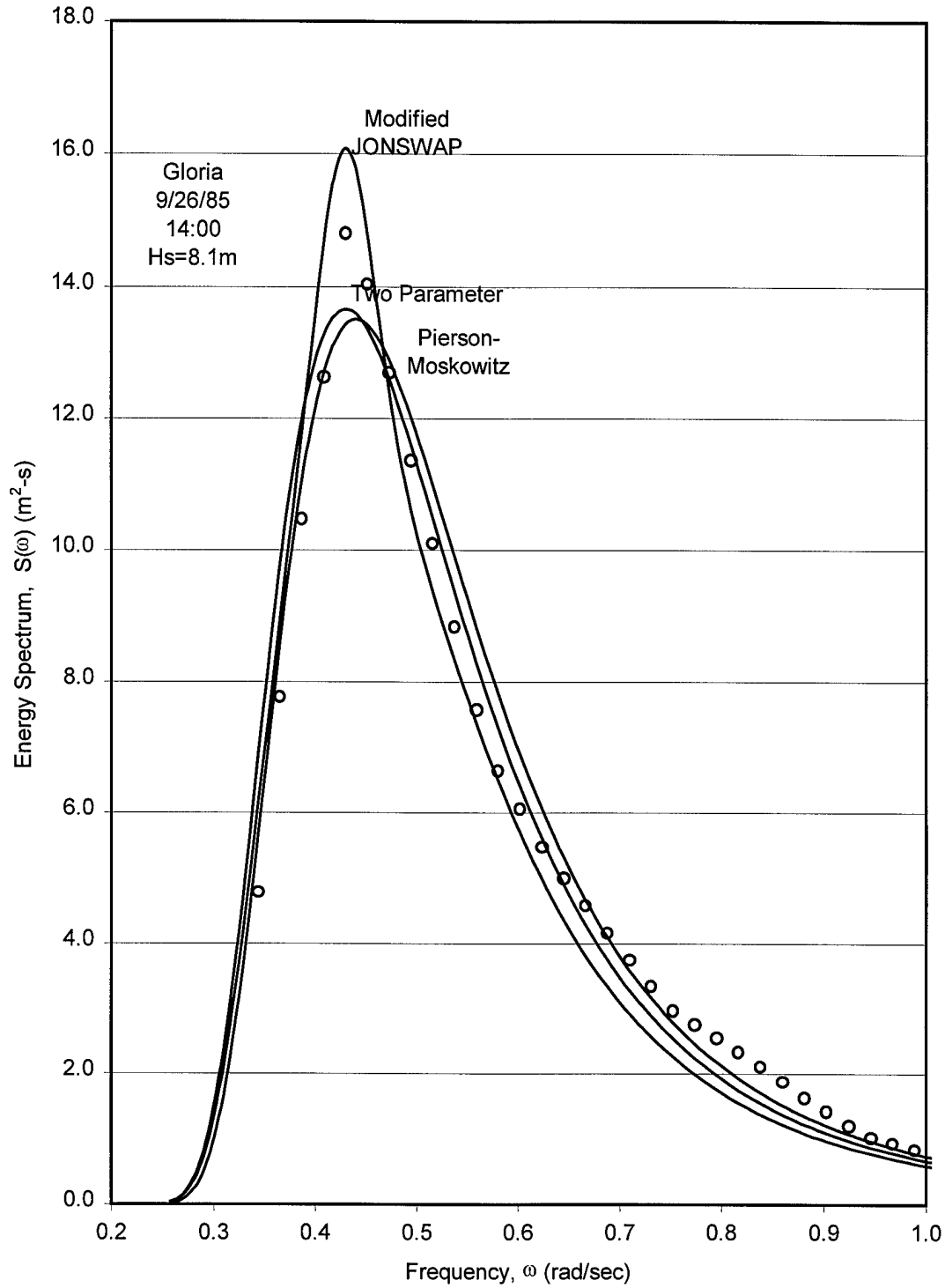
Figure 38 Comparison between Modified JONSWAP and measured spectrum for Hurricane Gloria, H_s=8.1\text{ m}
