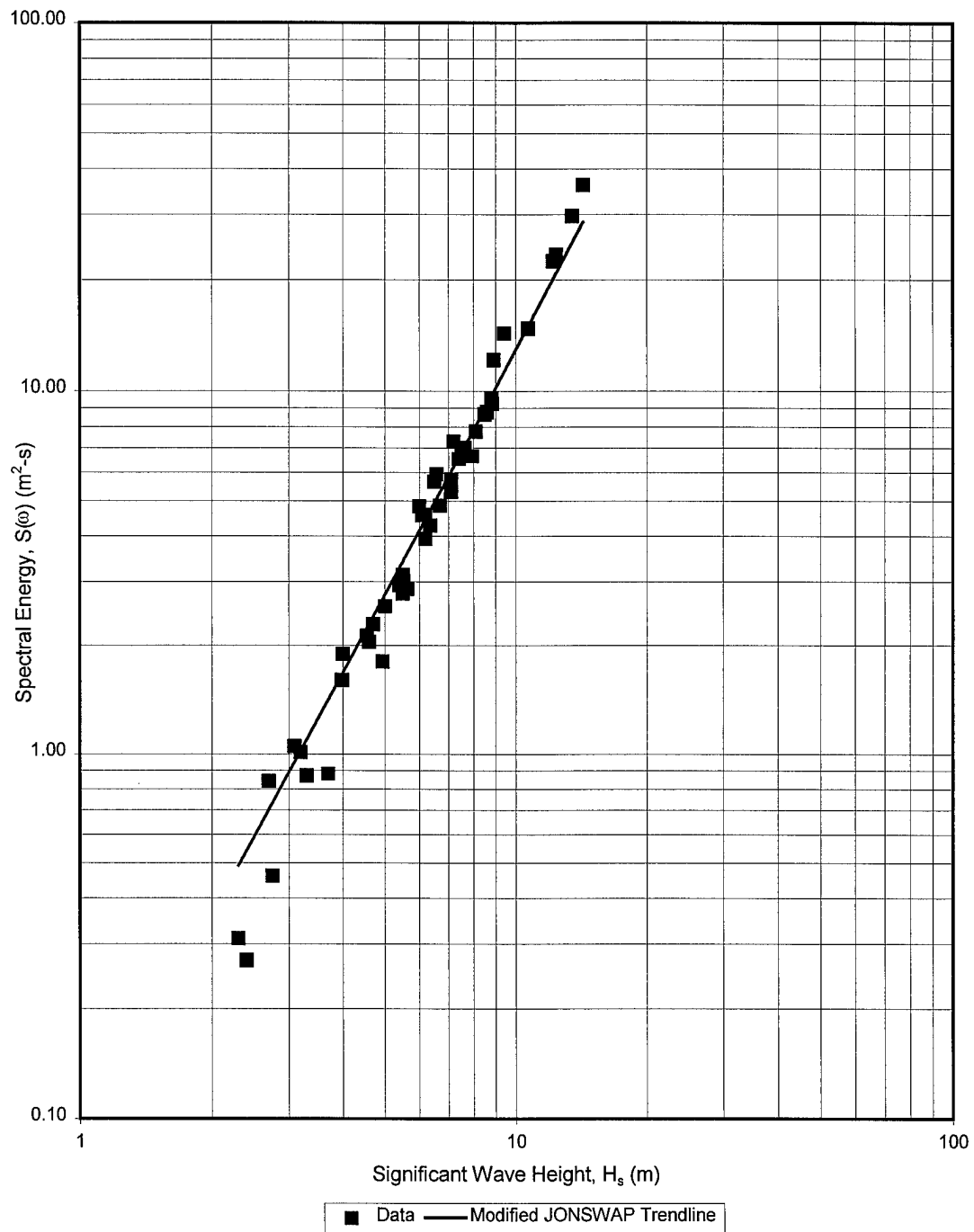
Figure 3 Modified JONSWAP spectrum versus significant wave height for \omega/\omega_m=0.85
