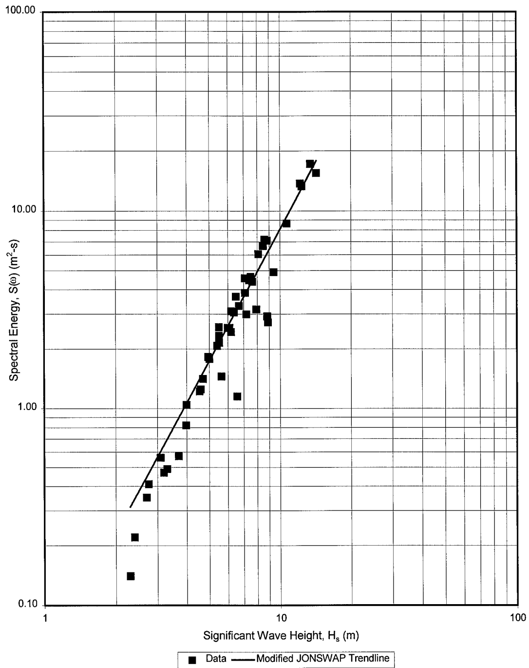
Figure 14 Modified JONSWAP spectrum versus significant wave height for \omega/\omega_m=1.40
