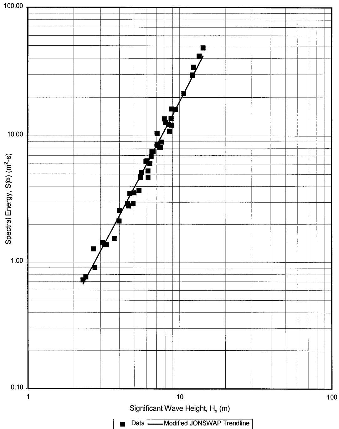
Figure 8 Modified JONSWAP spectrum versus significant wave height for \omega/\omega_m=1.10
