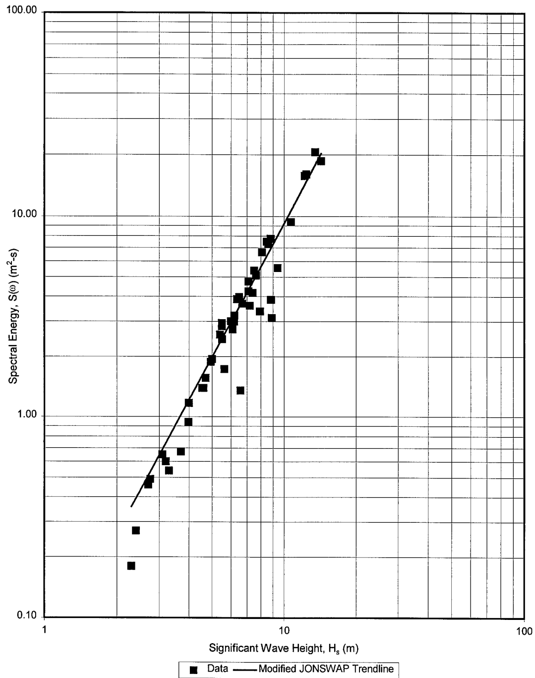
Figure 13 Modified JONSWAP spectrum versus significant wave height for \omega/\omega_m=1.35
