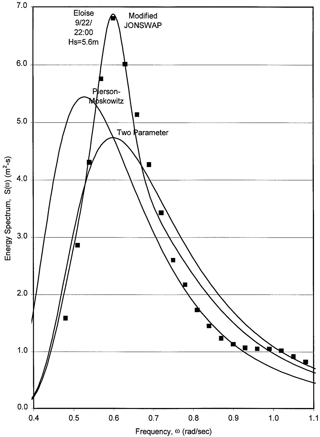
Figure 39 Comparison between Modified JONSWAP and measured spectrum for Hurricane Eloise, H_s=5.6\text{ m}
