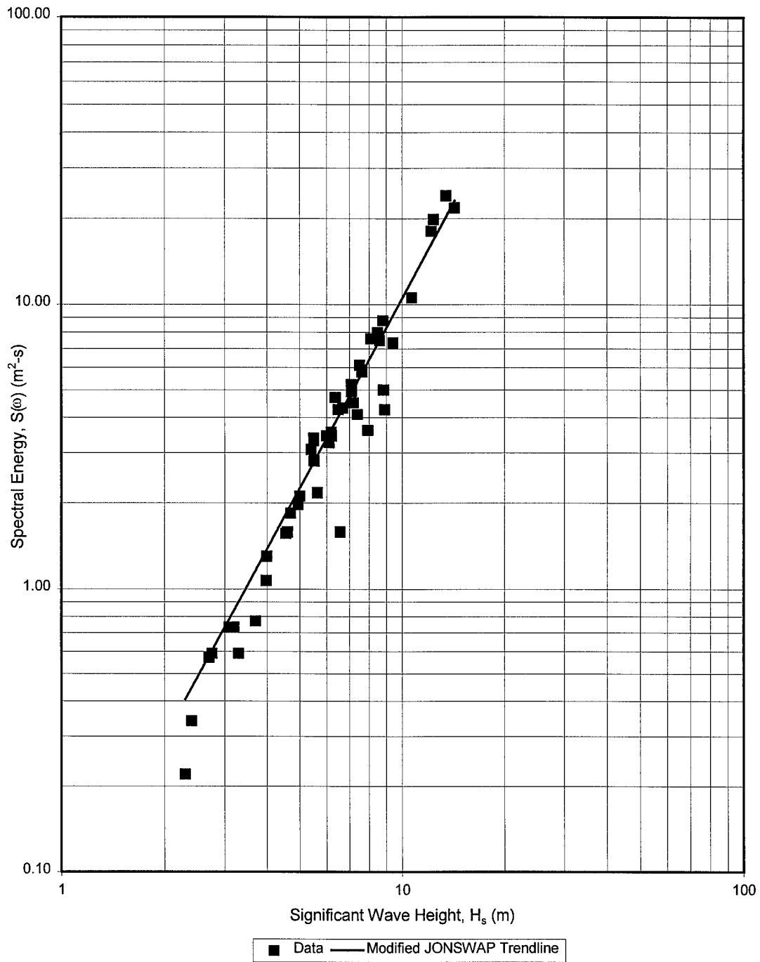
Figure 12 Modified JONSWAP spectrum versus significant wave height for \omega/\omega_m=1.30
