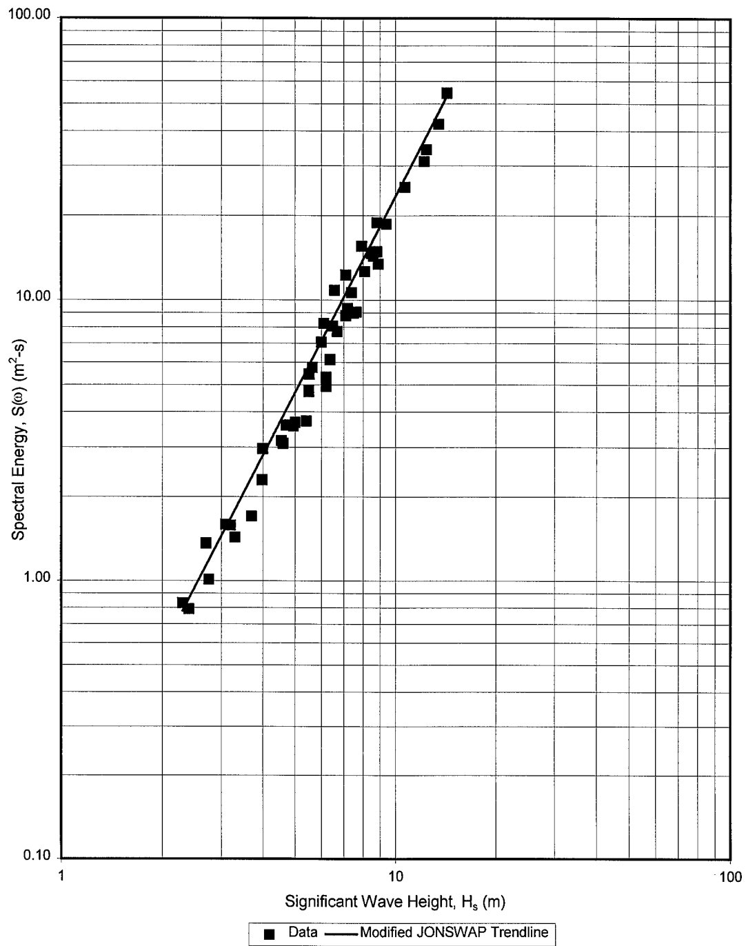
Figure 5 Modified JONSWAP spectrum versus significant wave height for \omega/\omega_m=0.95
