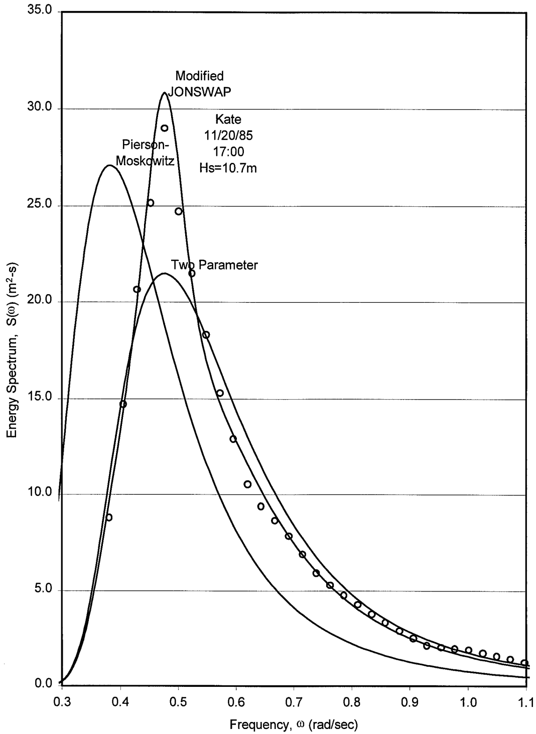
Figure 44 Comparison between Modified JONSWAP and measured spectrum for Hurricane Kate, H_s=10.7\text{ m}
