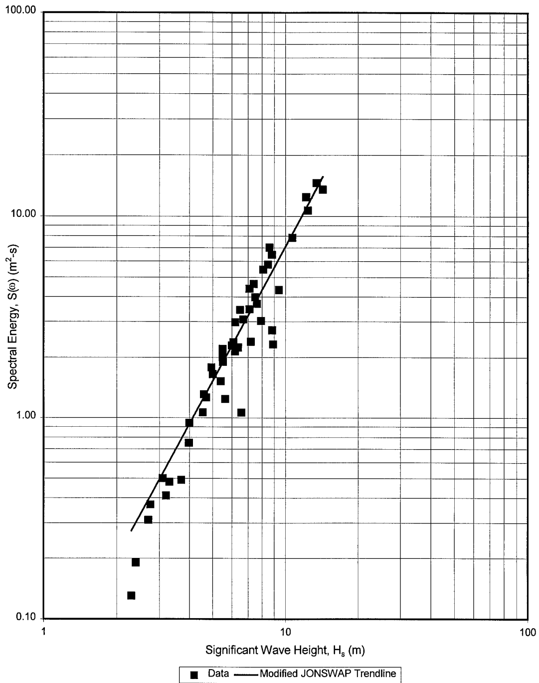
Figure 15 Modified JONSWAP spectrum versus significant wave height for \omega/\omega_m=1.45
