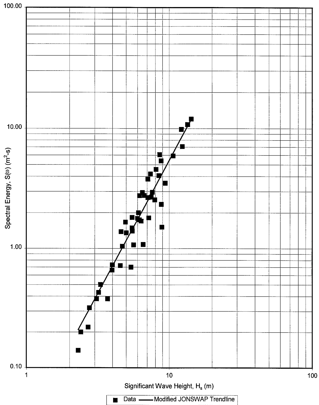
Figure 17 Modified JONSWAP spectrum versus significant wave height for \omega/\omega_m=1.55
