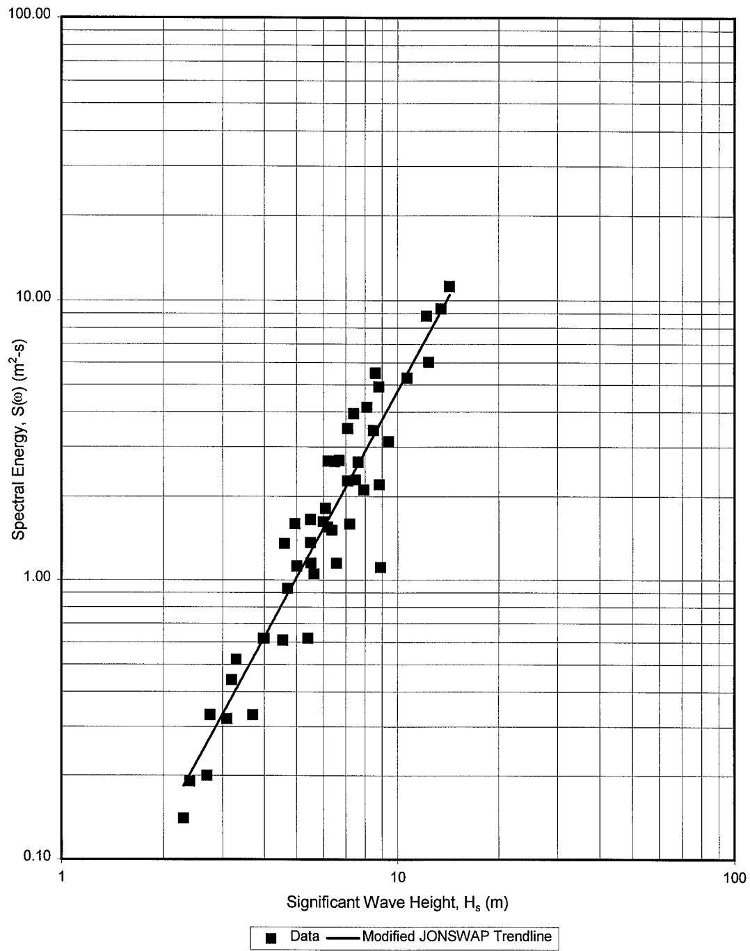
Figure 18 Modified JONSWAP spectrum versus significant wave height for \omega/\omega_m=1.60
