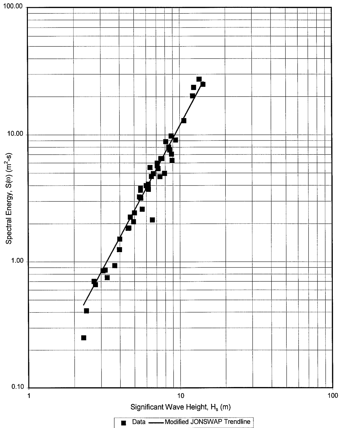
Figure 11 Modified JONSWAP spectrum versus significant wave height for \omega/\omega_m=1.25
