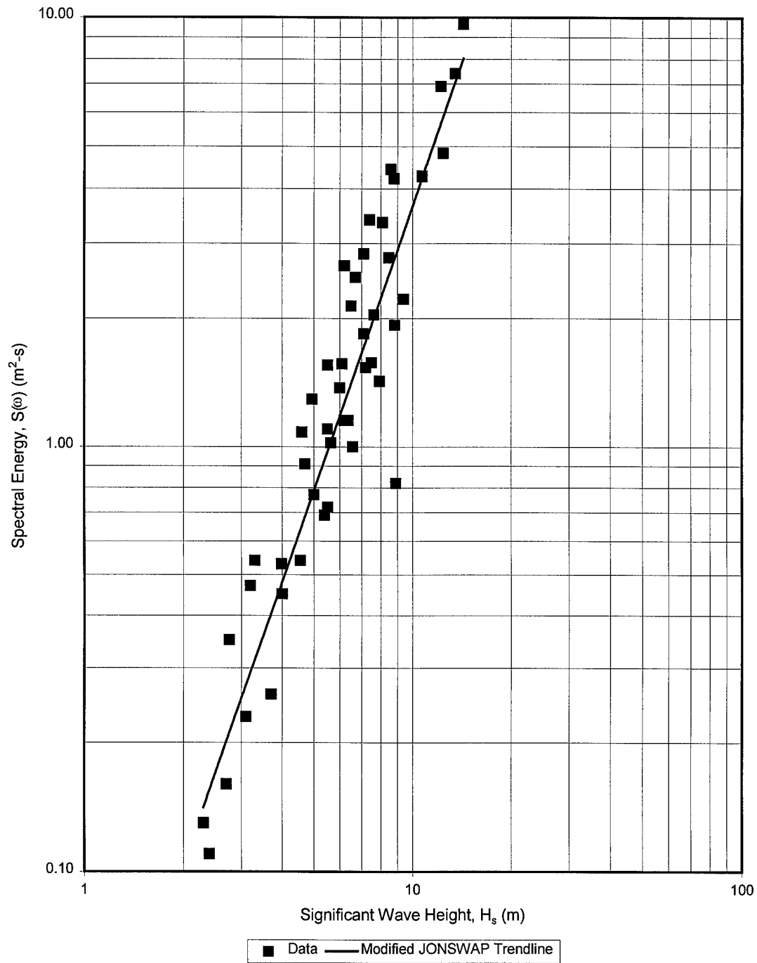
Figure 20 Modified JONSWAP spectrum versus significant wave height for \omega/\omega_m=1.70
