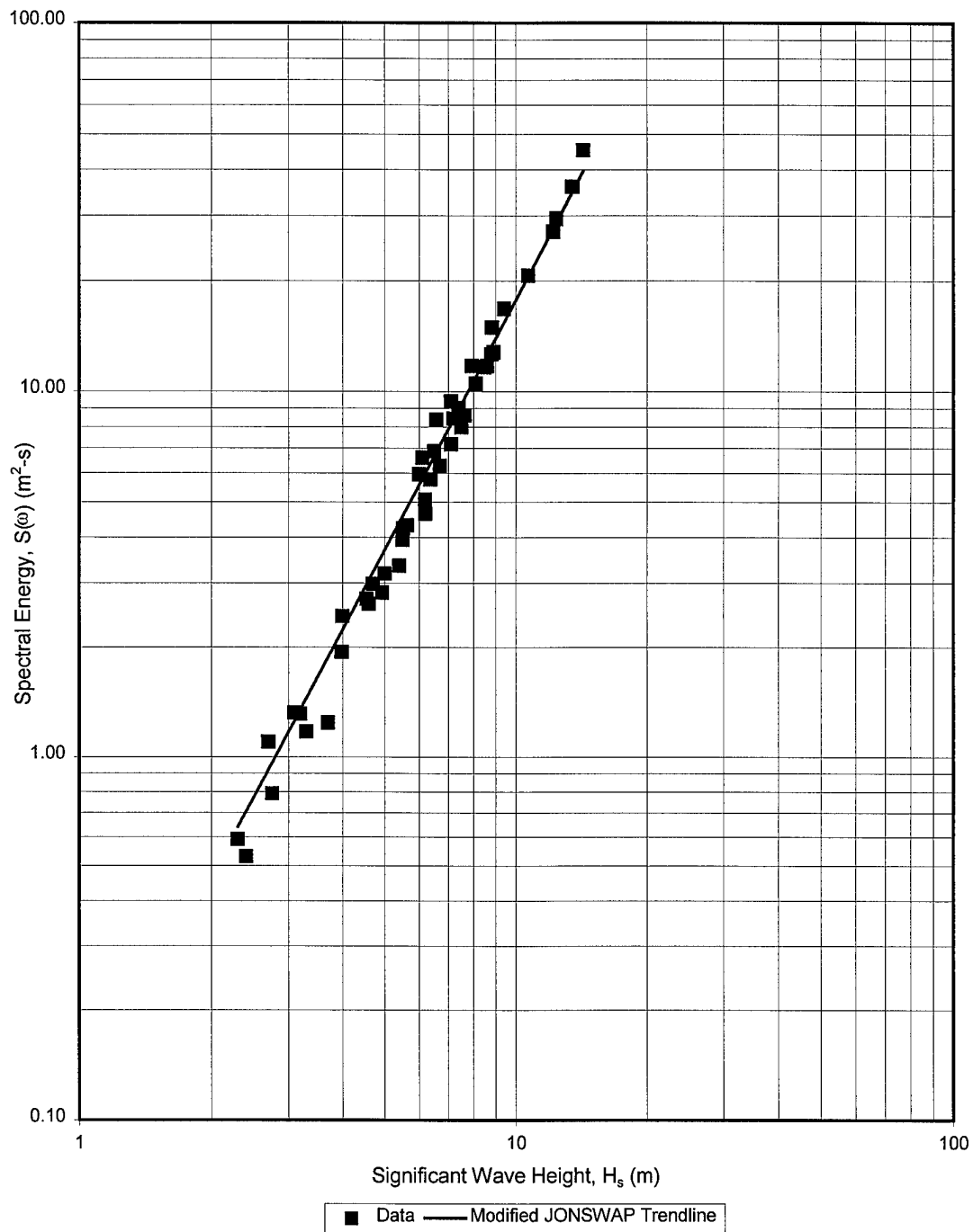
Figure 4 Modified JONSWAP spectrum versus significant wave height for \omega/\omega_m=0.90
