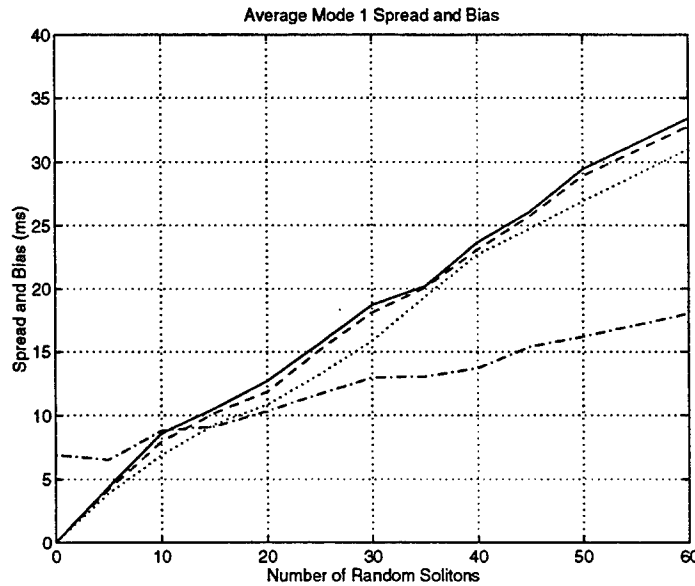
Figure 5-7: The average mean (-), median (- -), and peak ( \cdots ) lag with respect to the pseudo-adiabatic arrival, and standard deviation ( -\cdot- ) of scattered mode 1 arrivals plotted as a function of the number of solitons placed between the source and the receiver, where the solitons are added starting from the source end. The upper three lines are all bias measures, and the lower line is a measure of spread.
