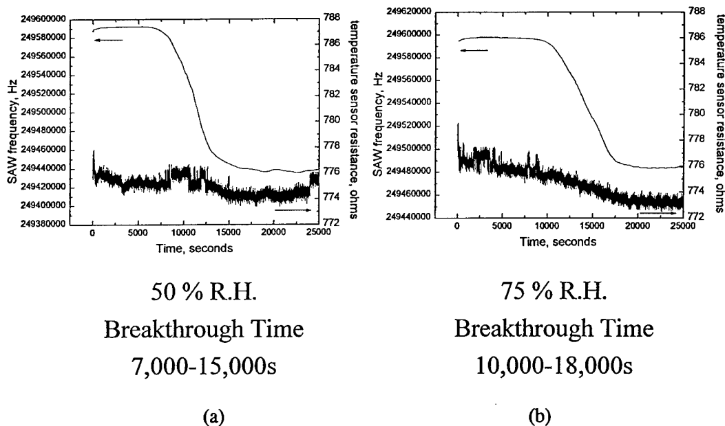
Fig. 3 – DMMP breakthrough curves on initially dry carbon with the % relative humidity of the air carrier gas varied as follows: (a) air at 50% R.H. and (b) air at 75% R.H. The SAW sensor was embedded in the carbon adsorbent at the test bed exit in these experiments. The top curves are the frequency responses of the coated SAW. The bottom curves are the resistances of the temperature sensors
