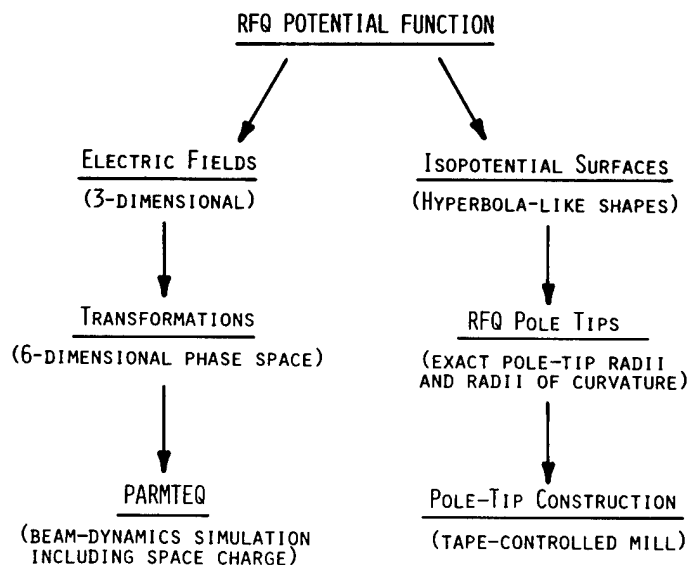
Fig. 56. Beam-dynamics simulation and pole-tip geometry.
