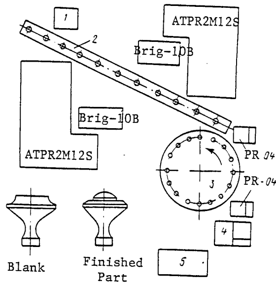
Figure 5. Automatic Pushbutton Processing Line
