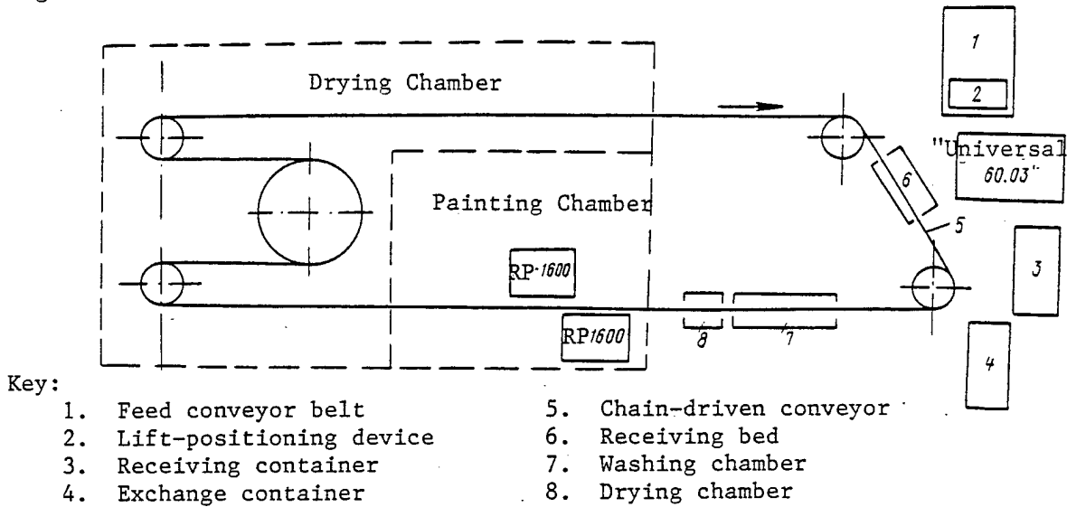
Figure 6. Automatic Panel Painting Line
