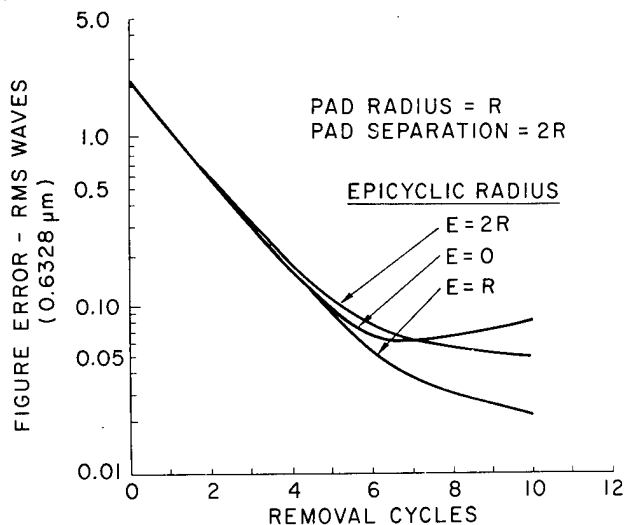
Fig. 6. Modeled figure process for several epicyclic motion tools.
