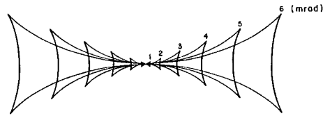
Figure 2. Effect of Tilt on the Spot Diagram of a Perfect Cone
