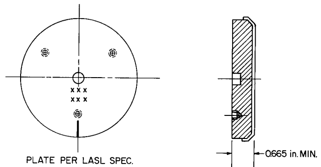
Fig. 9. Substrate plating.
