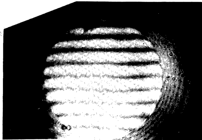
Fig. 10. Interferogram of 10" diam. F/2 sphere.
