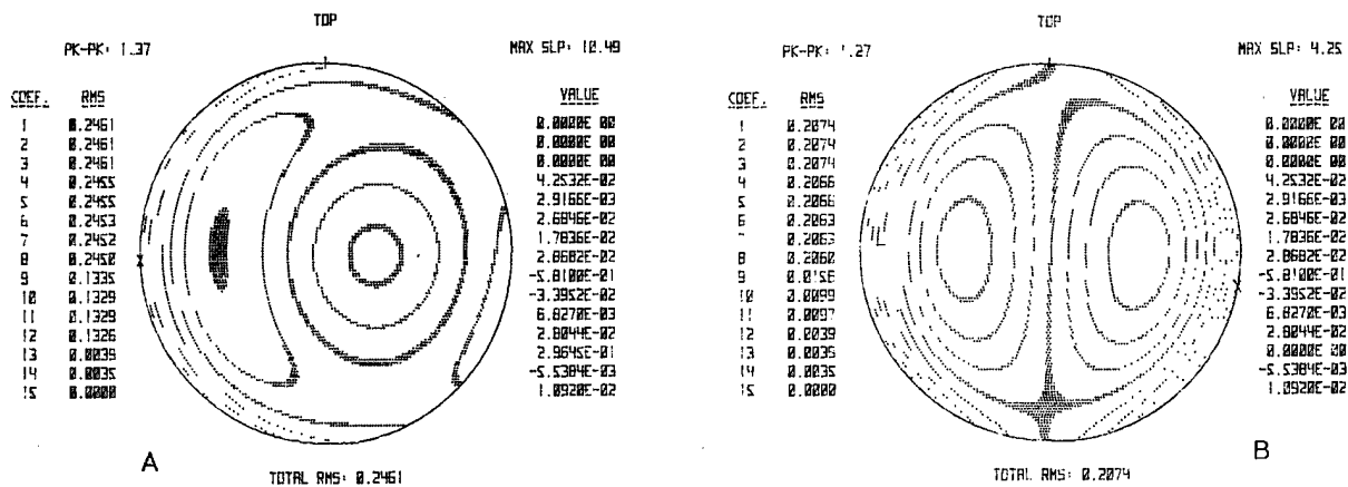
Fig. 4. Plots of a Real Interferogram with some Zernike Polynomial Coefficients set Equal to Zero. The contour interval in Plot A is 0.2 fringe, and in Plot B, 0.1 fringe.
