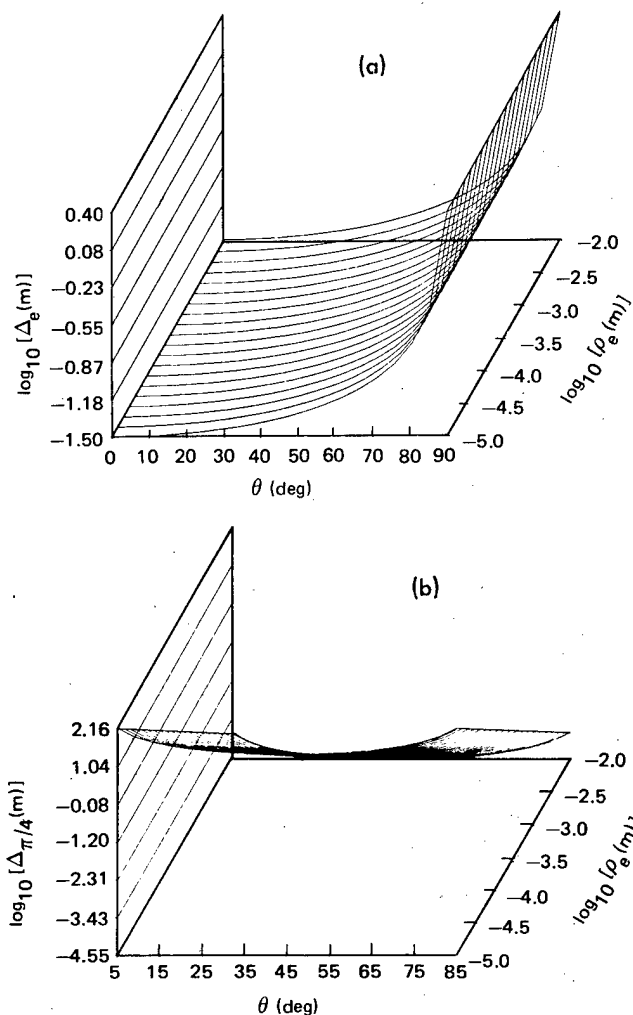
FIG. 4. Calculated values of the amplitude (a) and phase (b) coherence lengths as functions of the propagation angle ( \theta^+ ) and source coherence length ( \rho_e ). Fixed parameters are \lambda = 10^{-5} m, C_n^2 = 10^{-15} m ^{-2/3} , L = 10^{-1} m, and R^+ = 10^3 m.
