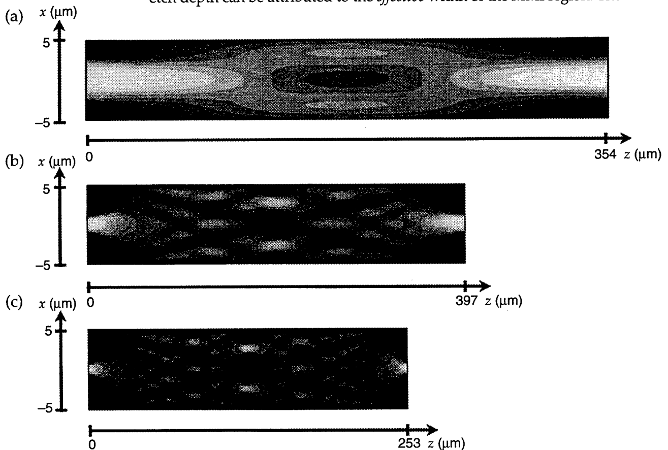
Figure 4. Top view of MMI region showing a gray-scale plot of TE field. (a) Etch depth 0.52\ \mu\text{m} ; only 3 lateral modes supported in MMI region. (b) Etch depth 0.82\ \mu\text{m} (transverse mode is at cutoff); 10 lateral modes supported in MMI region. (c) Semi-infinite etch depth assumed (i.e., lateral mode index surrounding MMI region and input/output rib waveguides is unity); 49 lateral modes supported in MMI region.
