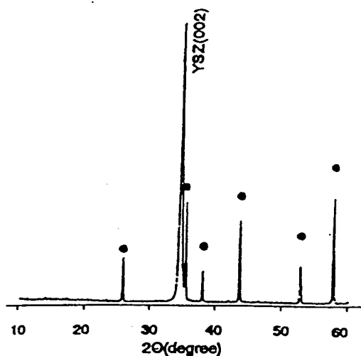
Fig. 1. X-ray diffraction \theta - 2\theta scan of YSZ on \text{Al}_2\text{O}_3 ( \bullet \text{Al}_2\text{O}_3 peak)
