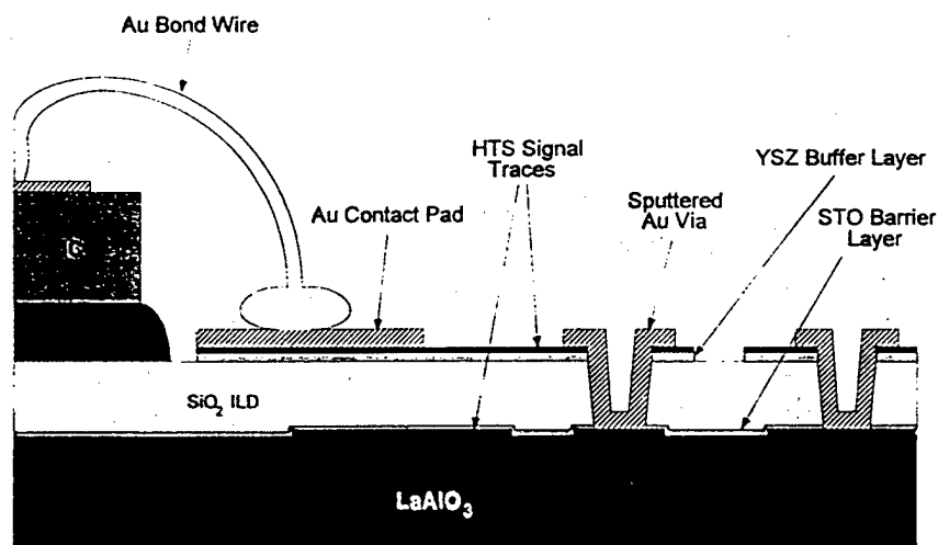
Figure 1: HTS MCM cross-section.
