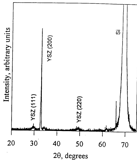
Figure 2. XRD scan of YSZ deposited on Si substrate with IBAD.
