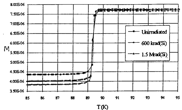
Figure 2. Critical temperature transition of YBa 2 Cu 3 O 7-x on a LaAlO 3 substrate after gamma irradiations.
