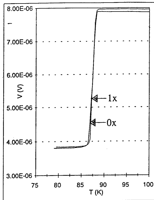
Figure 7: T_c of sputtered YBCO on YSZ
