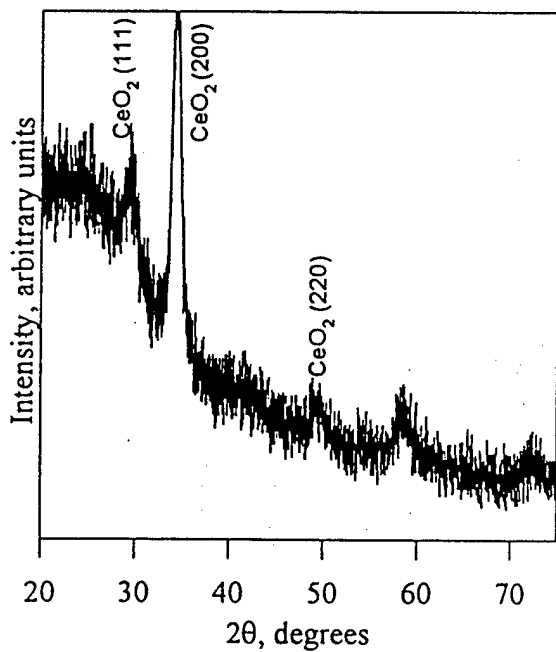
Figure 3. XRD scan of \text{CeO}_2 deposited on Pyrex with IBAD.
