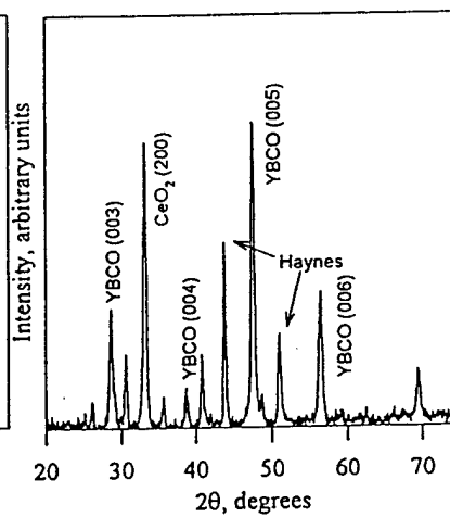
Figure 8. XRD scan of YBCO/CeO 2 deposited on Haynes with IBAD.
