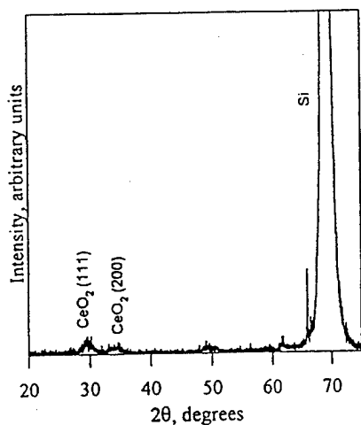
Figure 1. XRD scan of CeO 2 deposited on Si without IBAD.
