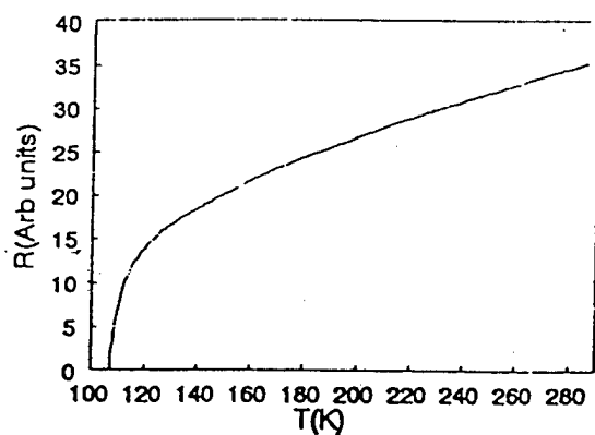
Fig. 2. Resistance vs. Temperature for the \text{Tl}_2\text{Ba}_2\text{CaCu}_3\text{O}_7 on \text{YSZ}/\text{Al}_2\text{O}_3 .
