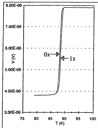
Figure 5: T_c of sputtered YBCO on YSZ
