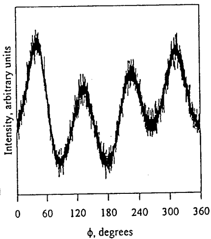
Figure 4. Phi scan of CeO 2 (111) family of peaks deposited on Pyrex.
