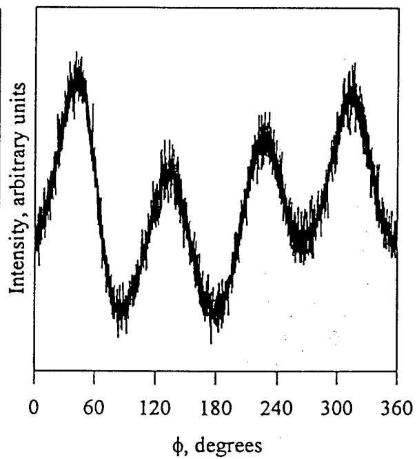
Figure 4. Phi scan of \text{CeO}_2 (111) family of peaks deposited on Pyrex.
