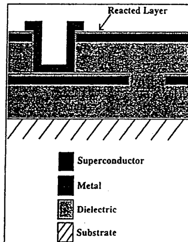
Figure 2: Reactivity of YBCO
