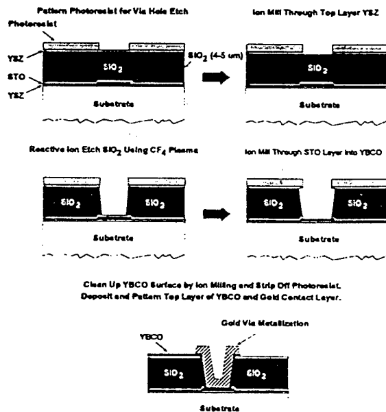
Figure 1. HTS via process.
