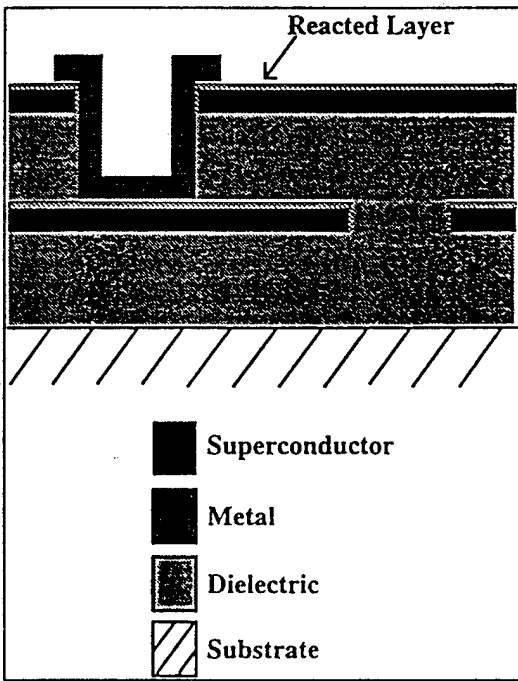
Figure 2: Reactivity of YBCO
