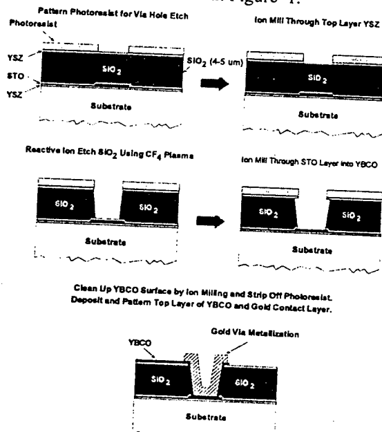
Figure 1. HTS via process.
