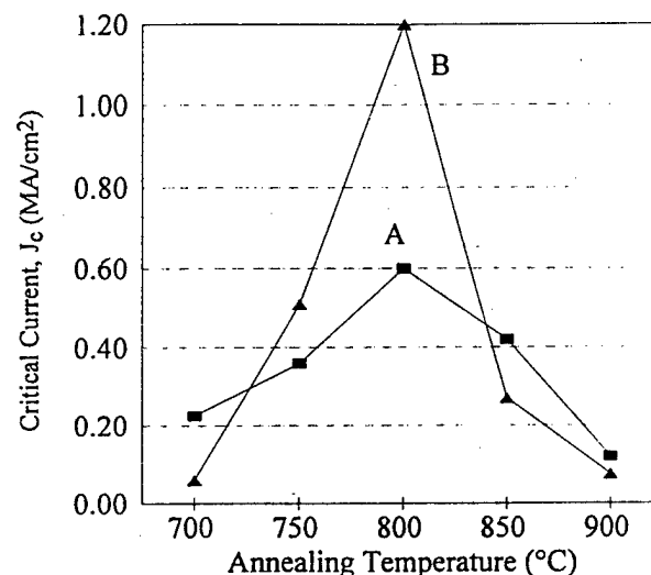
Figure 2. Critical current density versus annealing temperature plots for groups A and B of the YBCO samples.
