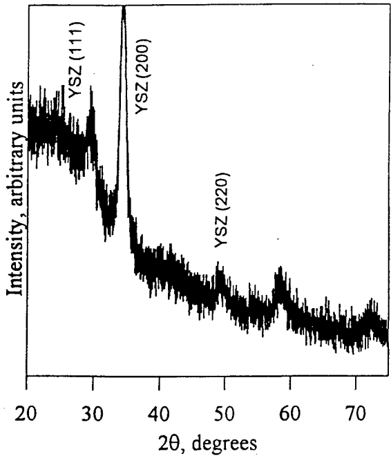
Figure 3. XRD scan of YSZ deposited on Pyrex substrate with IBAD.
