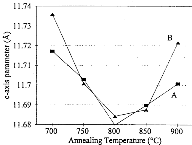
Figure 4. The c -axis parameter of the YBCO films as a function of annealing temperature.
