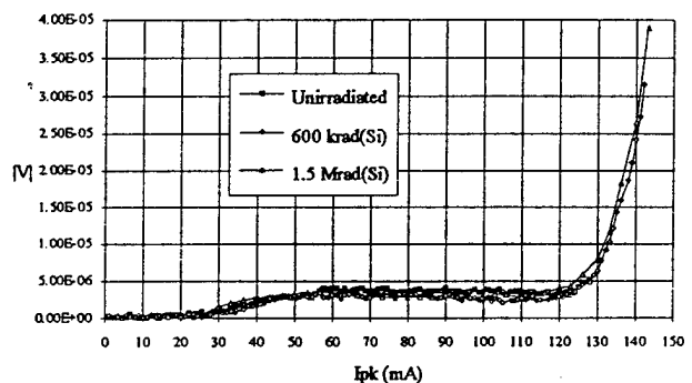
Figure 3. Critical current density measurement of YBa 2 Cu 3 O 7-x on a LaAlO 3 substrate after gamma irradiations.
