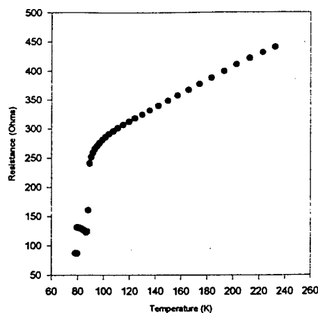
Figure 2. Temperature transition of a chain of ten 40 \mu\text{m} wide vias.
