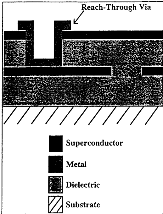
Figure 1: Interconnect Structure
