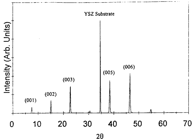
Figure 1. The XRD pattern of a typical as-deposited YBCO film.
