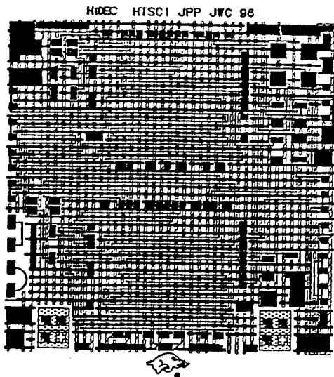
Figure 2. Layout of a 2 layer 15 mm x 15 mm HTS MCM-D substrate.
