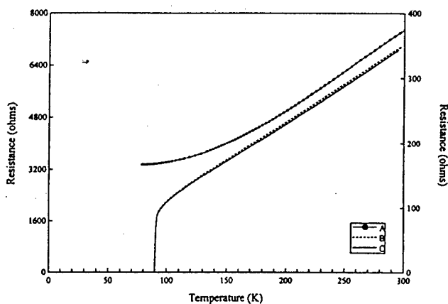
FIG. 4. Resistance versus temperature for the 40 \mu m wide bridge in the bottom YBCO. (A) After simulation of top YBCO deposition. (B) After annealing at 450 °C in 500 Torr of O_2 for 30 min. Left y-axis used for plot A and right y-axis used for plots B and C. (C) Before simulation of top YBCO deposition.
