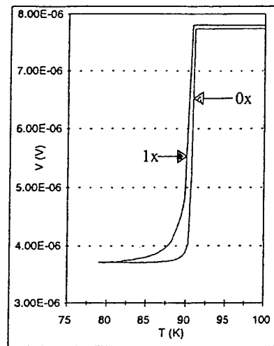
Figure 3: T_c of laser-deposited YBCO on LAO
