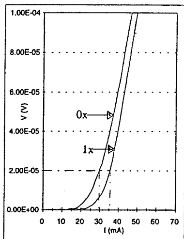
Figure 6: I_c of sputtered YBCO on YSZ
