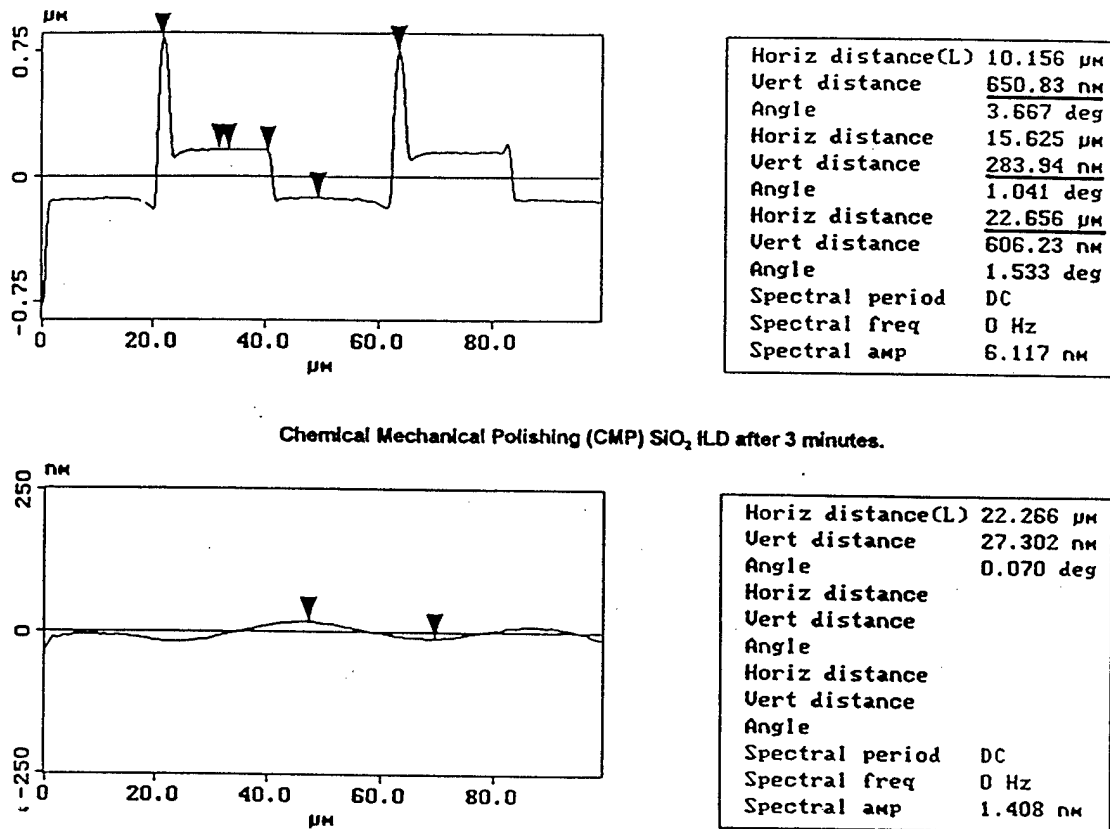
Figure 3. Step height reduction using silicon dioxide chemical-mechanical polishing (CMP) process.
