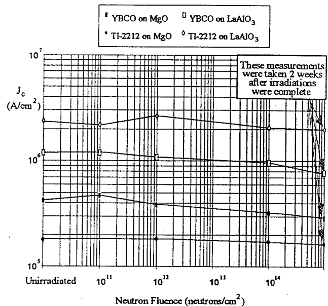
Figure 6. Critical current density variation of various superconductor/substrate combinations for different neutron fluences (also shown is the variation due to air exposure.)
