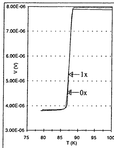
Figure 7: T_c of sputtered YBCO on YSZ
