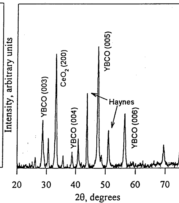
Figure 8. XRD scan of YBCO/CeO 2 deposited on Haynes with IBAD.
