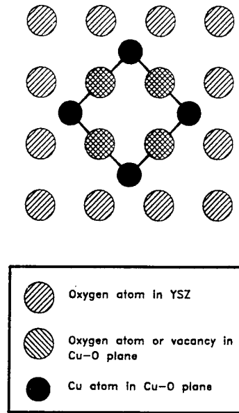
Figure 7. Illustration of the 45° (alignment of c -axis oriented YBCO on (100) oriented YSZ.
