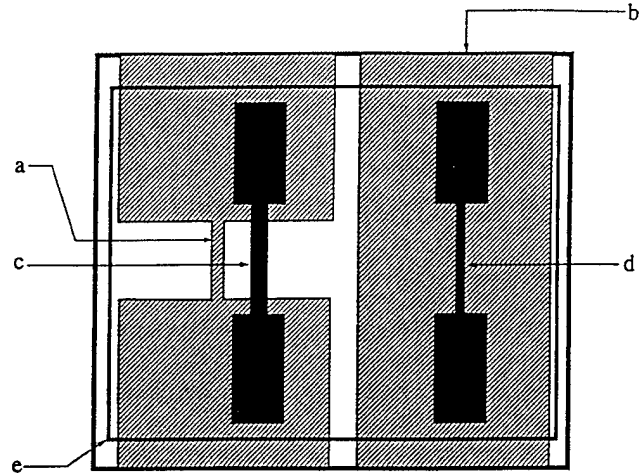
FIG. 2. Schematic of the patterned multilayer structure. (a) 40\ \mu\text{m} wide bridge in the bottom YBCO layer. (b) Unpatterned bottom YBCO layer. (c) 60\ \mu\text{m} wide bridge with step edges on the top YBCO layer. (d) 30\ \mu\text{m} wide bridge without step edges on the top YBCO layer. (e) YSZ/ SiO_2 /YSZ insulator layers.
