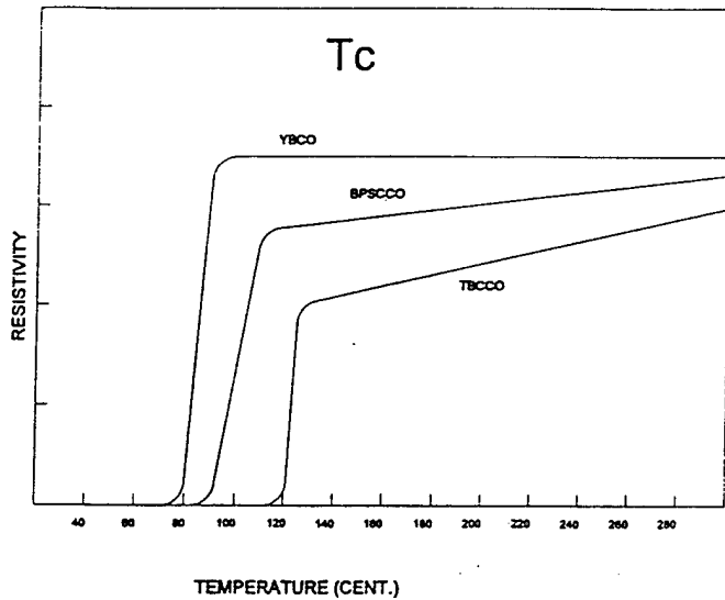
Fig. 2. Comparison of Typical T_c Curves.
