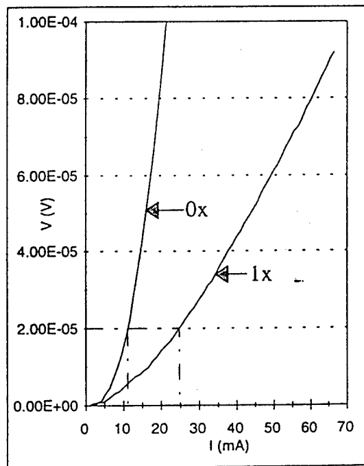
Figure 4: I_C of laser-deposited YBCO on LAO
