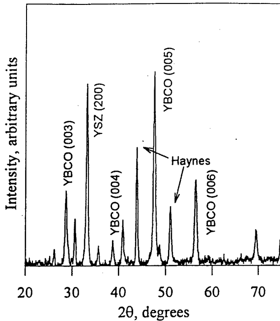
Figure 9. XRD scan of YBCO/YSZ deposited on Haynes alloy substrate with IBAD.
