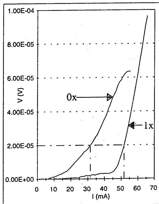
Figure 8: I_c of sputtered YBCO on YSZ
