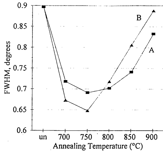
Figure 5. The FWHM versus annealing temperature for groups A and B of the YBCO samples.
