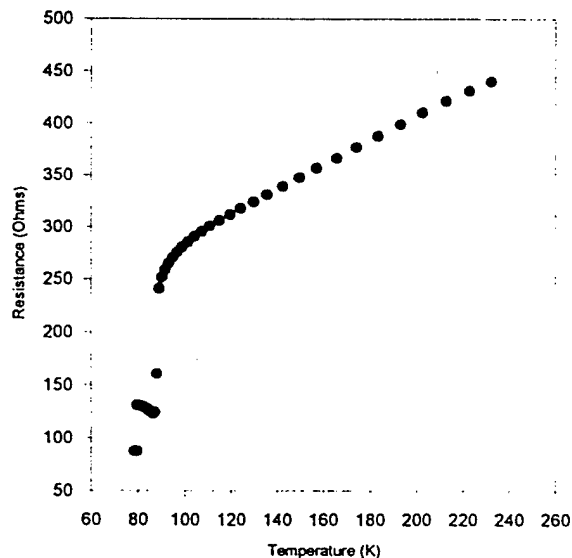
Figure 5: Temperature transition of a chain of ten 40 \mu\text{m} wide vias.
