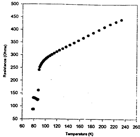
Figure 4. Temperature transition of a chain of ten 40 \mu\text{m} wide vias.
