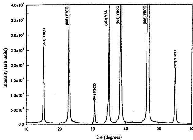
FIG. 1. \theta - 2\theta x-ray diffractometer pattern for the YBCO/YSZ/ SiO_2 /YSZ/YBCO structure on (001)YSZ.
