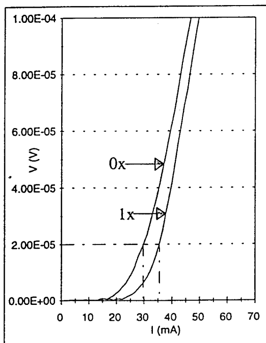
Figure 6: I_c of sputtered YBCO on YSZ
