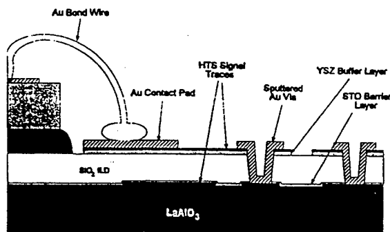
Figure 1. HTS MCM cross-section.
