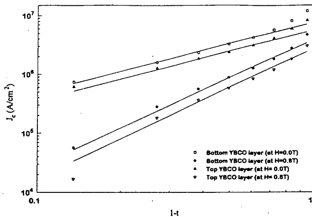
FIG. 3. Logarithmic plots of J_c vs 1-t for each of the YBCO layers within the multilayer structure. Straight lines are the curve fits to (1-t)^n , where n \sim 1.3 for H=0.0 T and n \sim 2.1 for H=0.8 T.
