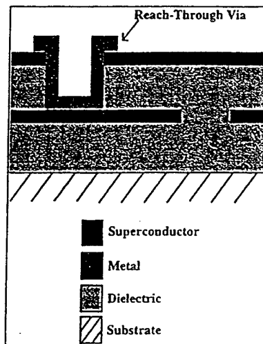
Figure 1: Interconnect Structure
