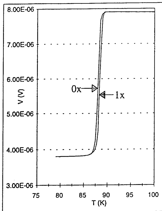
Figure 5: T_c of sputtered YBCO on YSZ
