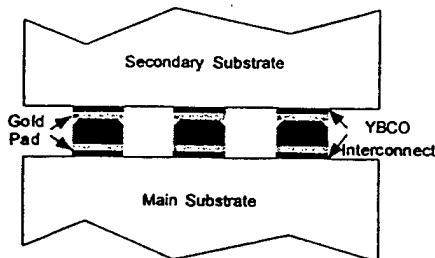
Figure 6. Flip-Mesh via cross-section.
