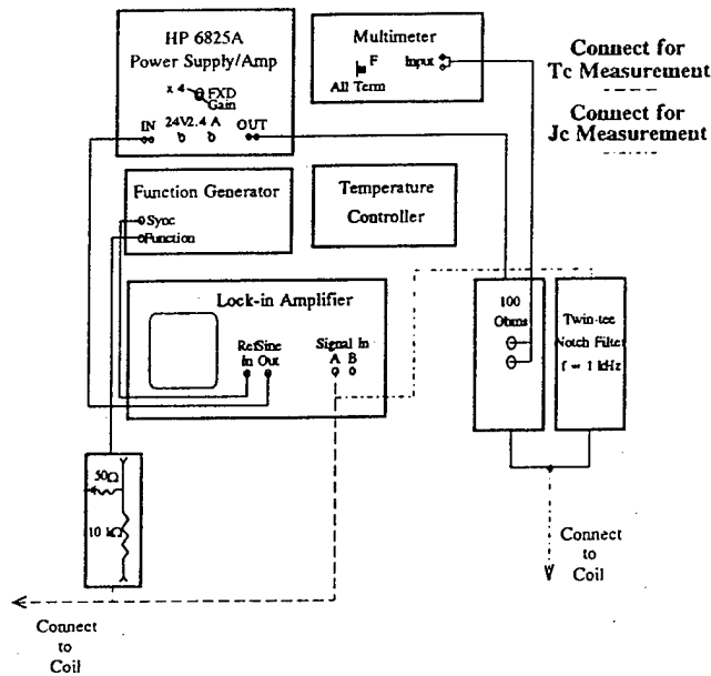
Figure 1. Critical temperature and critical current density measurement system schematic.
