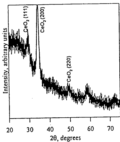
Figure 3. XRD scan of CeO 2 deposited on Pyrex with IBAD.
