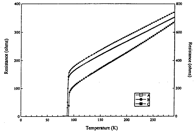
FIG. 3. Resistance versus temperature for the (A) 40\ \mu\text{m} wide bridge in the bottom YBCO layer. (B) 60\ \mu\text{m} wide bridge in the top YBCO layer with step edges. (C) 30\ \mu\text{m} wide bridge in the top YBCO layer without step edges. Left y-axis used for plots A and C and right y-axis for plot B.
