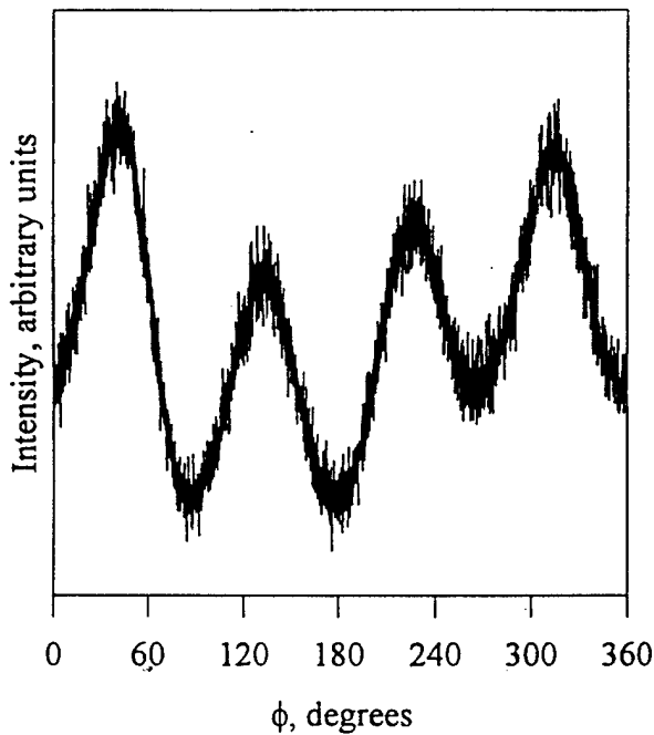
Figure 6. \phi scan of YSZ (111) family of peaks for the film shown in figure 5.
