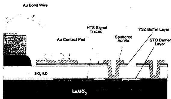
Figure 1. HTS MCM cross-section.
