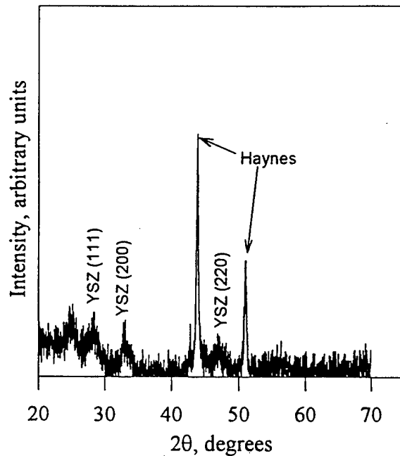
Figure 8. XRD scan of YSZ deposited on Haynes alloy substrate without IBAD.
