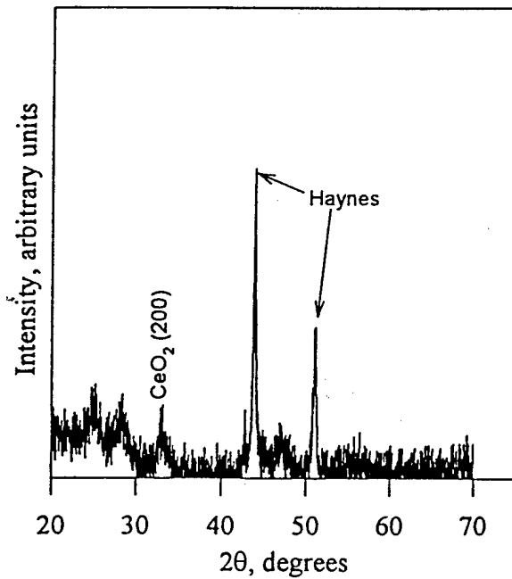
Figure 7. XRD scan of CeO 2 deposited on Haynes without IBAD.
