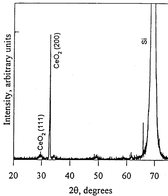
Figure 2. XRD scan of \text{CeO}_2 deposited on Si with IBAD.
