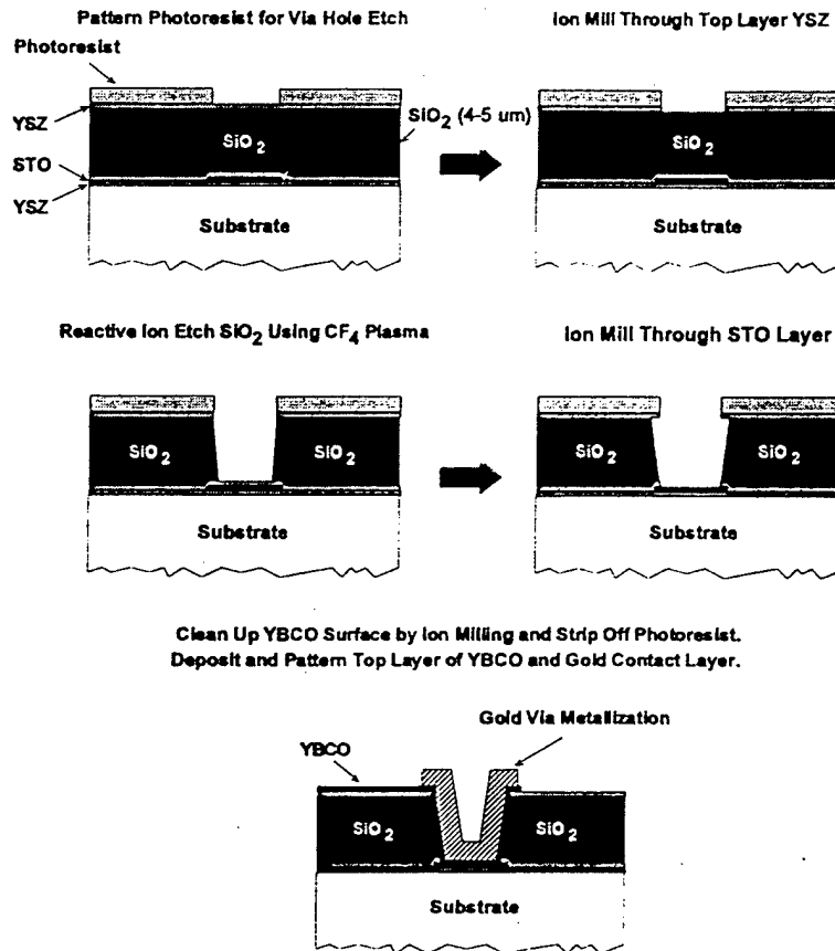
Figure 4: HTS via fabrication process.
