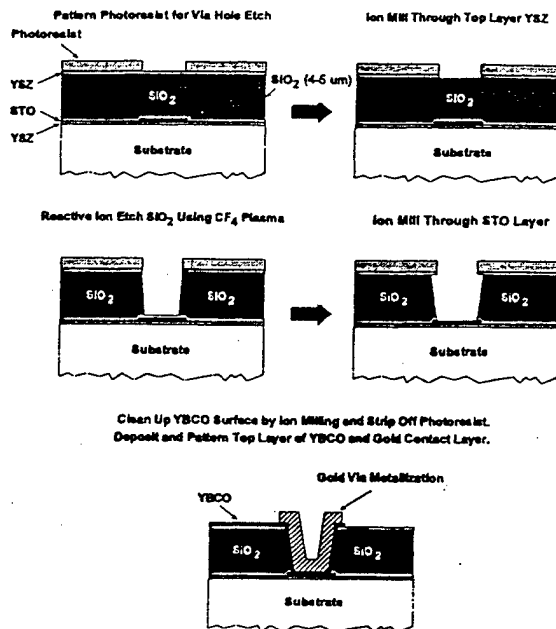
Figure 3. HTS via fabrication process.
