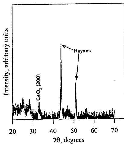
Figure 7. XRD scan of CeO 2 deposited on Haynes without IBAD.
