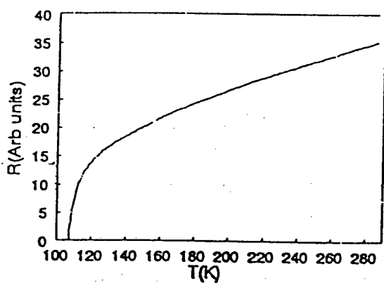
Fig. 2. Resistance vs. Temperature for the \text{Tl}_2\text{Ba}_2\text{CaCu}_1\text{O}_x on \text{YSZ}/\text{Al}_2\text{O}_3 .
