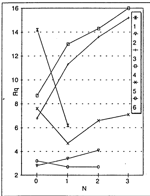
Figure 10: RMS roughness vs. number of mills
