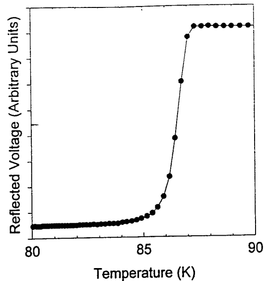
FIG. 3. The critical temperature curve of the YBCO shown in Fig. 2.
