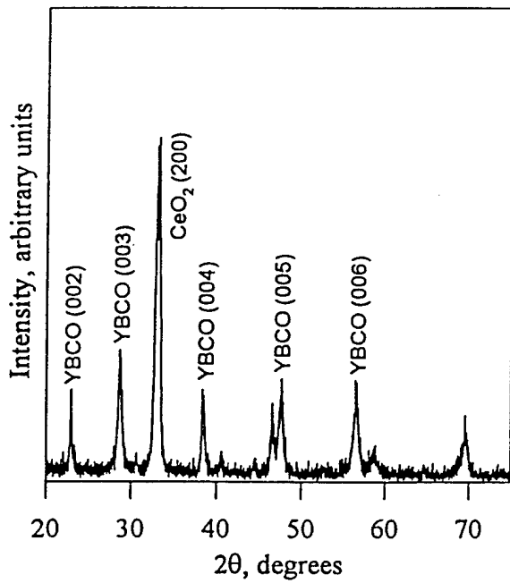
Figure 5. XRD scan of YBCO/CeO 2 deposited on Pyrex with IBAD.
