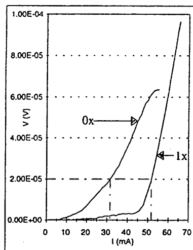
Figure 8: I_c of sputtered YBCO on YSZ
