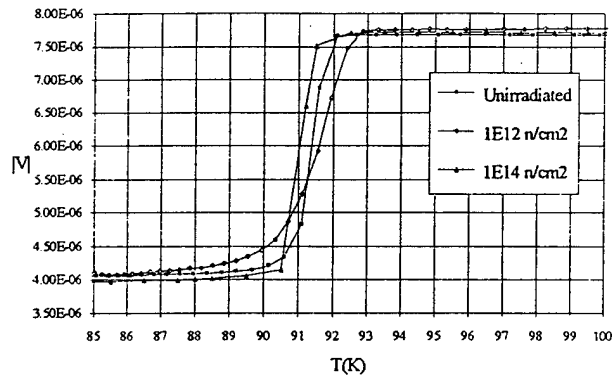
Figure 4. Critical temperature transition of Tl_2Ba_2CaCu_2O_{8+x} on a MgO substrate after various neutron fluences.
