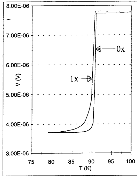
Figure 3: T_C of laser-deposited YBCO on LAO
