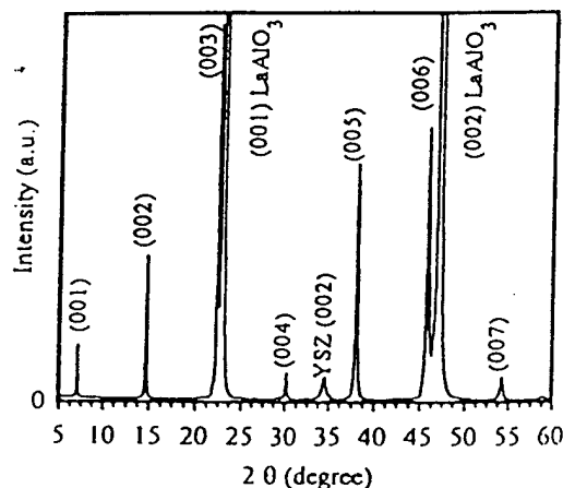
Fig. 1 X-ray diffraction pattern for a multilayer YBCO/YSZ/SiO 2 /YSZ/YBCO sample
