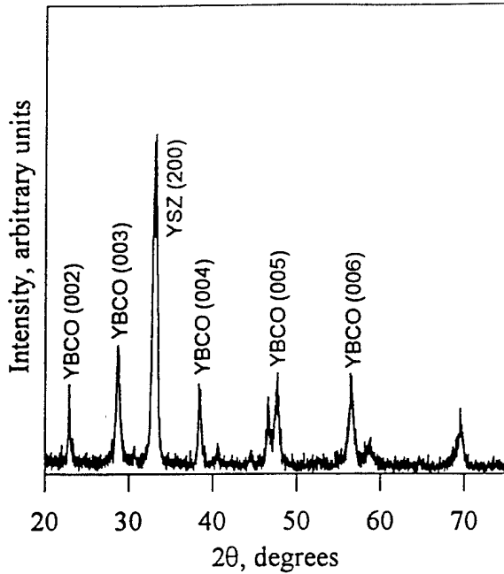
Figure 5. XRD scan of YBCO/YSZ deposited on Pyrex substrate with IBAD.
