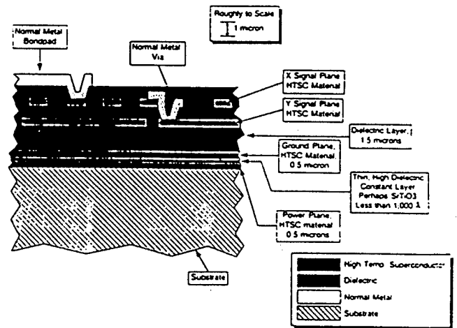
Fig. 1. Cross-sectional Schematic of a Superconducting Multi-Chip Module.
