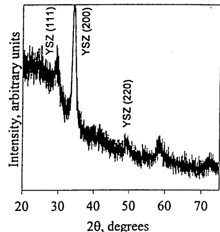
FIG. 1. Theta-two theta scan for a typical YSZ film deposited on Pyrex.
