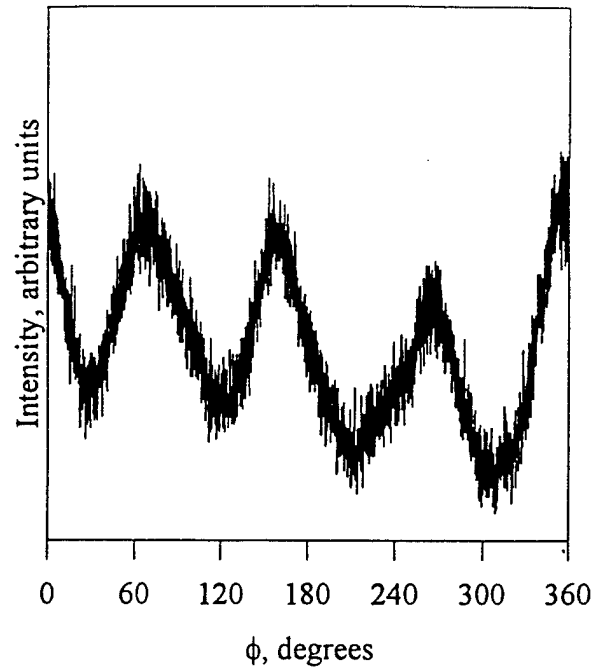
Figure 4. \phi scan of YSZ (111) family of peaks for the film shown in figure 3.
