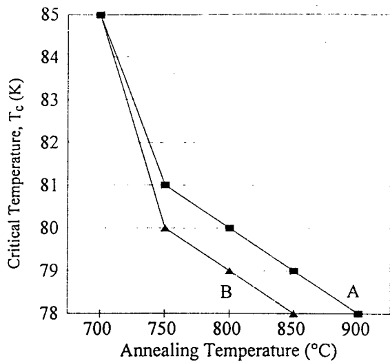
Figure 3. Critical transition temperature versus annealing temperature plots for groups A and B of the YBCO samples.
