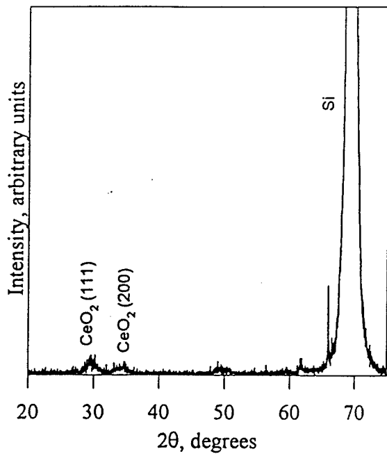
Figure 1. XRD scan of \text{CeO}_2 deposited on Si without IBAD.
