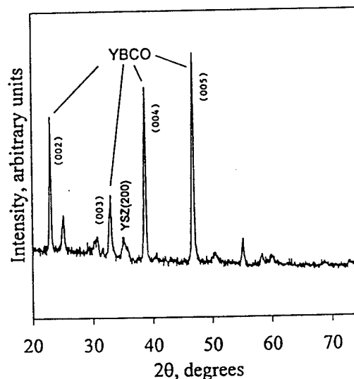
FIG. 4. Theta-two theta scan of the top YBCO layer.
