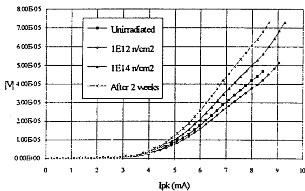
Figure 5. Critical current density measurement of Tl_2Ba_2CaCu_2O_{8+x} on a MgO substrate after various neutron fluences.
