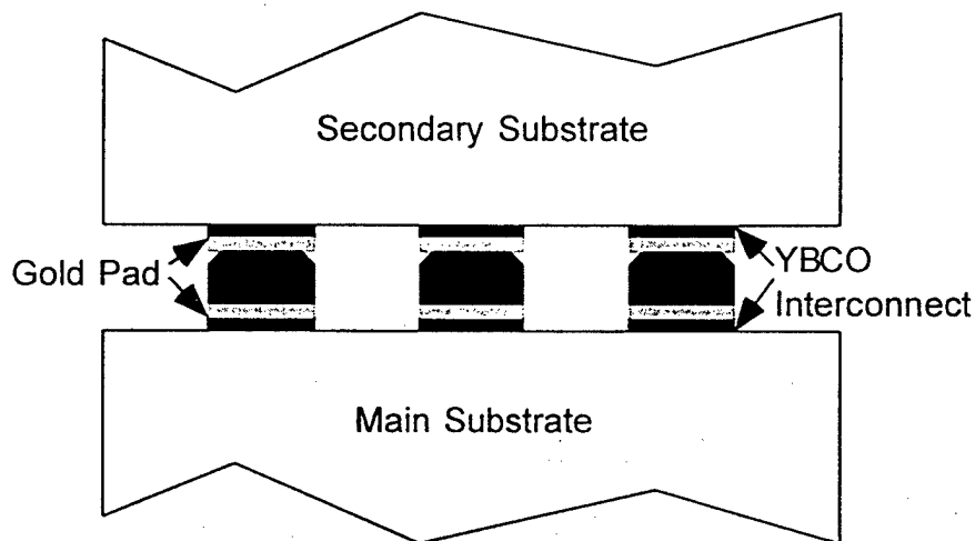
Figure 2: Flip-Mesh Via Cross-Section
