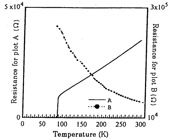
Fig. 2 Resistance versus temperature curves for (A) 20 \mu\text{m} wide bottom YBCO serpentine line, (B) 20 \mu\text{m} wide top YBCO serpentine line
