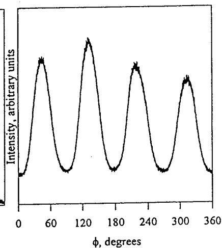
Figure 6. Phi scan of YBCO (103) family of peaks on CeO 2 /Pyrex.
