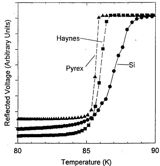
Figure 10. Transition temperature measurements for YBCO deposited on three different substrate materials.
