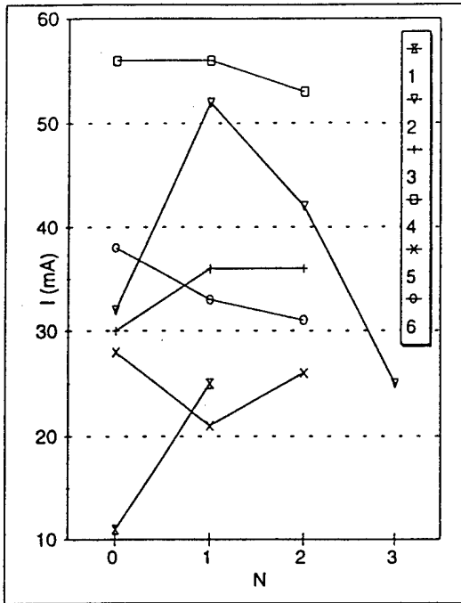
Figure 9: I_c vs. number of mills
