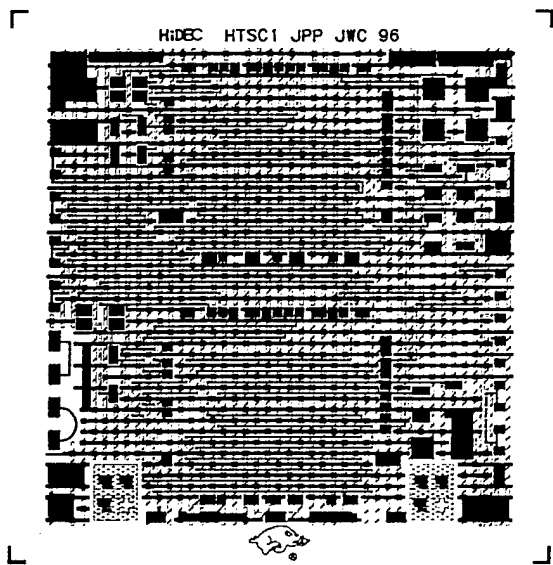
Figure 2. Layout of a 2 layer 15 mm x 15 mm HTS MCM-D substrate.
