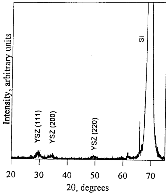
Figure 1. XRD scan of YSZ deposited on Si substrate without IBAD.
