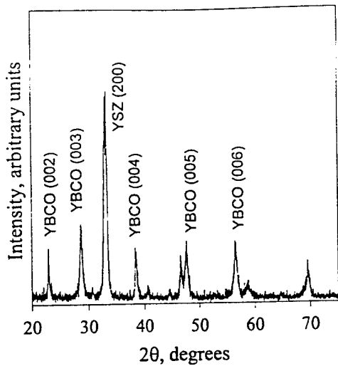
FIG. 2. Theta-two theta scan for a typical YBCO/YSZ structure deposited on Pyrex.
