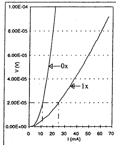
Figure 4: I_c of laser-deposited YBCO on LAO
