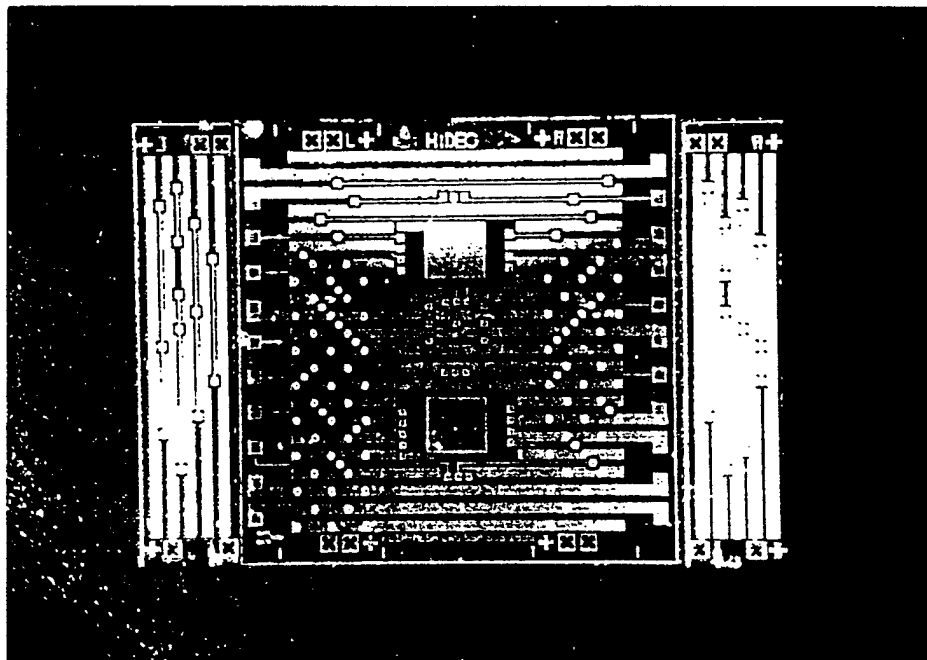
Figure 3: Assembled Flip-Mesh Module
