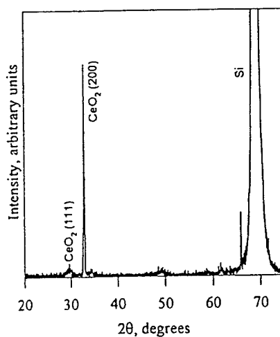
Figure 2. XRD scan of CeO 2 deposited on Si with IBAD.
