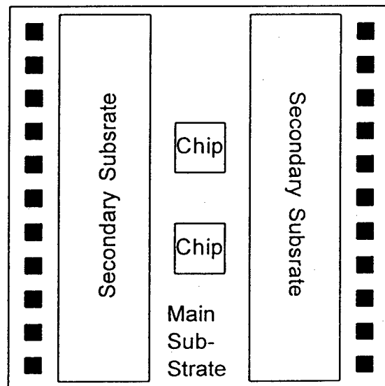
Figure 5. Flip-Mesh substrate configuration.
