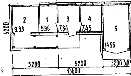
Fig. 5. 1--storeroom; 2--shed; 3--supply room; 4--woodworking shop; 5--garage.
