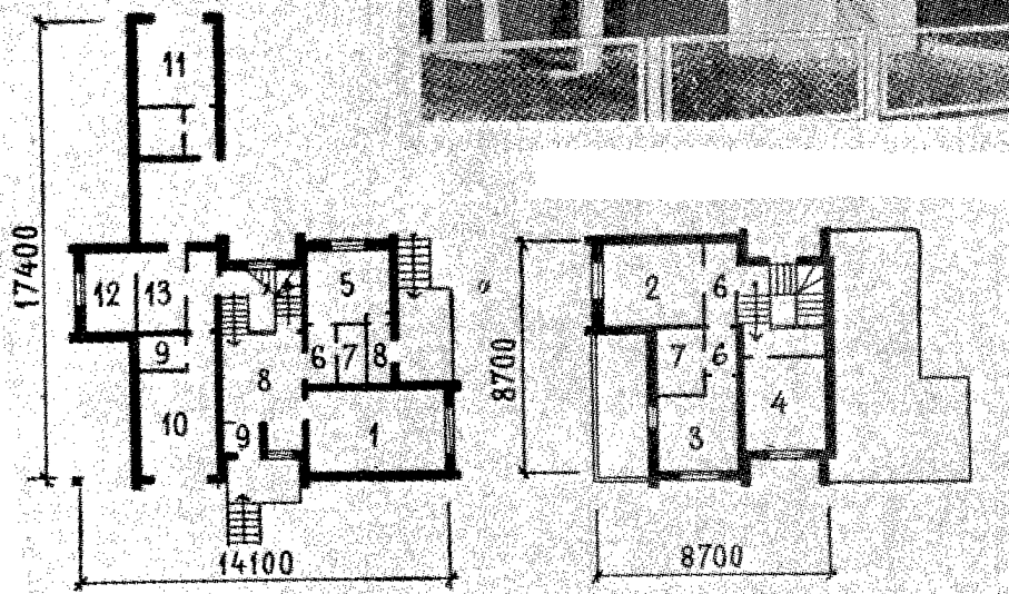
Fig. 6. Single-occupancy House. 1--living room; 2,3,4--bedrooms; 5--kitchen; 6--hall; 7--bathrooms; 8--entrance hall; 9,12--storerooms; 10--garage; 11--livestock pen; 13--feed preparation room.
