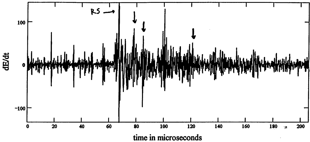
Figure 7: dE/dt waveforms for the first two strokes in figure 1. The strokes occurred 800 microseconds apart and were located 1.2 km apart. The main return stroke peaks are marked "RS" as well as locations obtained during the fine structure.
