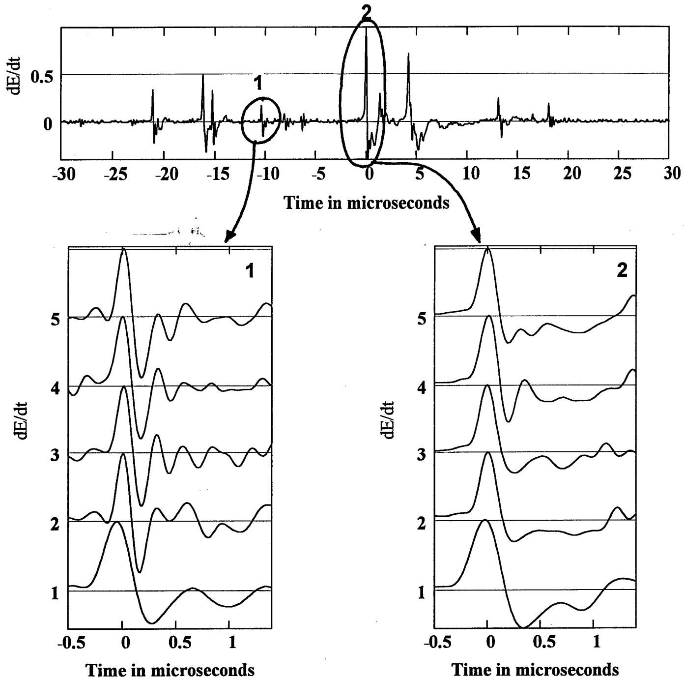
Figure 4 dE/dt pulses wavelshapes in bipolar pulse in C-G flash #254/2979
