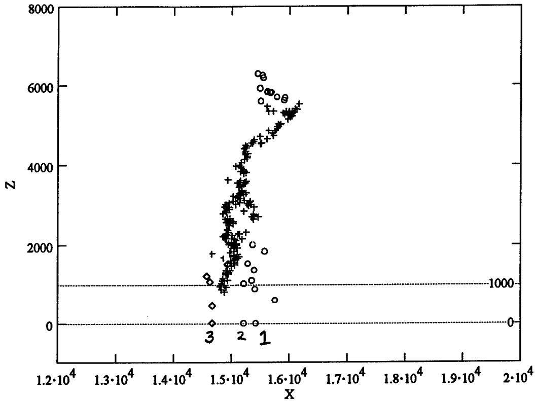
Figure 8 Locations of dE/dt sources preceding a new termination to ground in flash 24200770. Pulse train source locations shown as +'s. Stepped leader sources immediately prior to new termination shown as diamonds. New termination is labeled "3".
