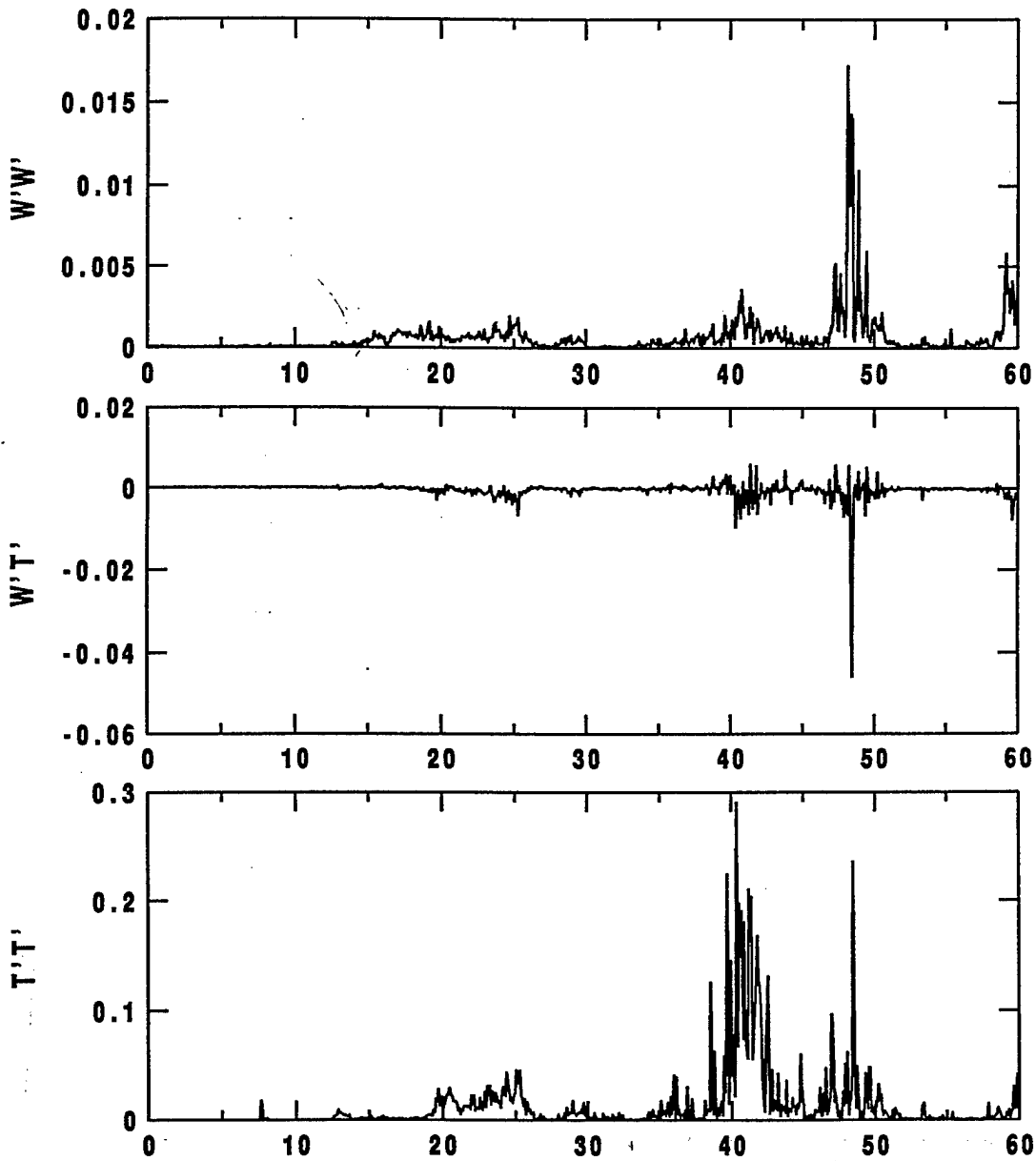
Figure 4. Vertical velocity variance, heat flux and temperature variance (dimensional) based on 10 Hz data at 3m on March 19, 1995 (2100—2200 CST, March 18, 1995).
