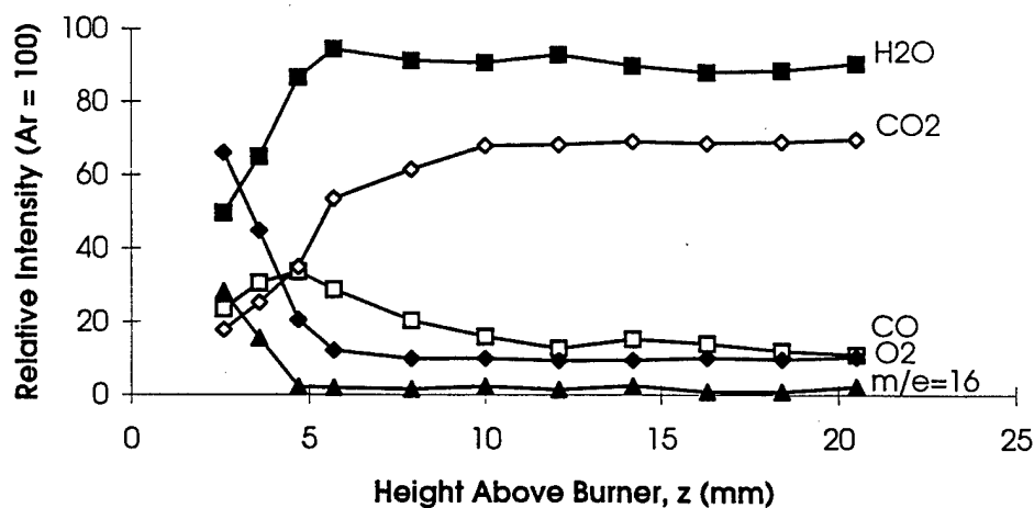
Figure 83. Experiment C133_Z: 40 torr, \phi = 0.94 —Principal Species in the Inhibited Flame as a Function of Distance of Quartz Probe from Burner.
