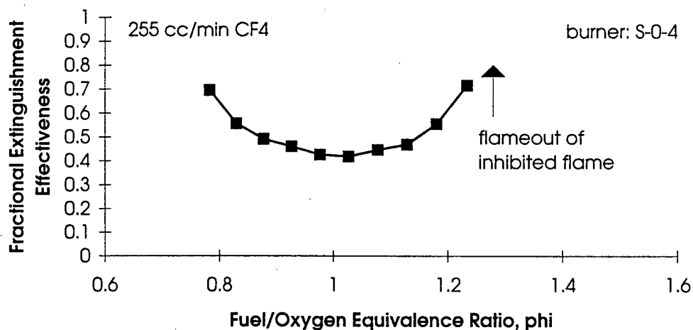
Figure 46. Inhibition of a \text{CH}_4 -Air Flame by \text{CF}_4 : Fractional Extinguishment Effectiveness.
