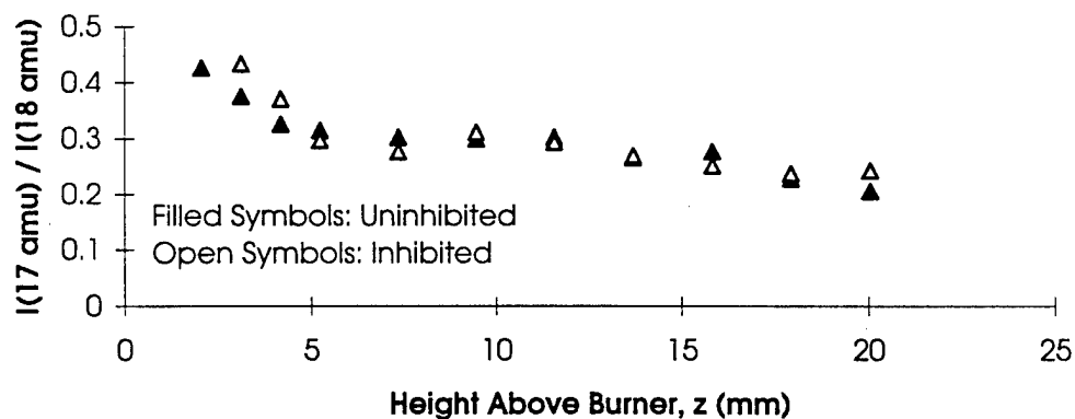
Figure 110. Experiment C148_Z: 35 torr, \phi = 1.00 —Apparent Fragmentation Ratios (17 amu/18 amu)
