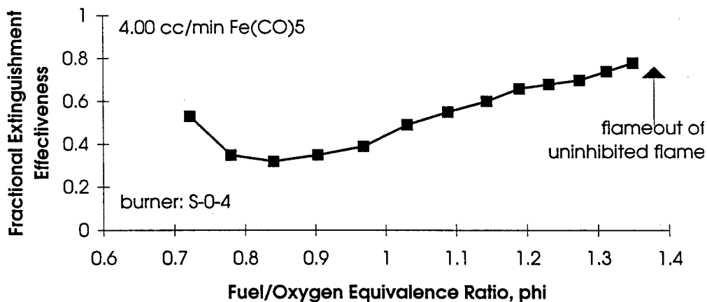
Figure 120. Inhibition by Fe(CO) 5 : Fractional Extinguishment Effectiveness.
