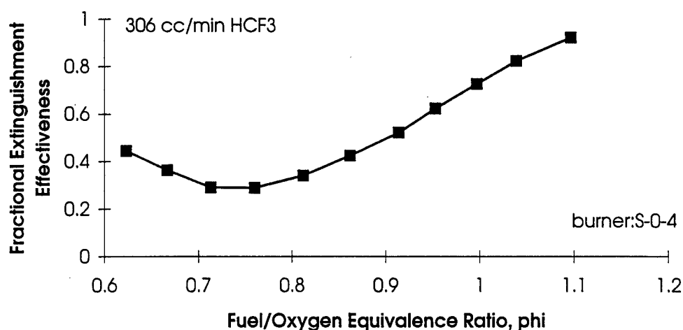
Figure 54. Inhibition of a CH 4 -Air Flame by CHF 3 : Fractional Extinguishment Effectiveness.
