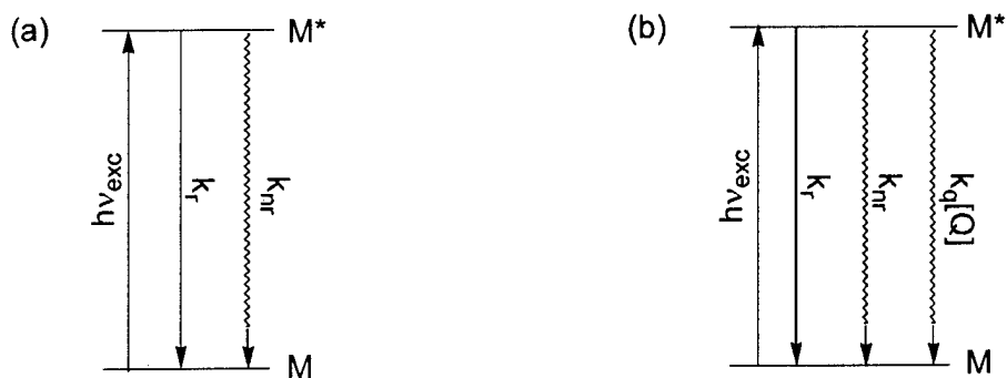
Figure 1. (a) Excited state diagram for (a) intramolecular and (b) intramolecular and intermolecular decay processes of a molecule in an excited state, M^* .
