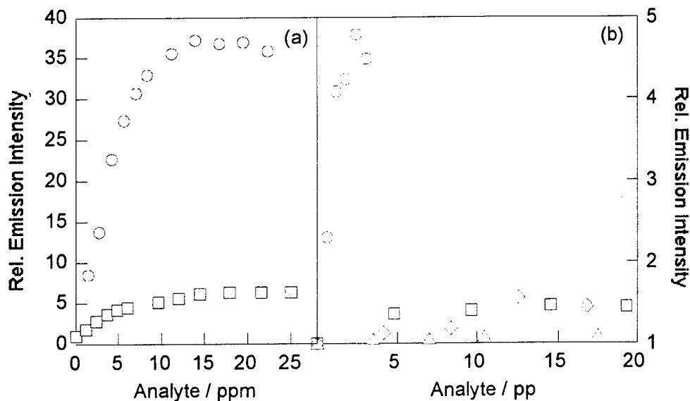
Figure 5. Relative emission intensity of aqueous solutions of DTPA cradle in the presence of selected (a) bicyclic (naphthalene, \circ ; biphenyl, \square ) and (b) monocyclic (benzene, \triangle ; toluene, \diamond ; xylene, \square ; durene, \circ ) aromatics.
