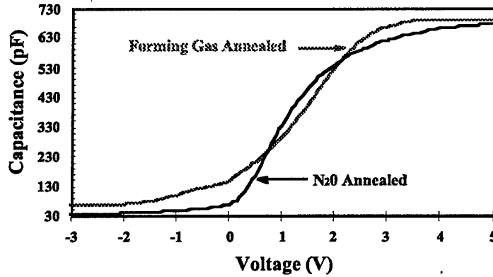
Figure 7. 1 MHz C-V measurement of \text{Ga}_2\text{O}_3/\text{GaN} MIS capacitors.
