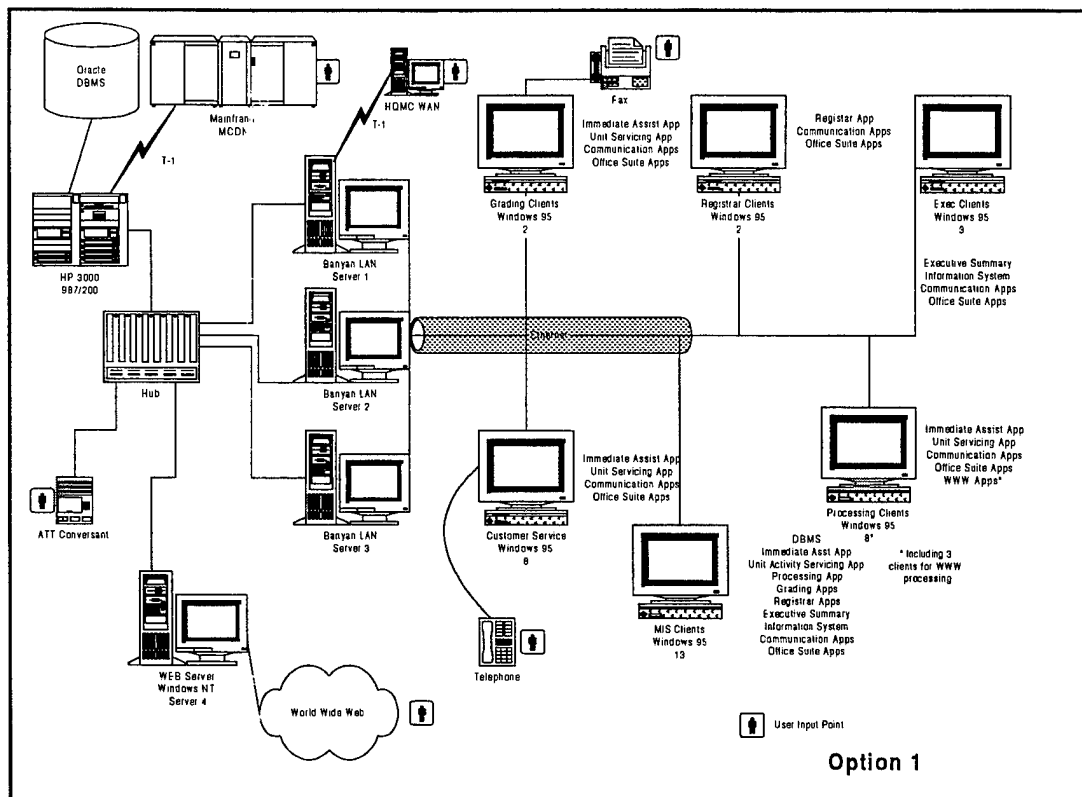
Figure 2. Option One Technology Architecture.
