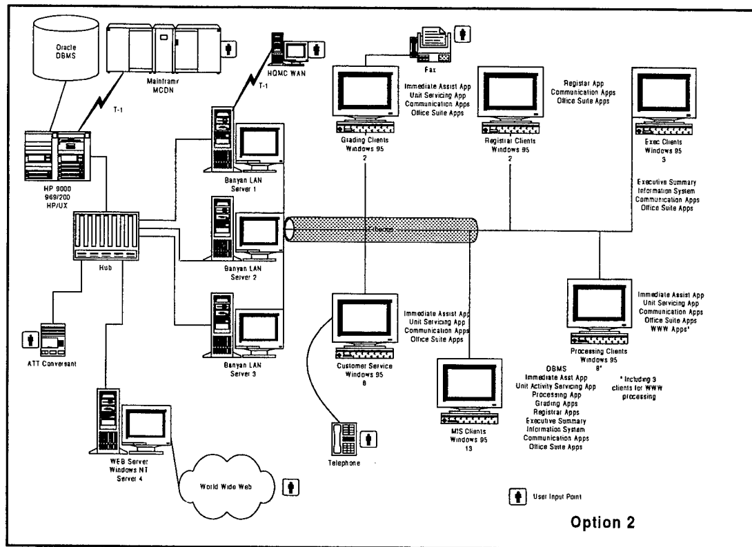
Figure 3. Option Two Technology Architecture.
