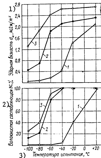
Figure 1. Variation in Impact Ductility, a_u , and Amount of Fiber in Fracture, VS , of 1420 \times 15 -mm Pipes Made of 17G1S-U Steel as Function of Testing Temperature: 1--hot-rolled state; 2, 3--thermally hardened; (1, 2--samples of type 11; 3--of type 1)
