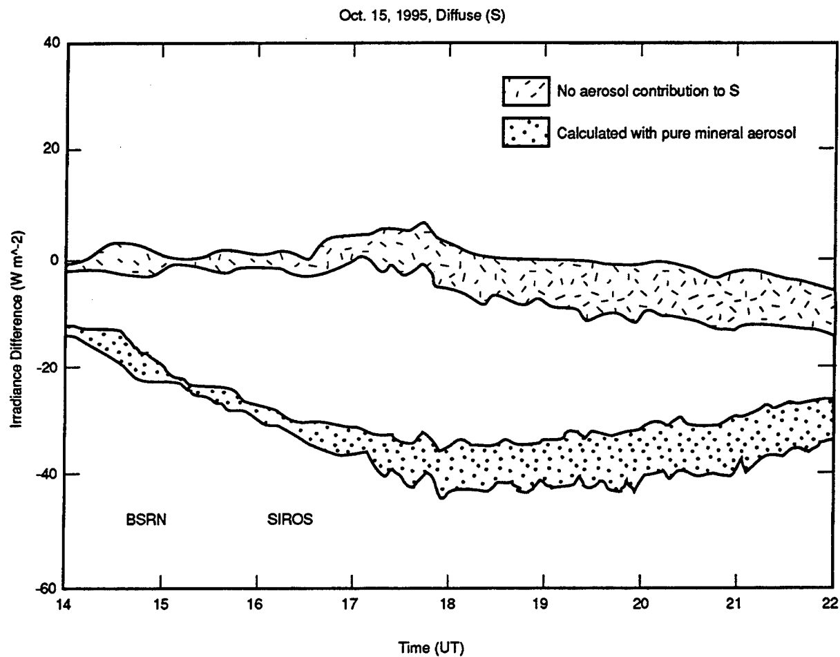
Figure 4. Measured scattered short wave radiation (s) — calculated scattered short wave radiation, when aerosol abundance is adjusted to fit observed attenuation of the direct solar incidence at the ground. The water vapor contribution to absorption is calculated from standard codes and measured M ( 1.1 \text{ g cm}^{-2} ).
