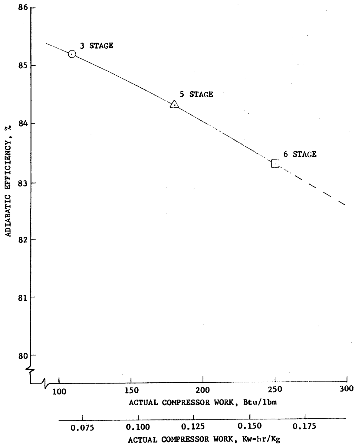
Figure 24. Compressor Efficiency
