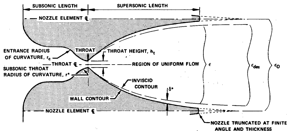
Figure 60. Nozzle Terminology
