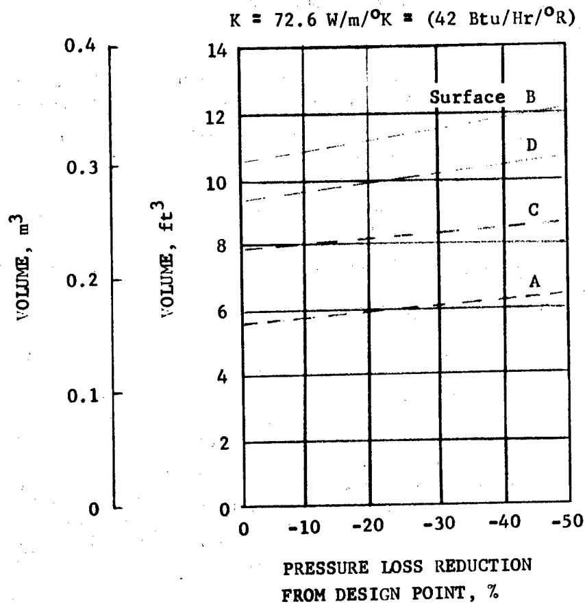
Figure 84. Effect of Pressure Loss on 1-Mw System Heat Source Heat Exchanger Volume
