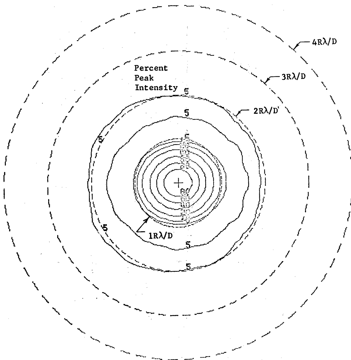
Figure 9. Typical Unstable Resonator Far-Field Intensity Distribution at High Geometric Coupling
