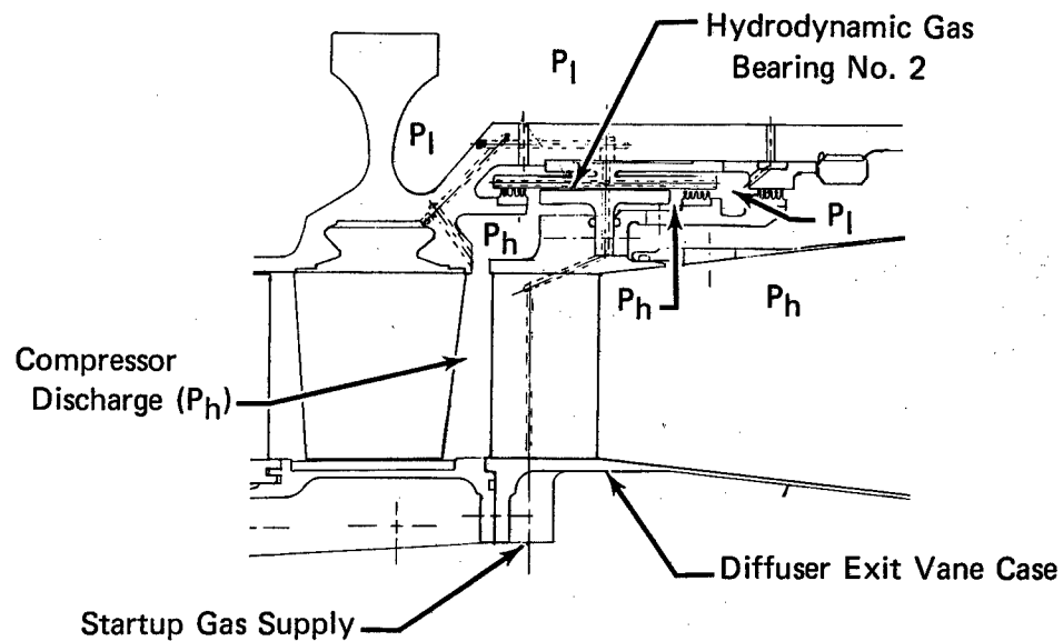
Figure 74. Hydrodynamic No. 2 Journal Gas Bearing
