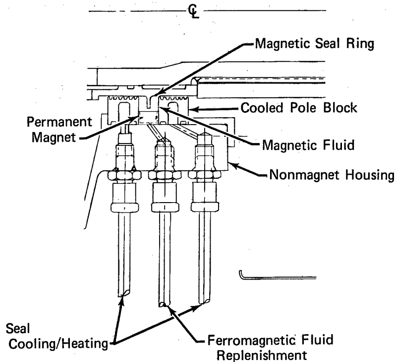
Figure 76. Centrifugal Ferrofluidic Shaft Seal
