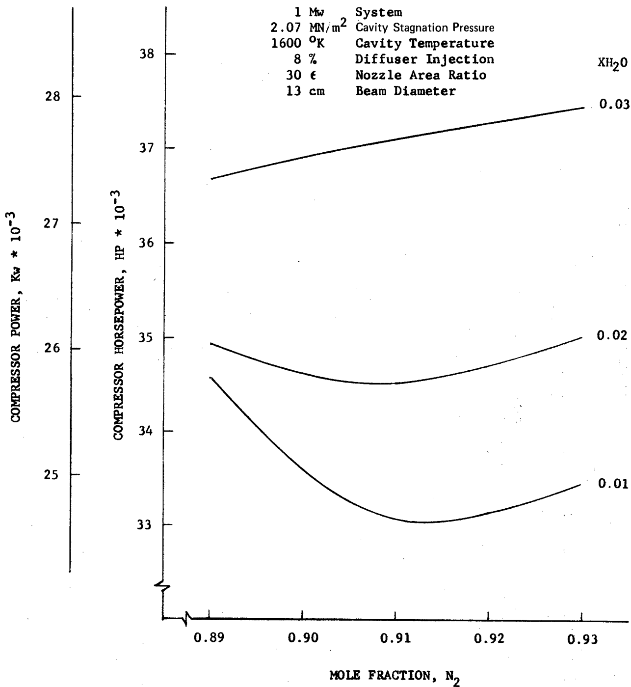
Figure 30. Effect of Gas Composition on Compressor Power Requirement
