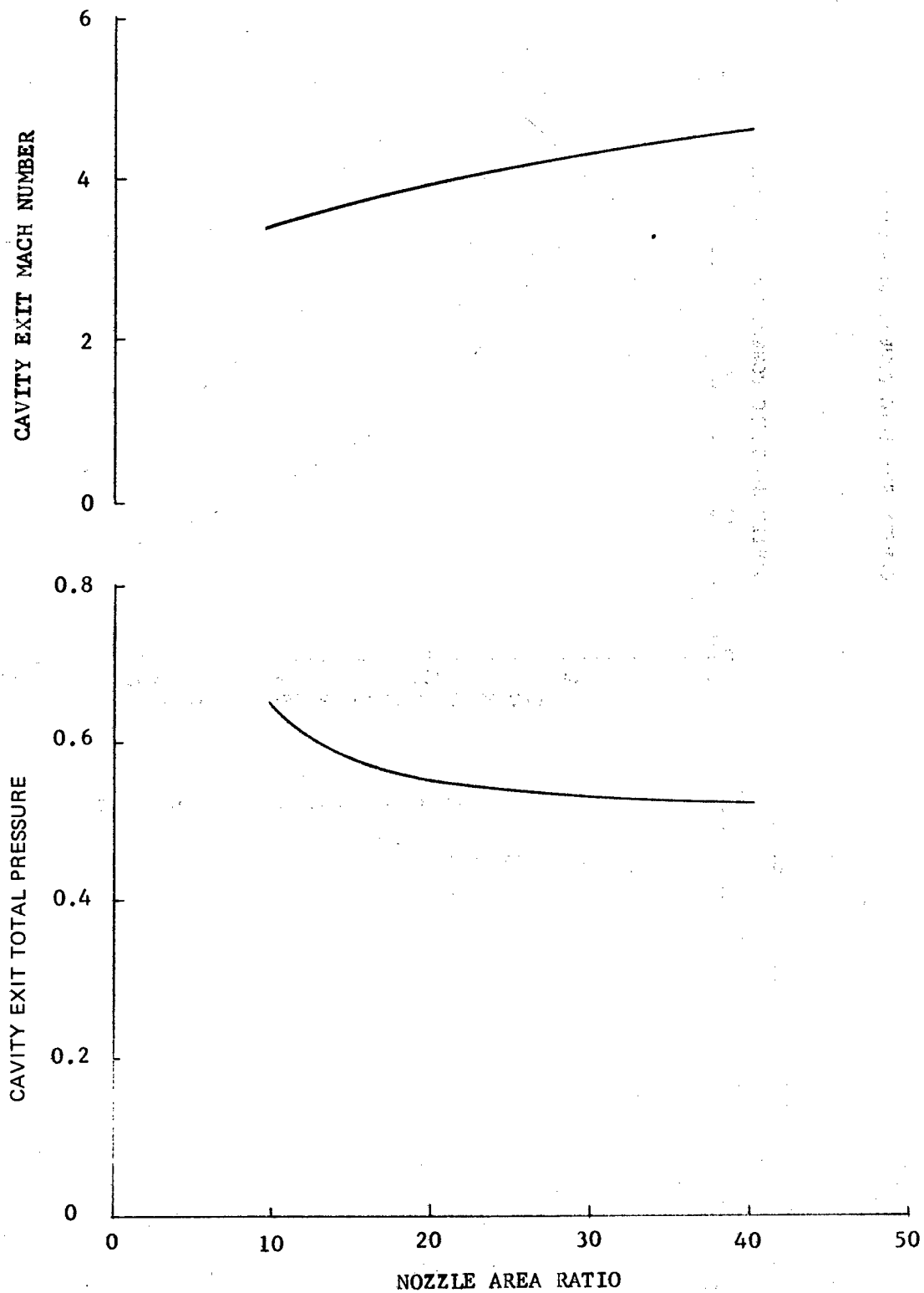
Figure 14. Cavity Mach Number and Exit Total Pressure
