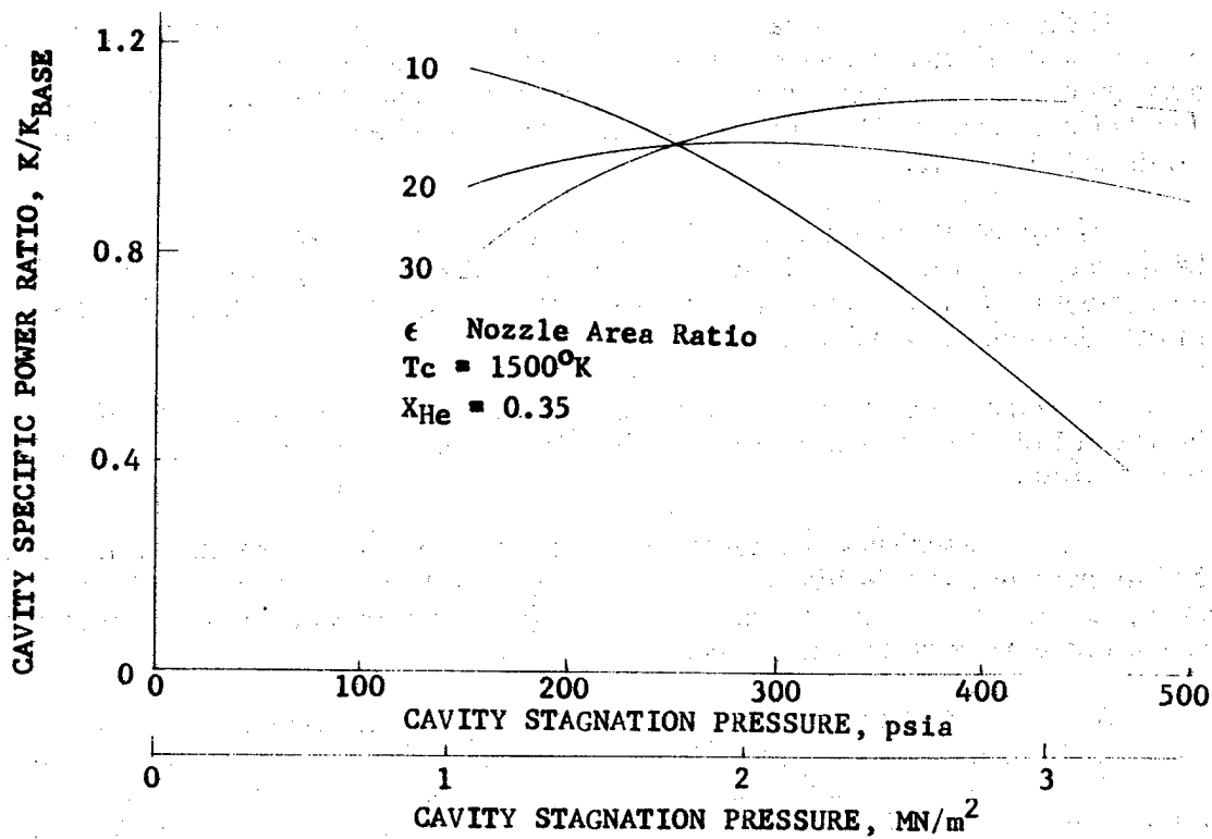
Figure 35. Effect of Cavity Stagnation Pressure on Performance
