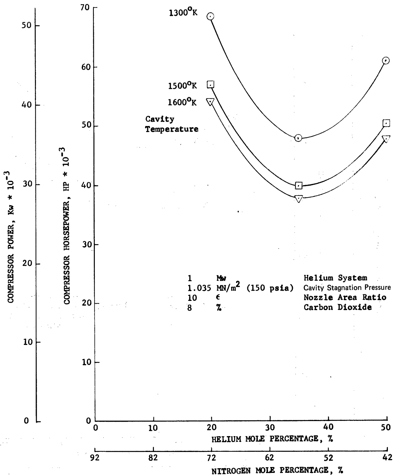
Figure 36. Effect of Helium Mole Percentage and Cavity Stagnation Temperature on Compressor Power Requirement
