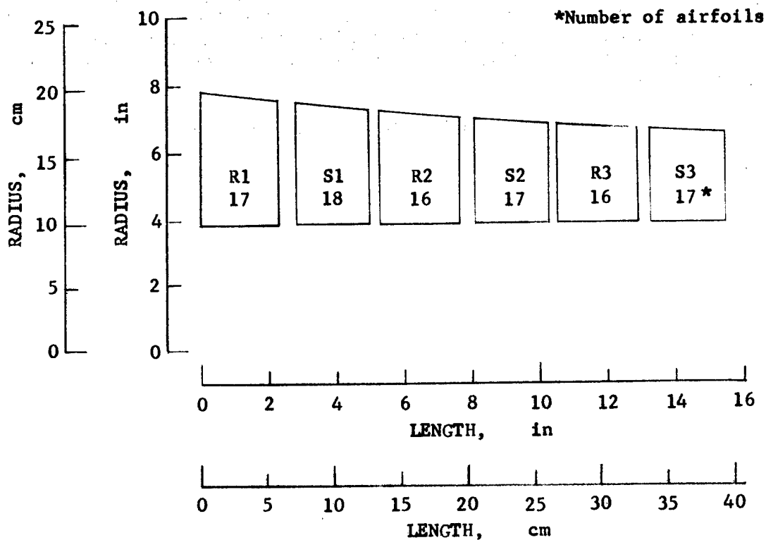
Figure 20. Three-Stage Compressor
