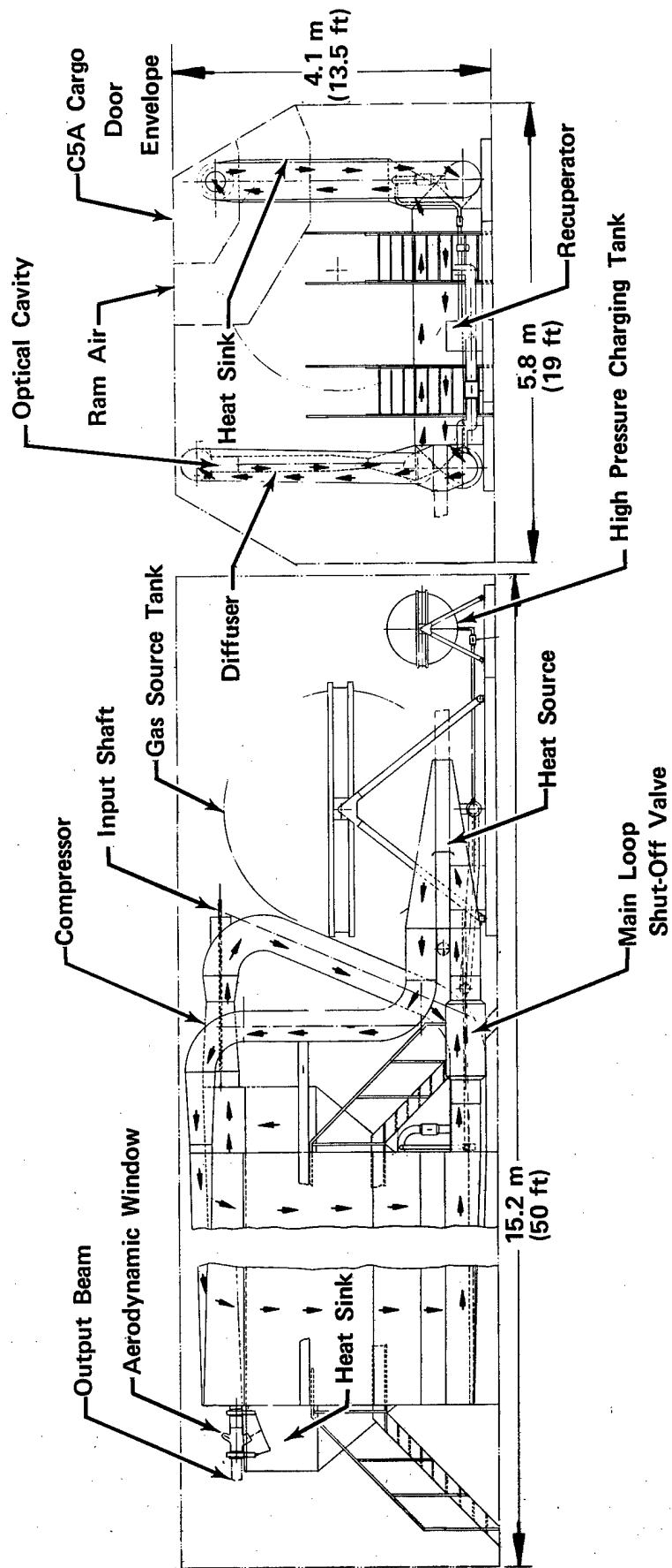
Figure 58. Closed-Cycle GDL Airborne Application
