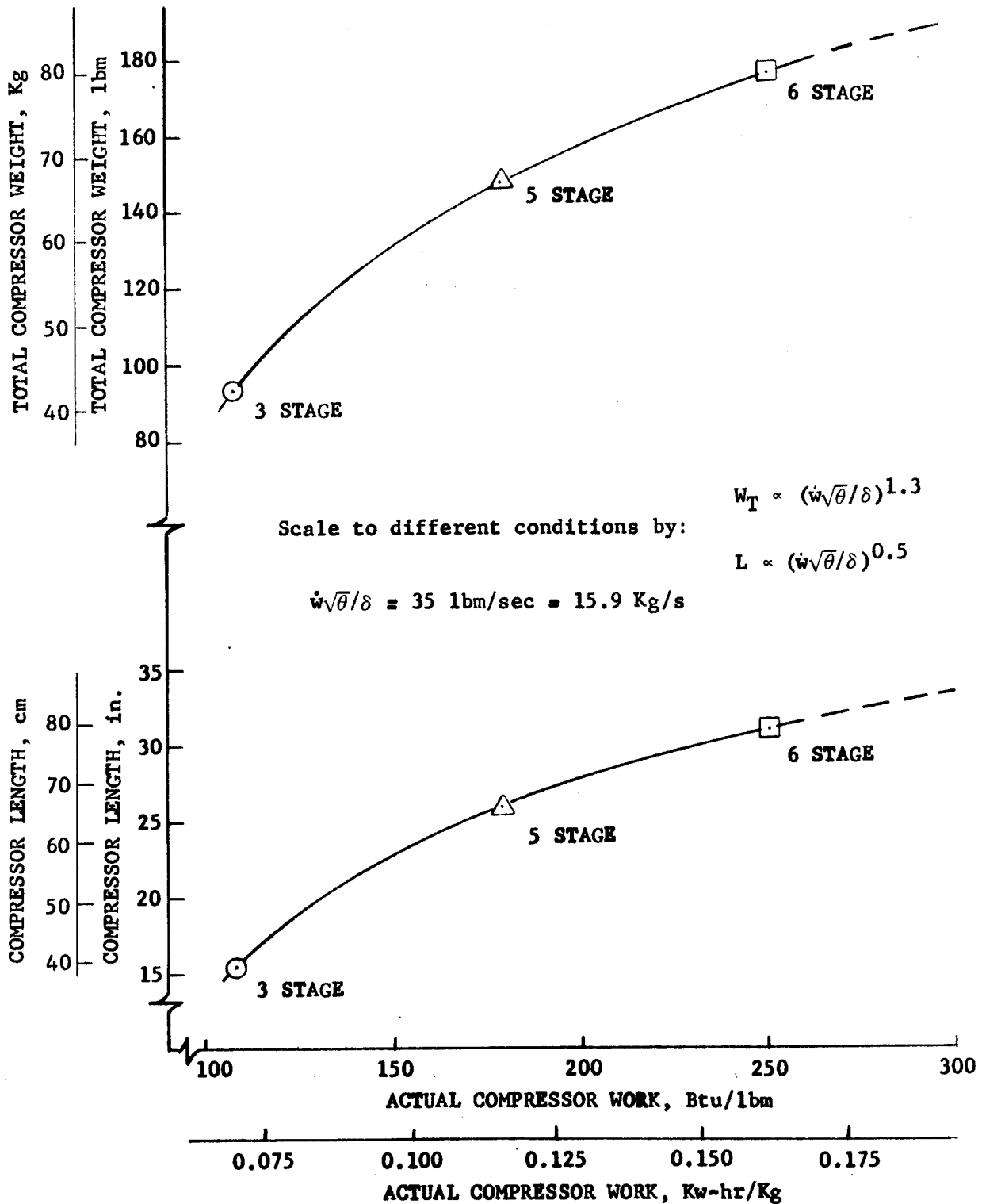
Figure 23. Compressor Weight and Geometry Characteristics
