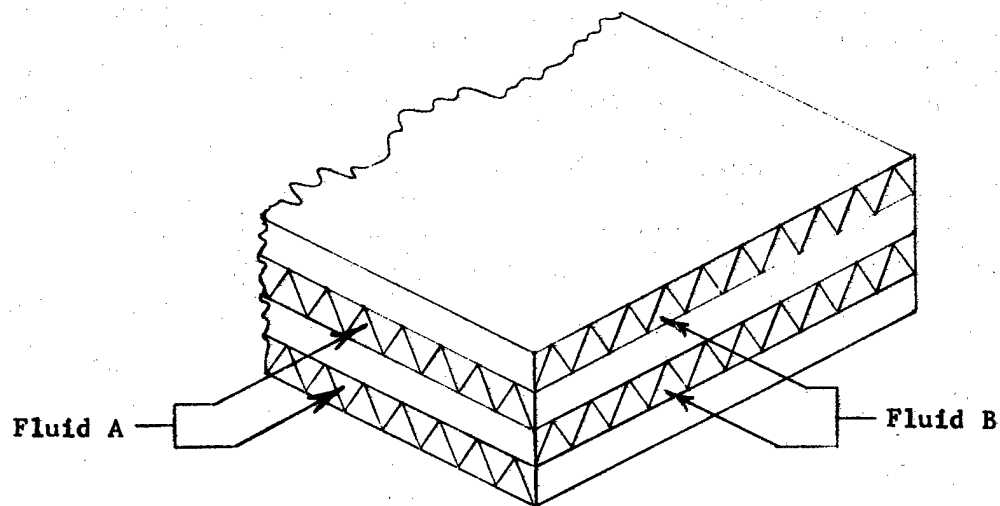
a. Conventional Plate/Folded-Fin Configuration
