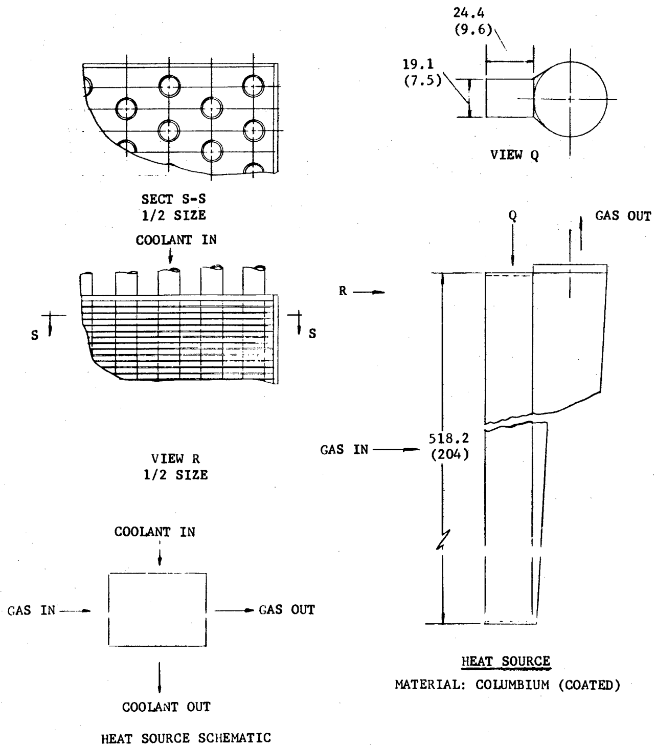
Figure 85. Heat Source
