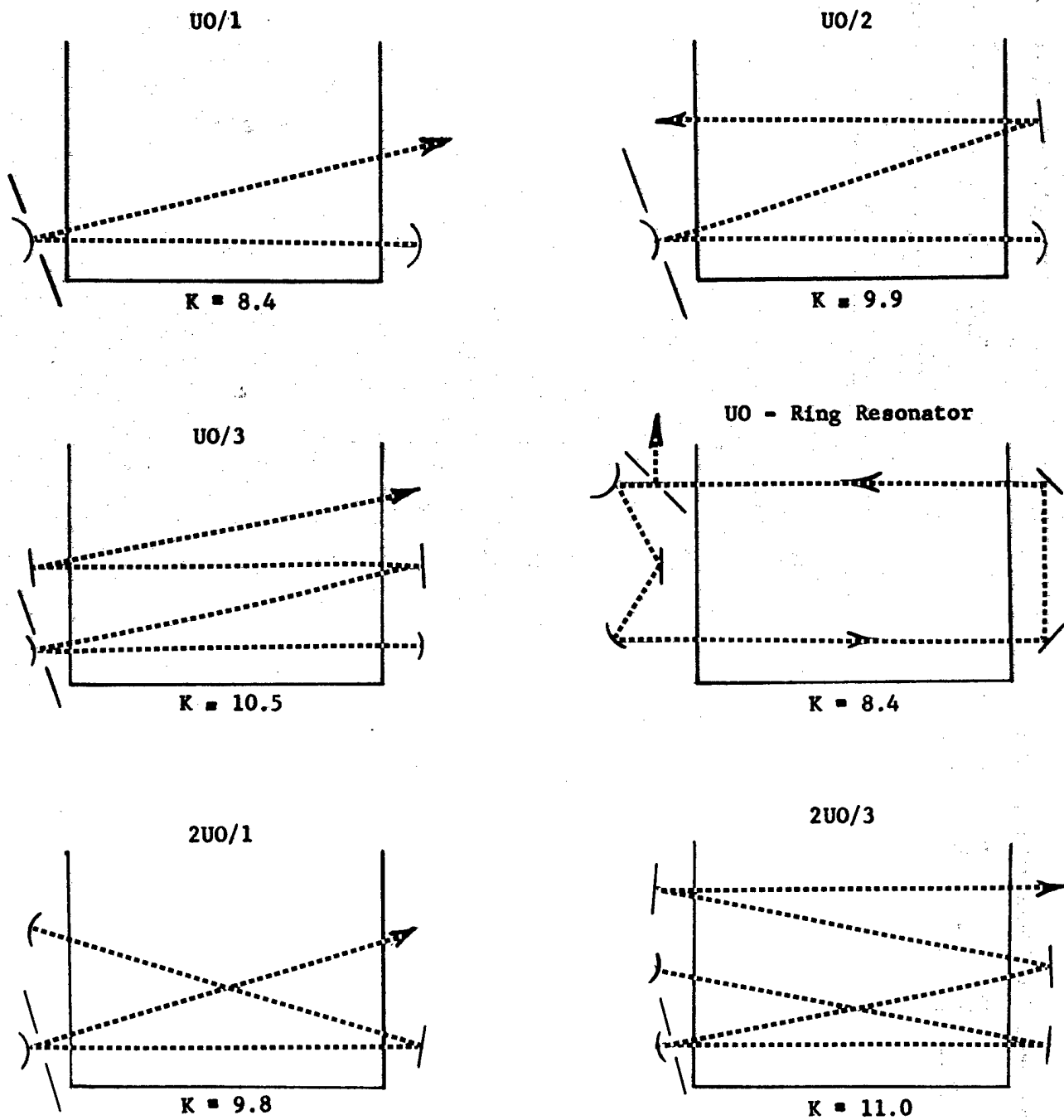
Figure 5. Optical Configuration Schematics
