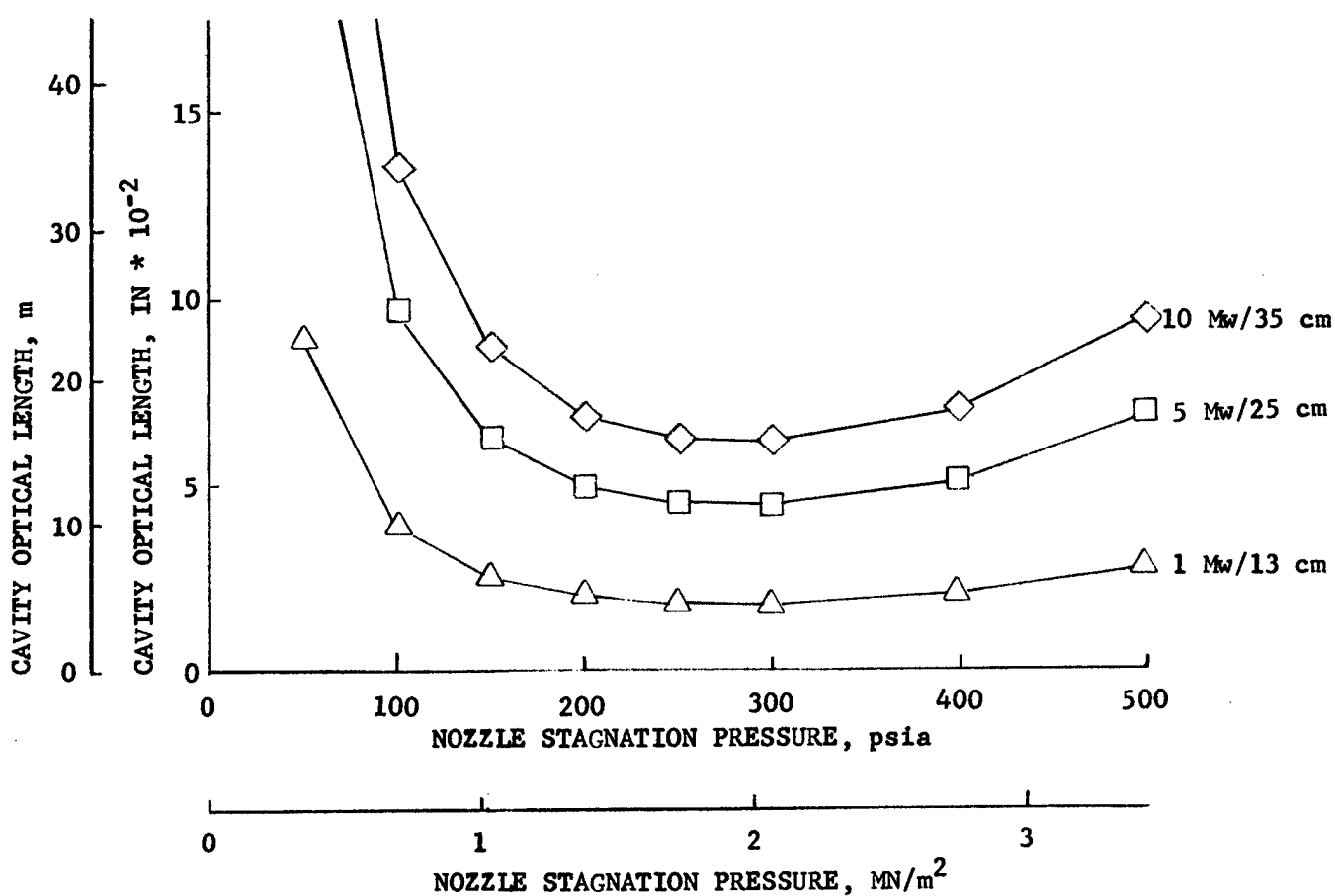
Figure 46. Effect of Laser Power Level and Nozzle Stagnation Pressure on Total System Weight and Cavity Optical Length
