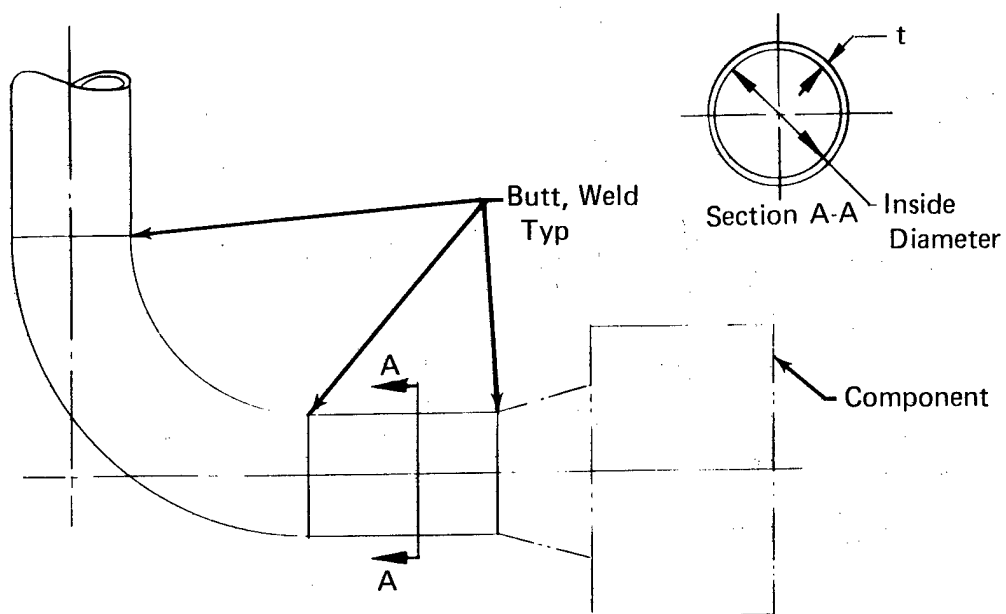
Figure 87. Type A Duct
