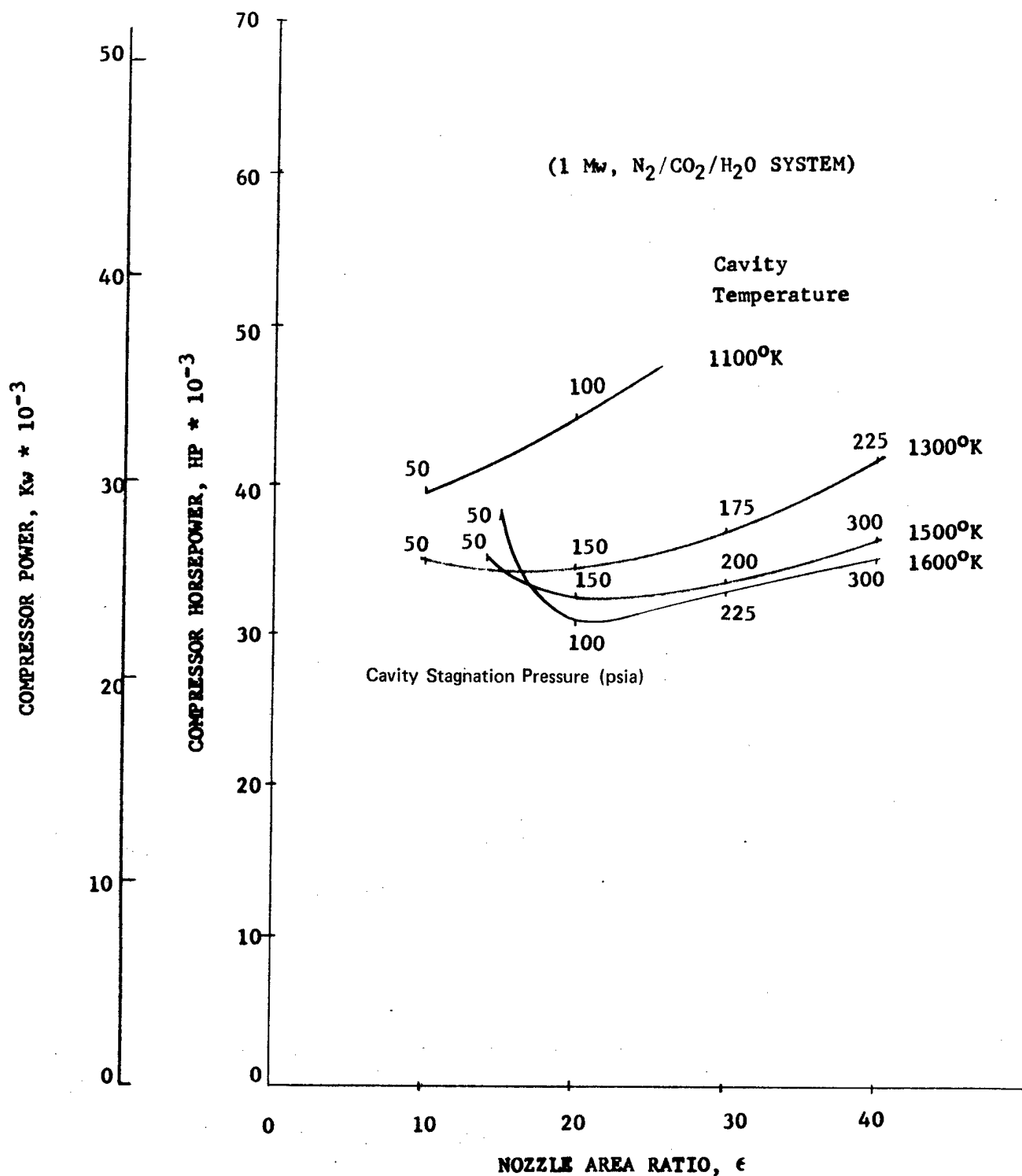
Figure 31. Effect of Nozzle Area Ratio and Cavity Stagnation Temperature on Compressor Power Requirement
