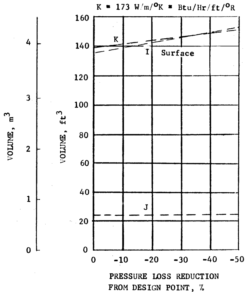
Figure 82. Effect of Pressure Loss on 1-Mw Airborne System Heat Sink Heat Exchanger Volume
