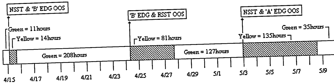
Figure 6.2 DID Levels for MP-3 1995 Refueling Outage
