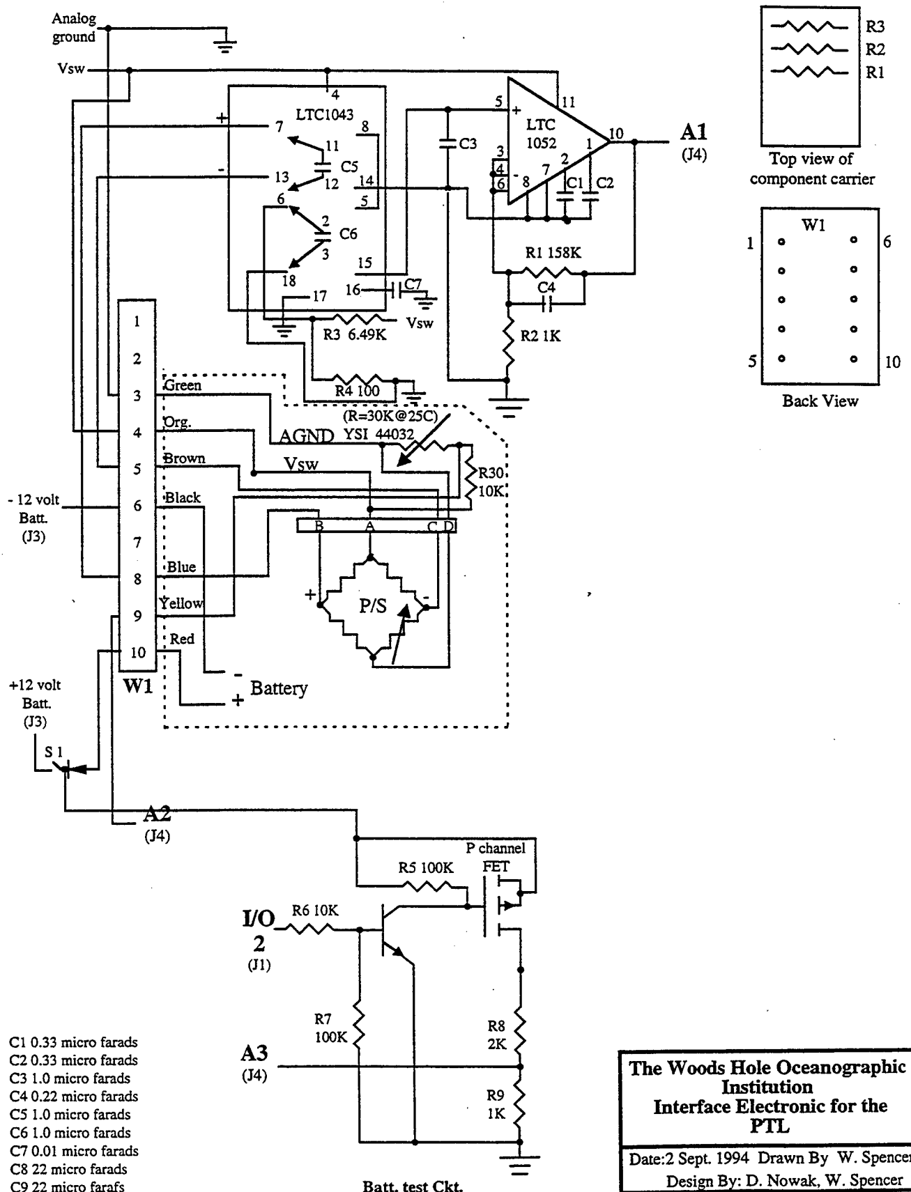
Figure 2.3: Interface electronics for the PTL.
