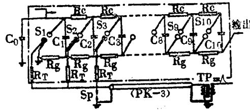
Figure 1. Circuitry of the 1 MV Marx Generator
