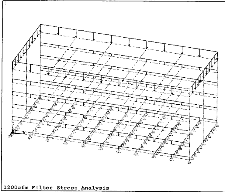
Figure 6: Load Case 3
