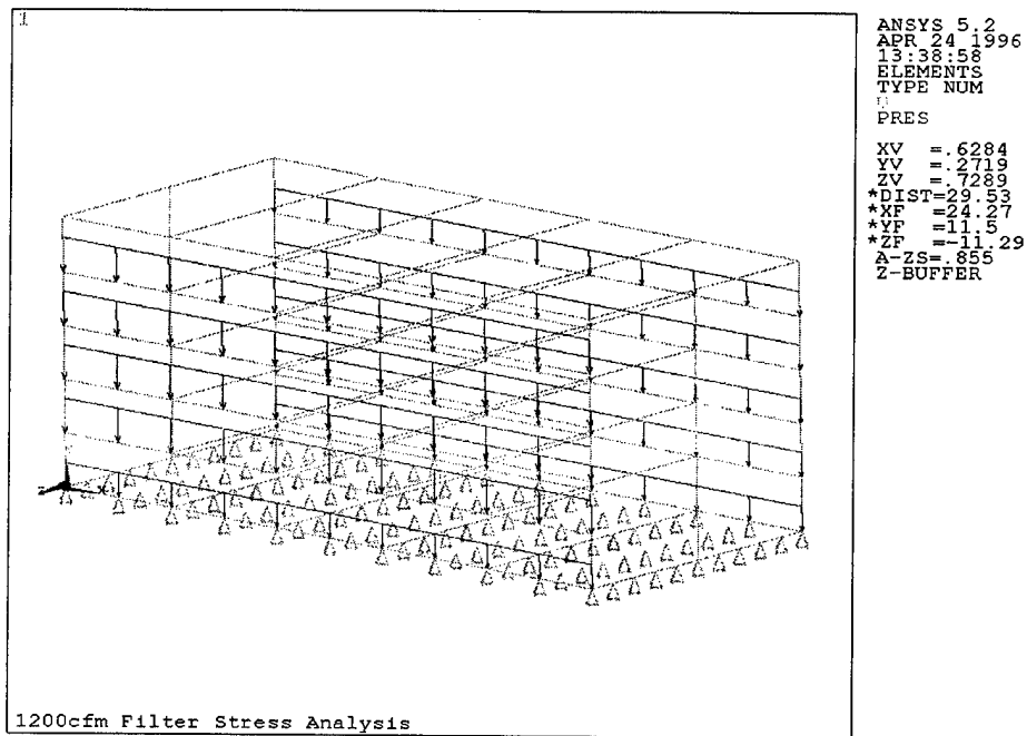
Figure 4: Load Case 1
