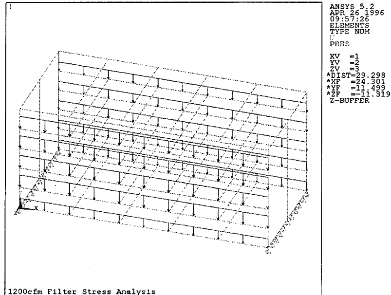
Figure 5: Load Case 2
