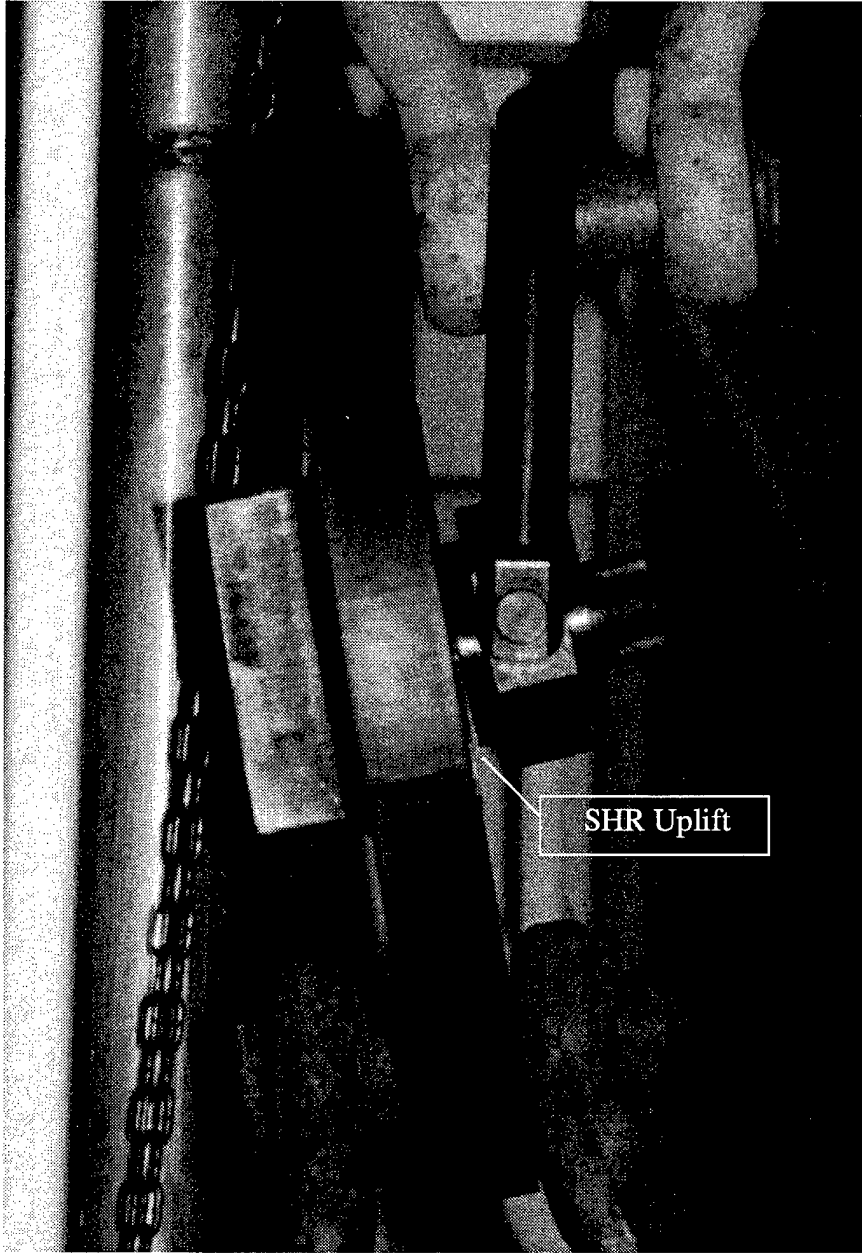
Figure 9. Base of Swivel Hoist Ring Tilts at 90,000 Pounds (NFESC # 9700128a)
