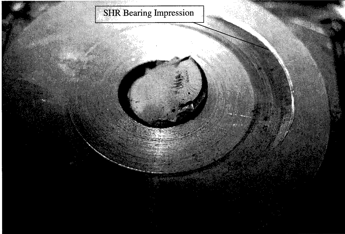
Figure 16. Washer Plate with Broken Bolt (NFESC # 9700173)
